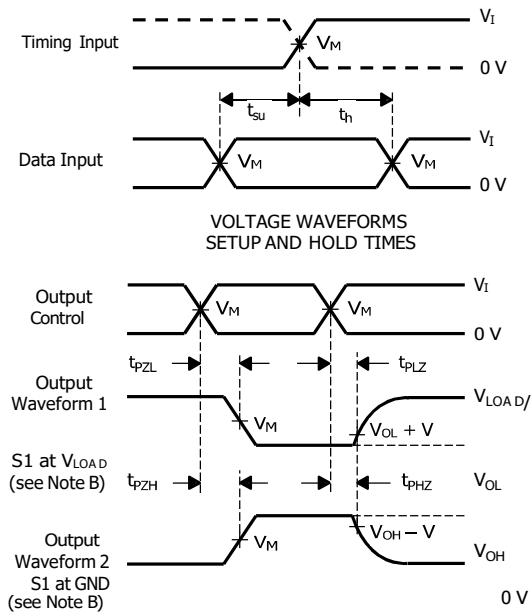
VOLTAGE WAVEFORMS ENABLE AND DISABLE TIMES LOW-AND HIGH-LEVEL ENABLING
