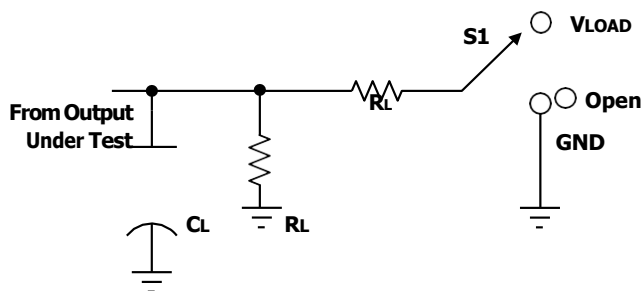
Figure 1. Load Circuit and Voltage Waveforms
