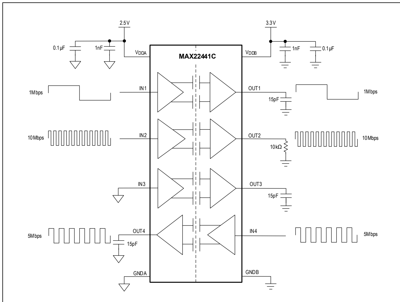
Figure 13. Example Circuit for Supply Current Calculation
