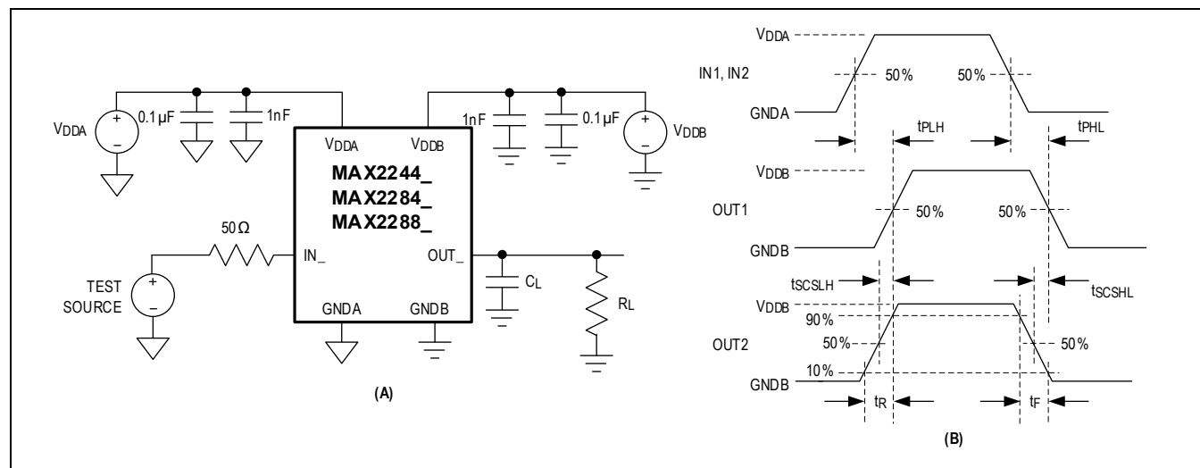
Figure 1. Test Circuit (A) and Timing Diagrams (B)
