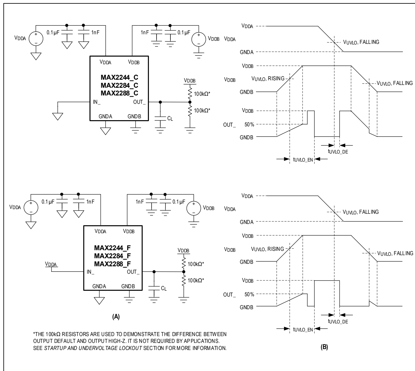
Figure 3. UVLO to Output Timing Diagrams ( t_{UVLO\_EN} , t_{UVLO\_DE} )
