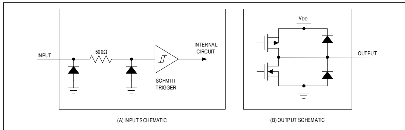
Figure 10. Device I/O Schematics
