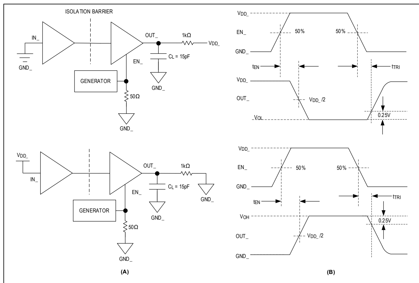
Figure 2. Enable to Output Timing Diagrams ( t_{EN} , t_{TRI} )
