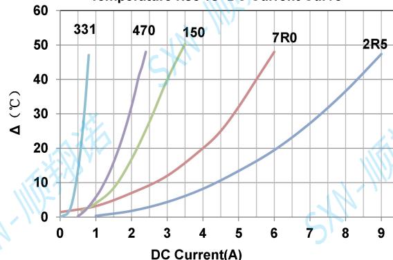
Temperature rise vs DC Current Curve
