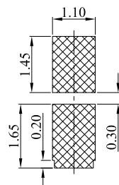
METAL MASK T=0.08 TOLERANCE:±0.05MM (FOR REFERENCE ONLY)
