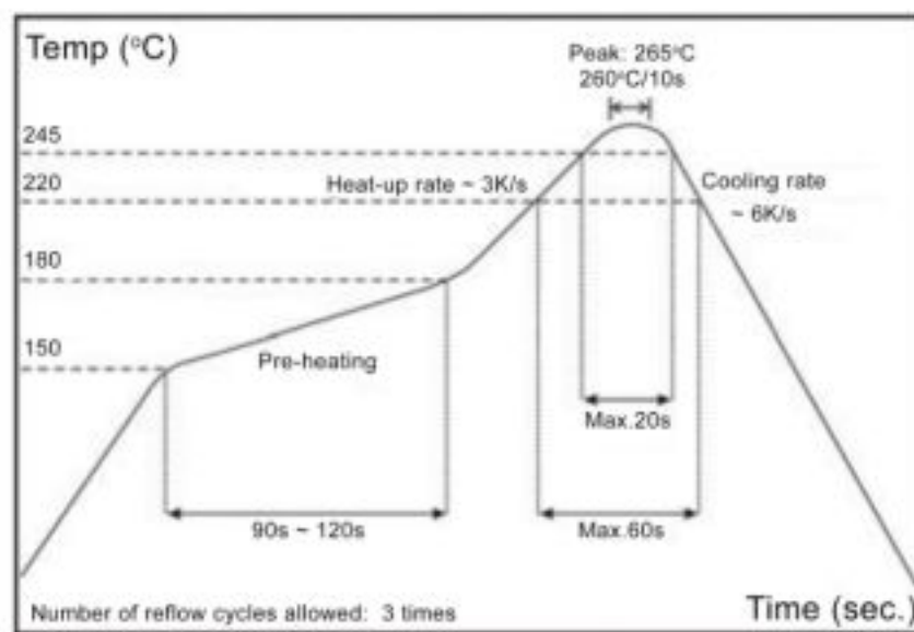
IR Reflow Soldering
