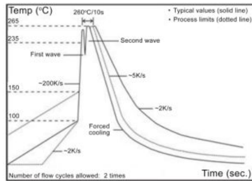
Wave Soldering (Flow Soldering)
