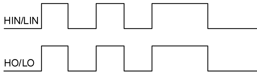
Figure 7-1 DOS2186 Input and output timing waveform
