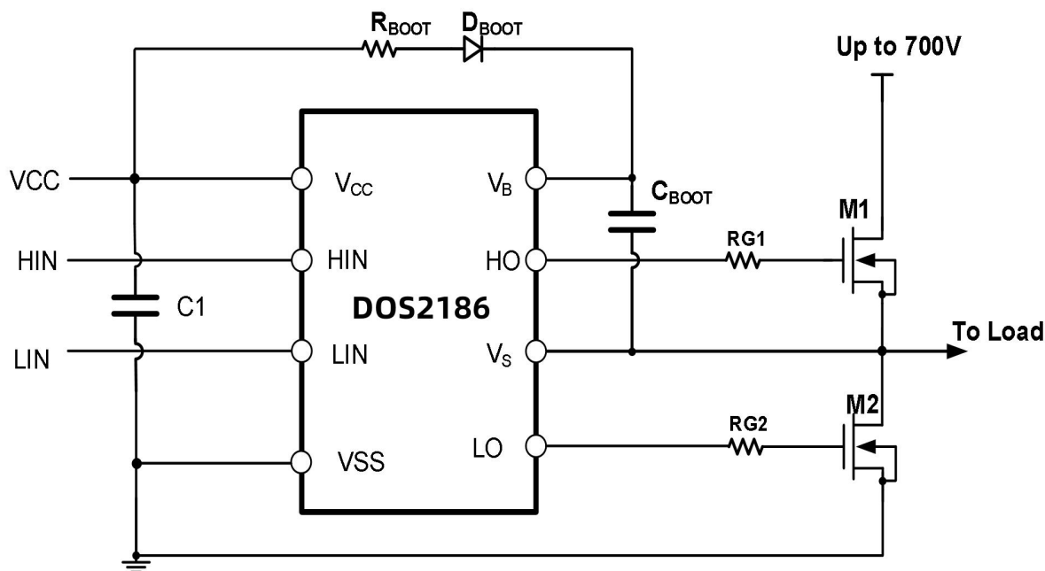
Figure 8-2 Typical application circuit of DOS2186
