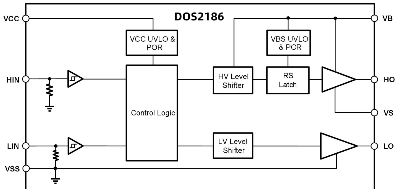
Figure 8 -1 Function Block Diagram of DOS2186
