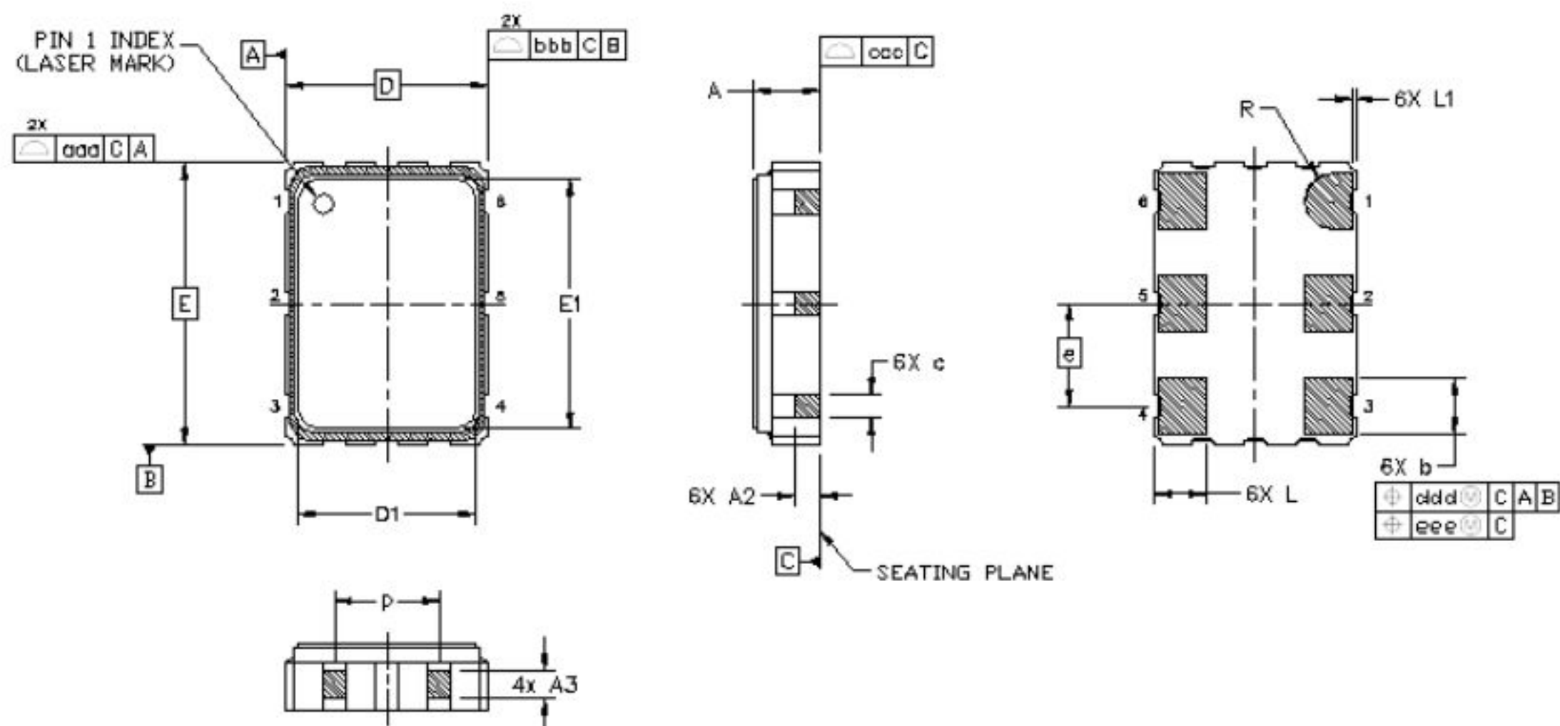
Figure 5.1. Si540 (5×7 mm) Outline Diagram
