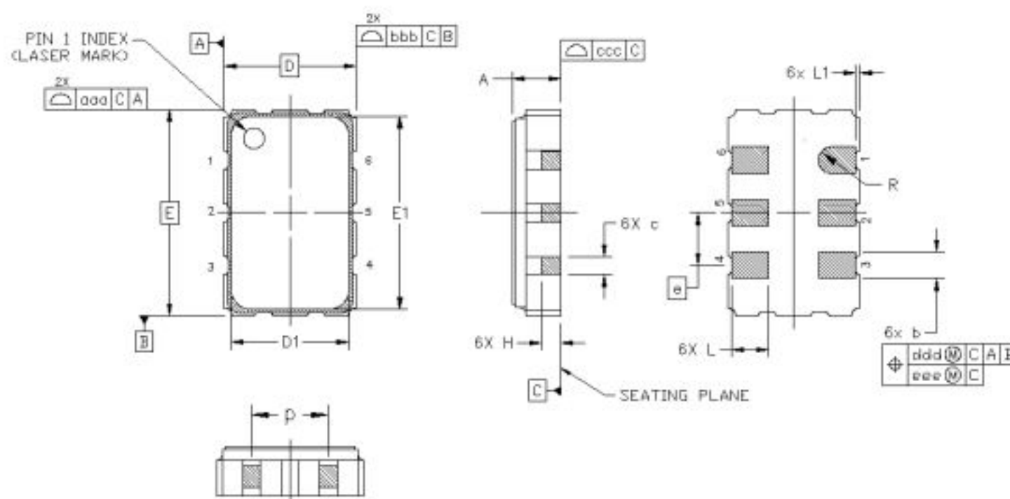
Figure 5.2. Si540 (3.2×5 mm) Outline Diagram
