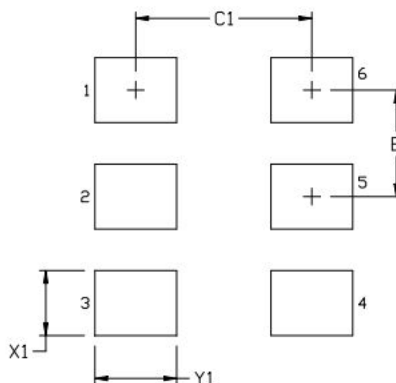
Figure 6.1. Si540 (5×7 mm) PCB Land Pattern
