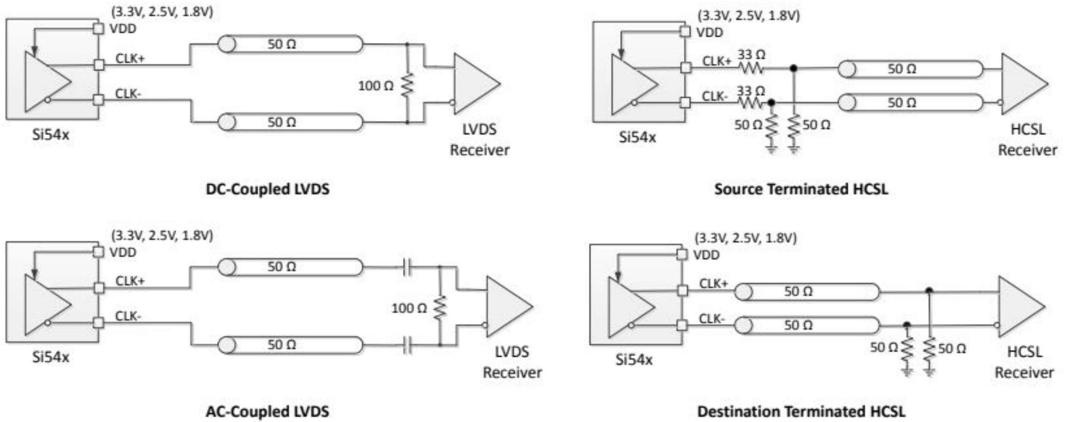
Figure 4.2. LVDS and HCSL Output Terminations
