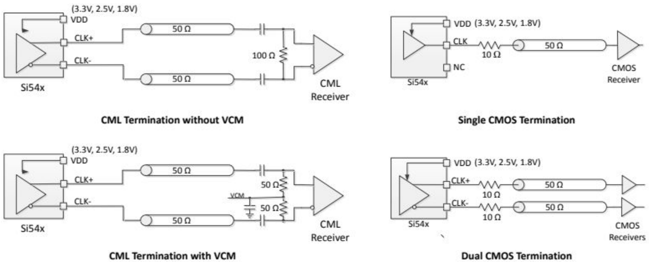
Figure 4.3. CML and CMOS Output Terminations
