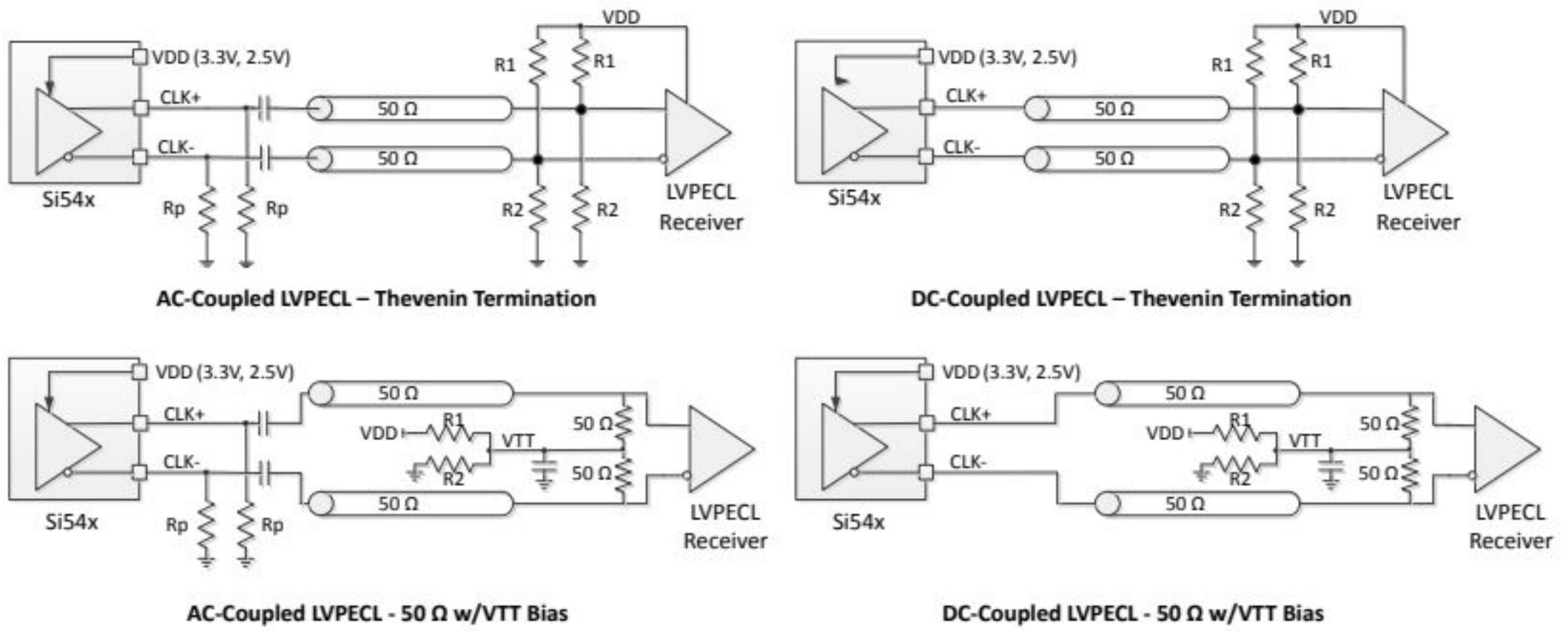
Figure 4.1. LVPECL Output Terminations
