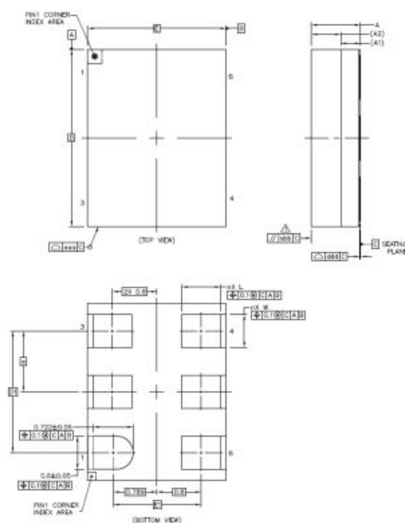
Figure 5.3. Si540 (2.5x3.2 mm) Outline Diagram
