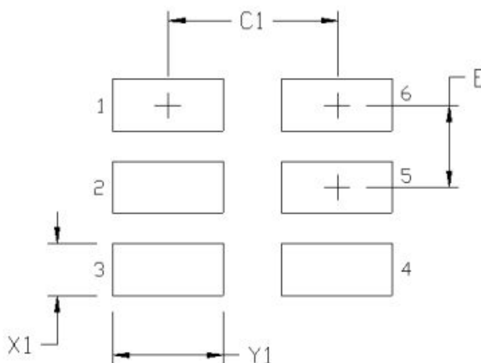
Figure 6.2. Si540 (3.2×5 mm) PCB Land Pattern
