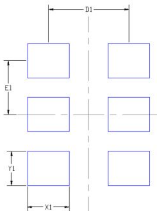
Figure 6.3. Si540 (2.5×3.2 mm) PCB Land Pattern
