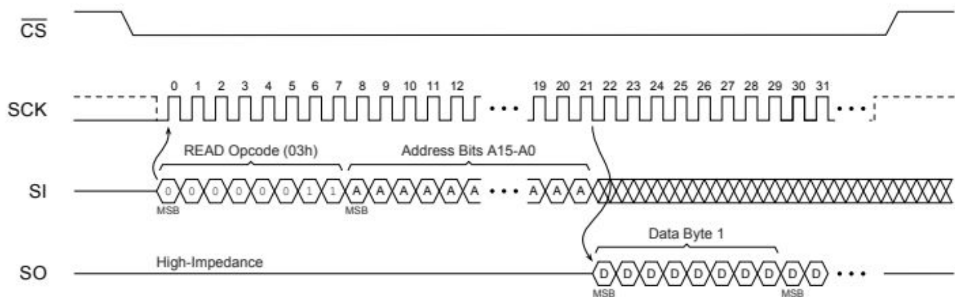
Figure 7-1. Read Waveform
