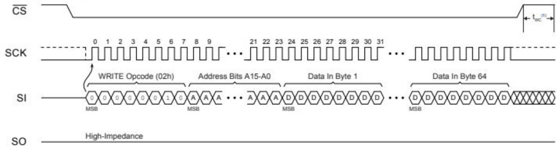
Figure 8-2. Page Write
