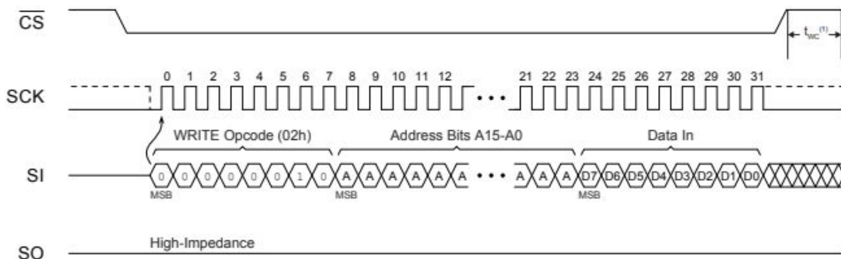
Figure 8-1. Byte Write
