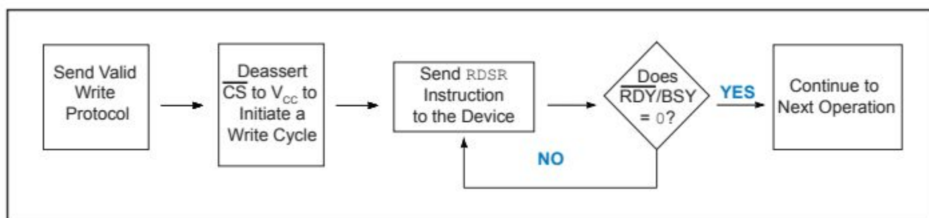
Figure 8-3. Polling Flowchart
