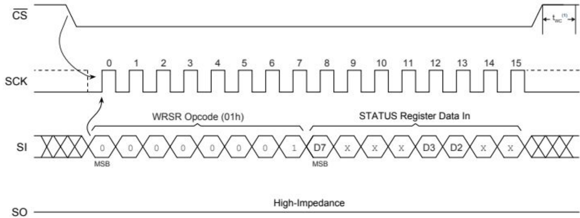
Figure 6-4. WRSR Waveform
