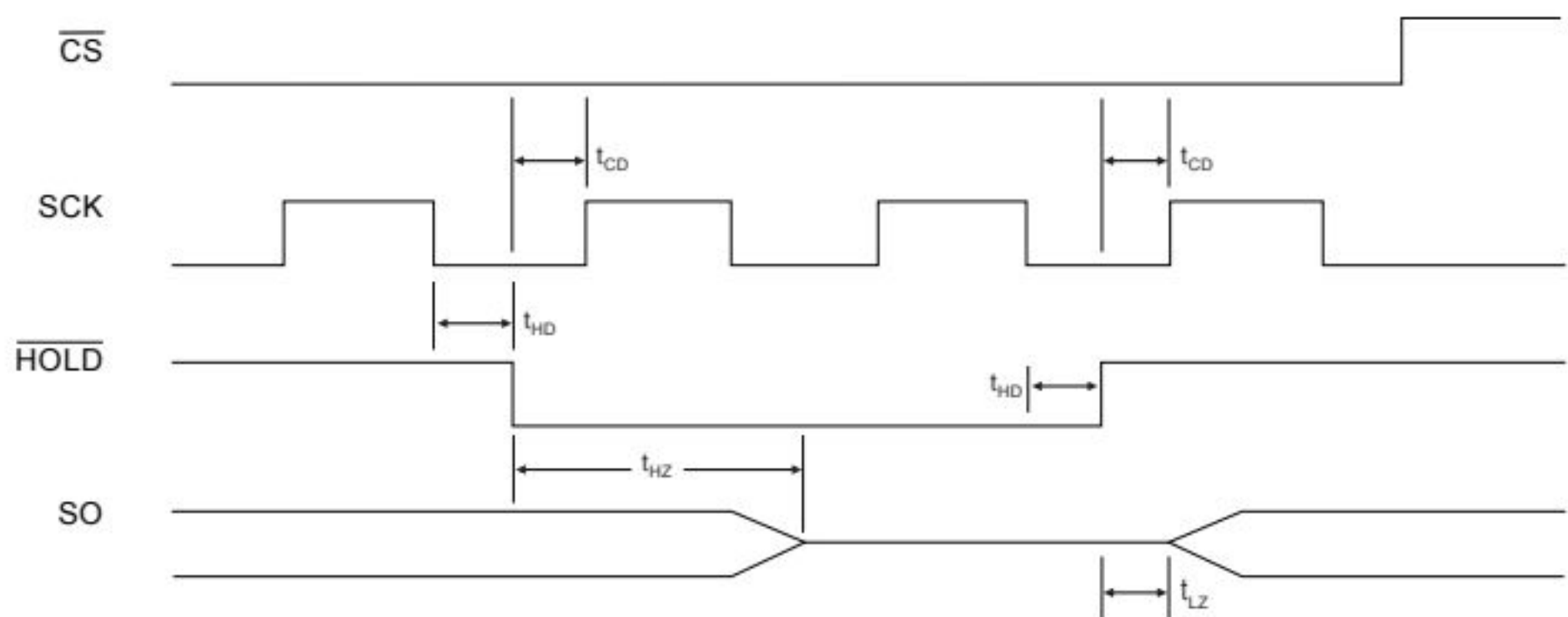
Figure 5-3. Hold Timing
