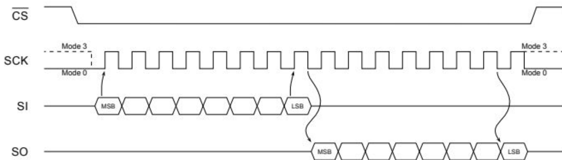
Figure 5-1. SPI Mode 0 and Mode 3
