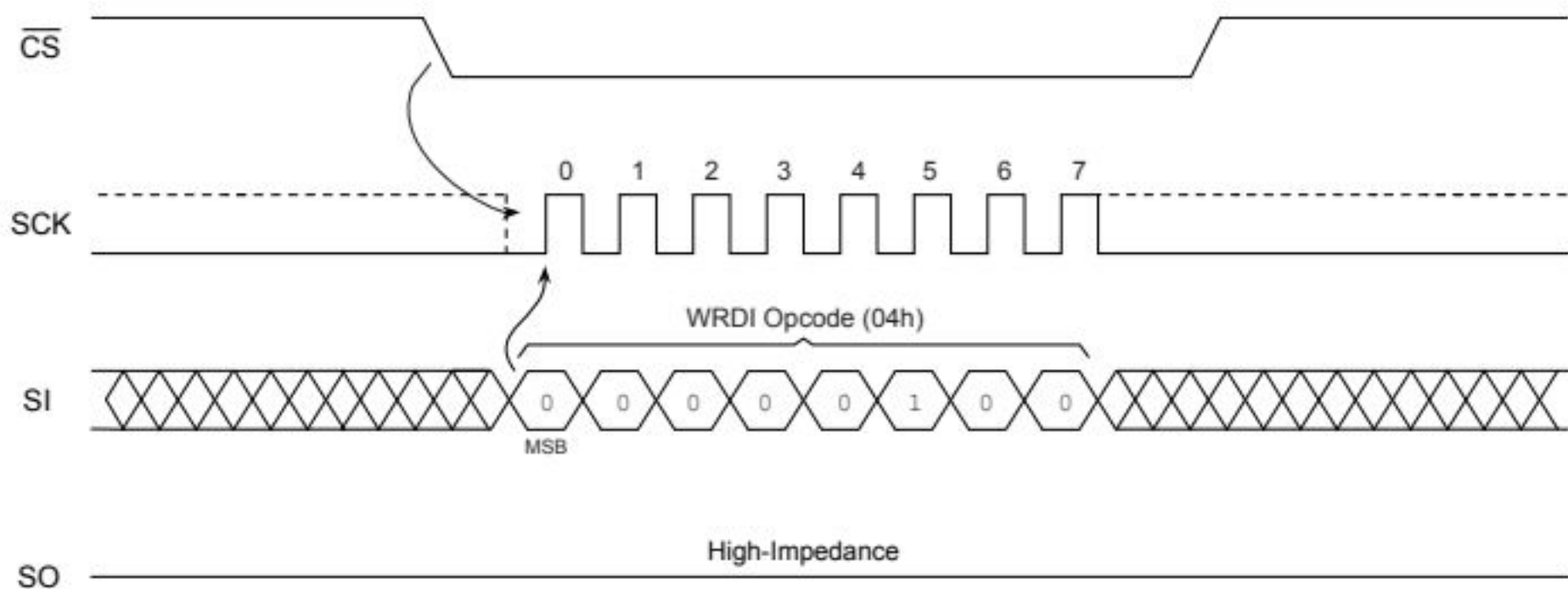
Figure 6-3. WRDI Timing
