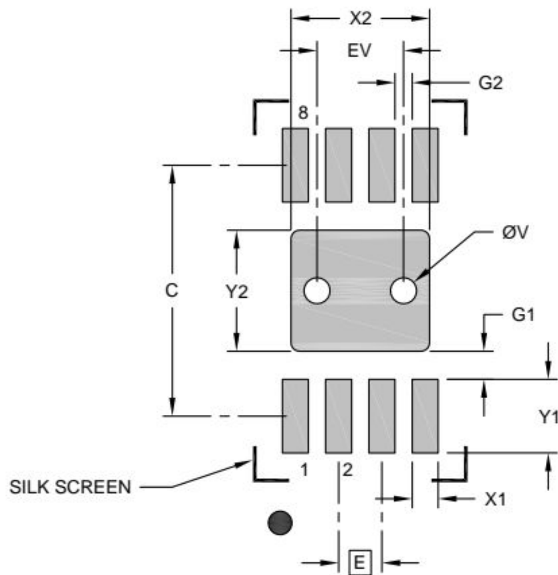
RECOMMENDED LAND PATTERN
