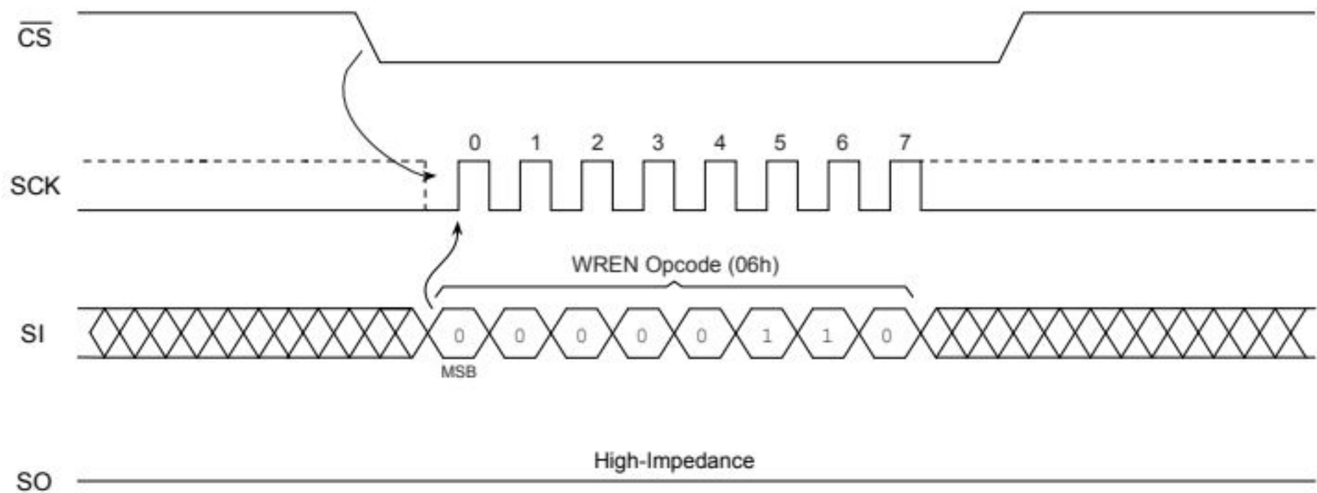
Figure 6-2. WREN Timing
