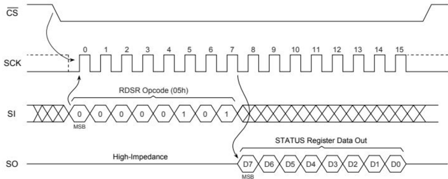
Figure 6-1. RDSR Waveform
