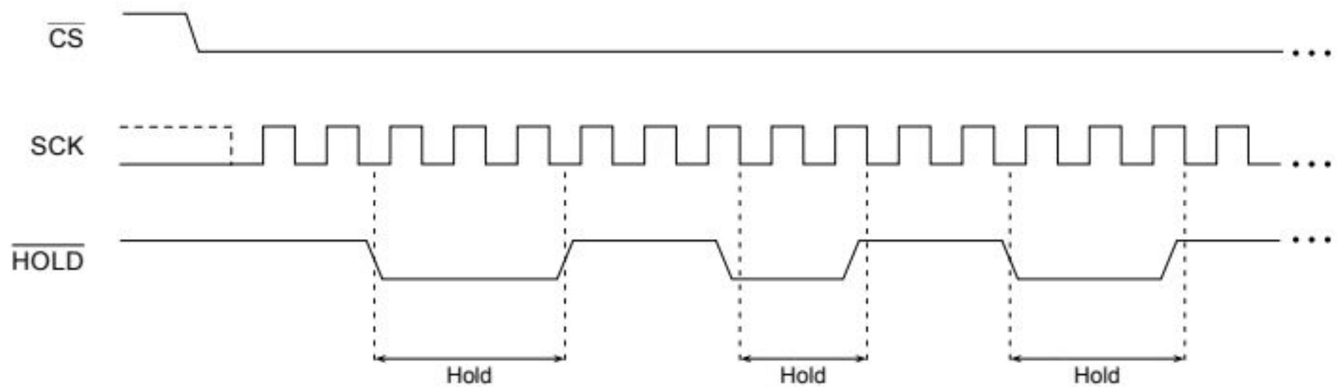
Figure 5-3. Hold Timing
