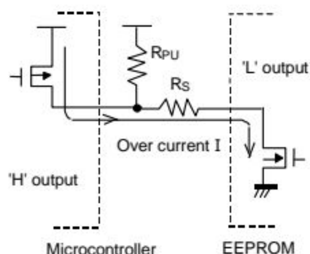
Figure 54. I/O circuit diagram
