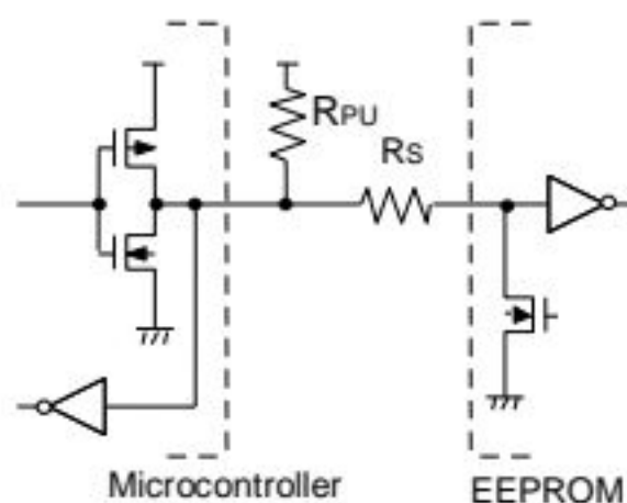
Figure 51. I/O circuit diagram
