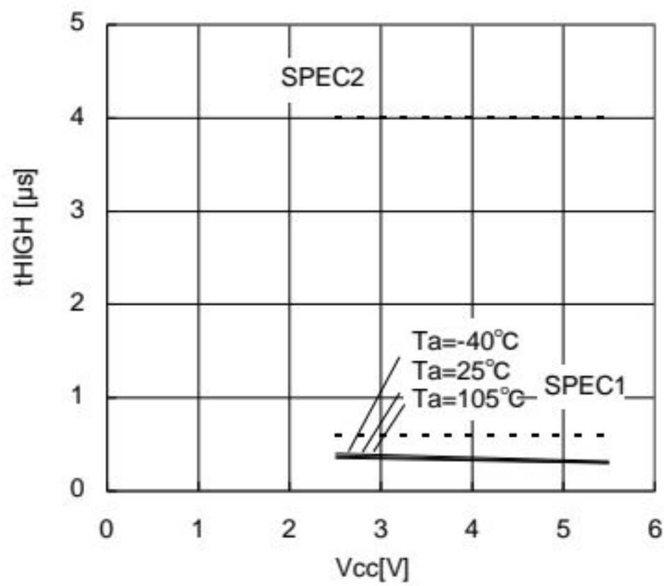
Figure 15. Data clock "H" time t_{HIGH}
