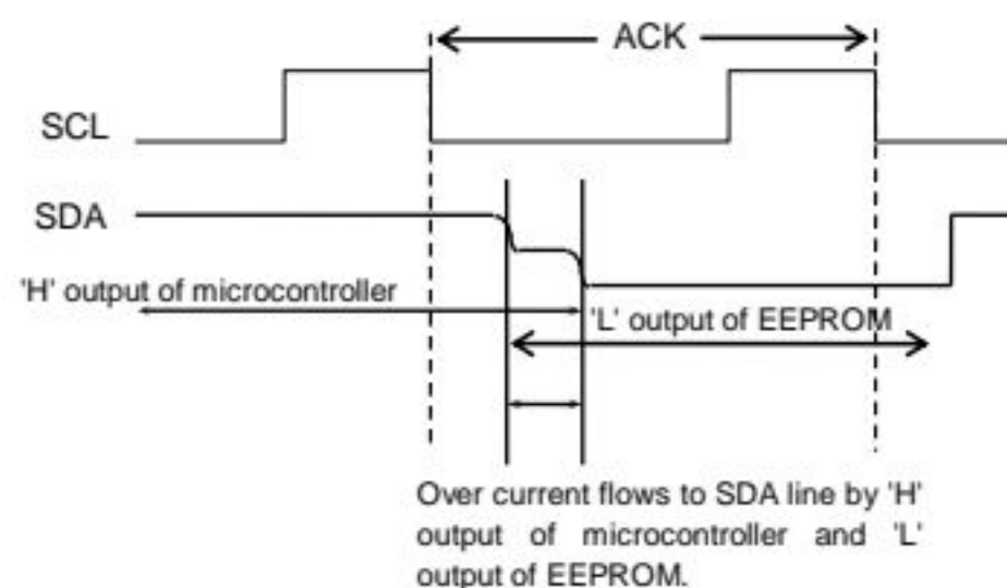
Figure 52. Input / output collision timing
