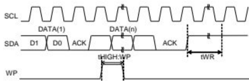
Figure 1-(c) Write cycle timing
