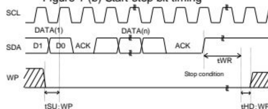
Figure 1-(d) WP timing at write execution
