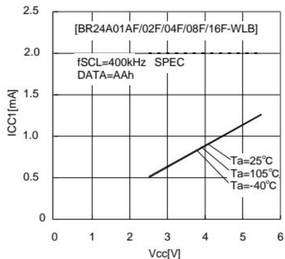
Figure 7. Current consumption at WRITE operation ICC1 (fSCL=400kHz)
