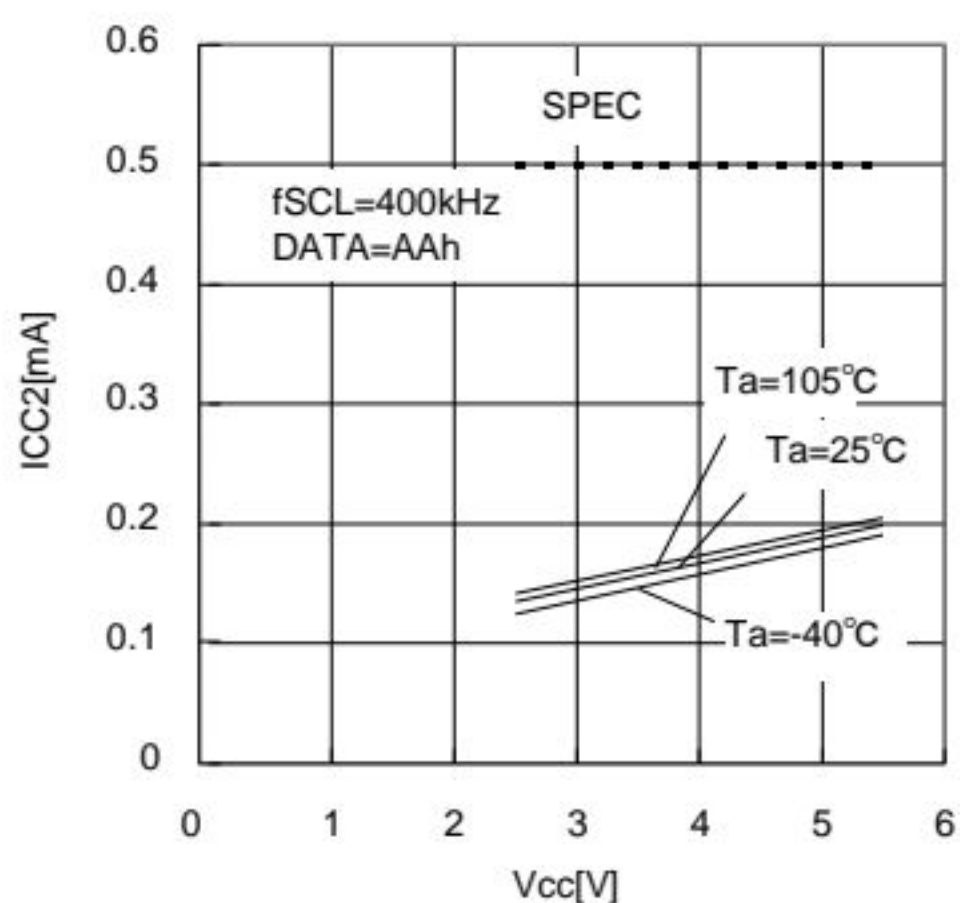
Figure 9. Current consumption at READ operation ICC2 (fSCL=400kHz)
