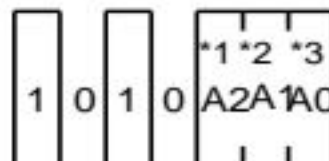
Figure 40. Difference of each type of slave address
