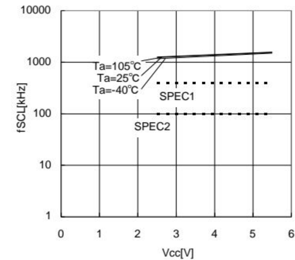
Figure 14. SCL frequency f_{SCL}
