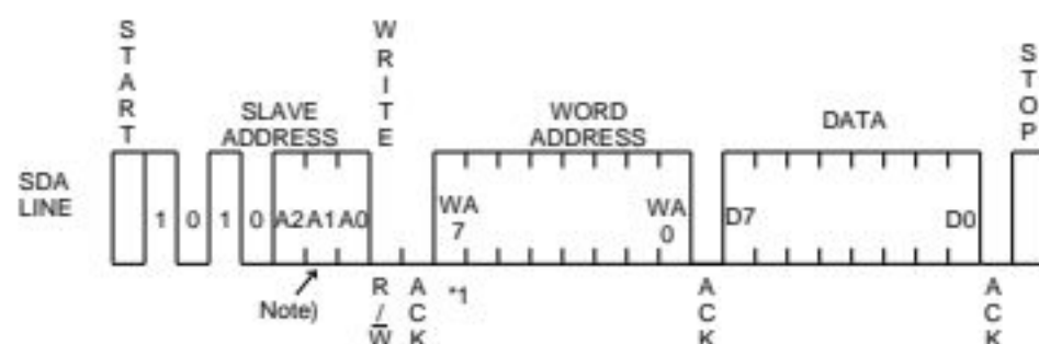
Figure 34. Byte write cycle (BR24A01AF/02F/04F/08F/16F-WLB)
