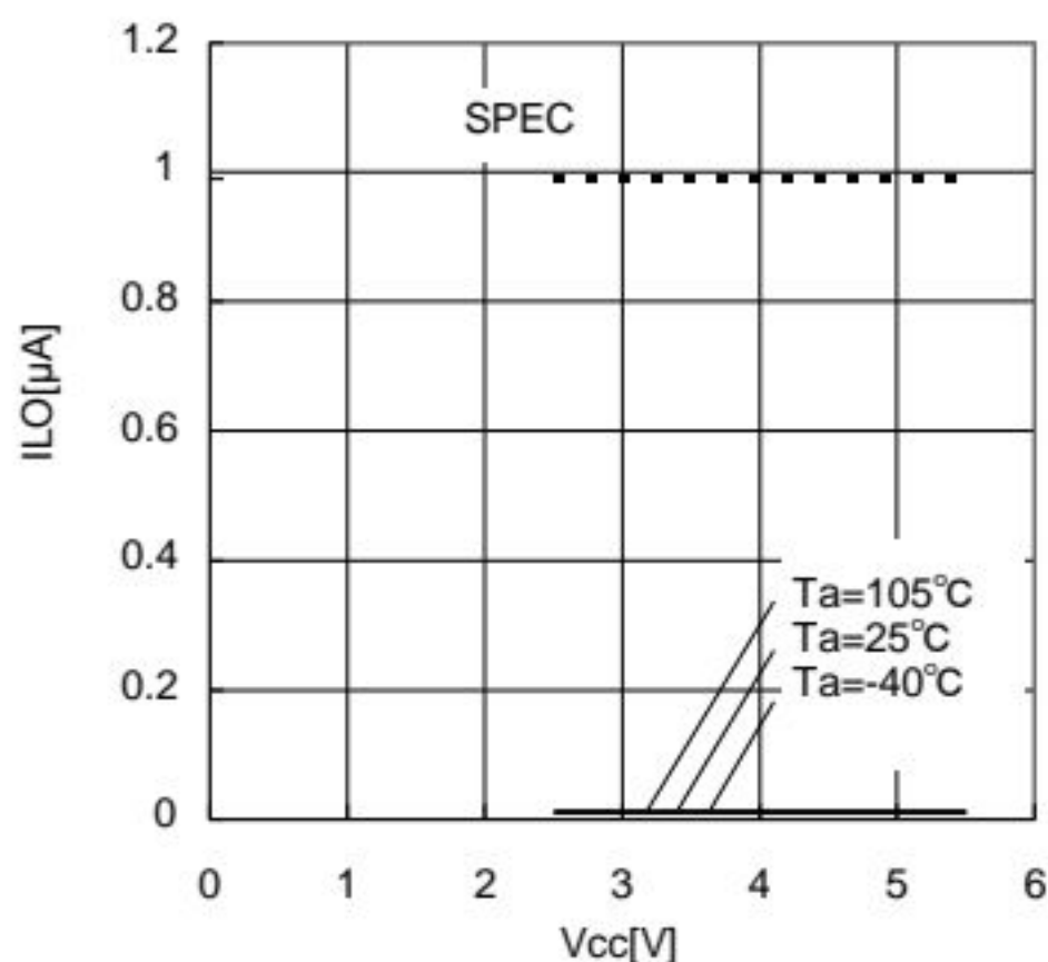
Figure 6. Output leak current ILO(SDA)
