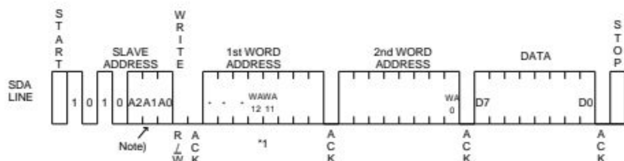
Figure 35. Byte write cycle (BR24A32F/64F-WLB)
