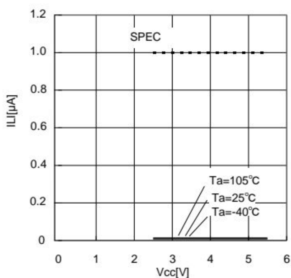
Figure 5. Input leak current I_{LI} (SCL, WP)
