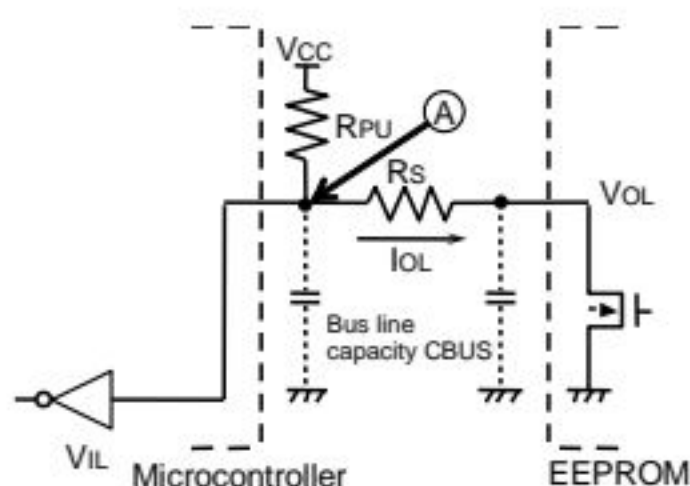
Figure 53. I/O circuit diagram
