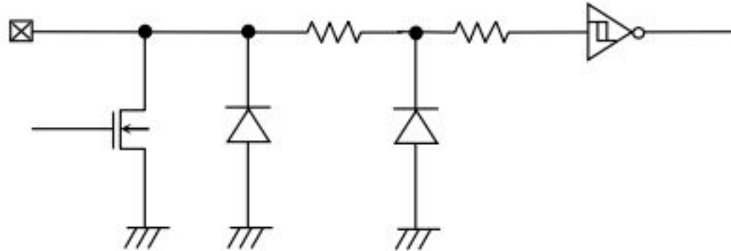
Figure 56. Input / output pin circuit diagram
