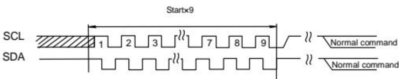
Figure 46-(c) STARTx9+ command input
