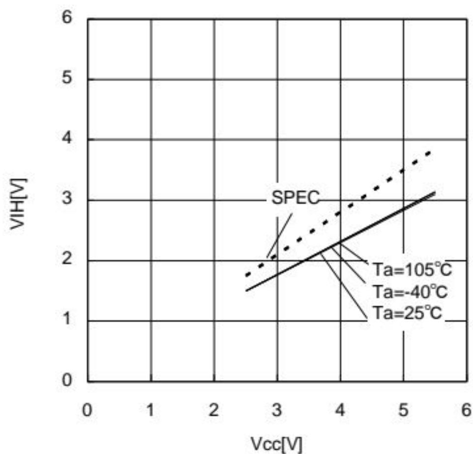
Figure 2. H input voltage V_{IH1,2} (SCL, SDA, WP)
