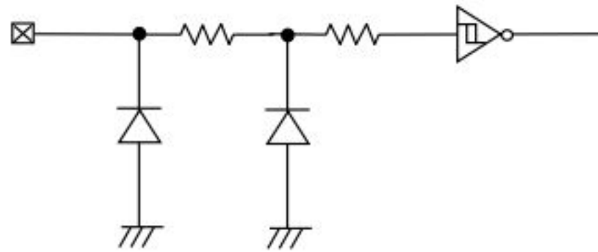
Figure 55. Input pin circuit diagram
