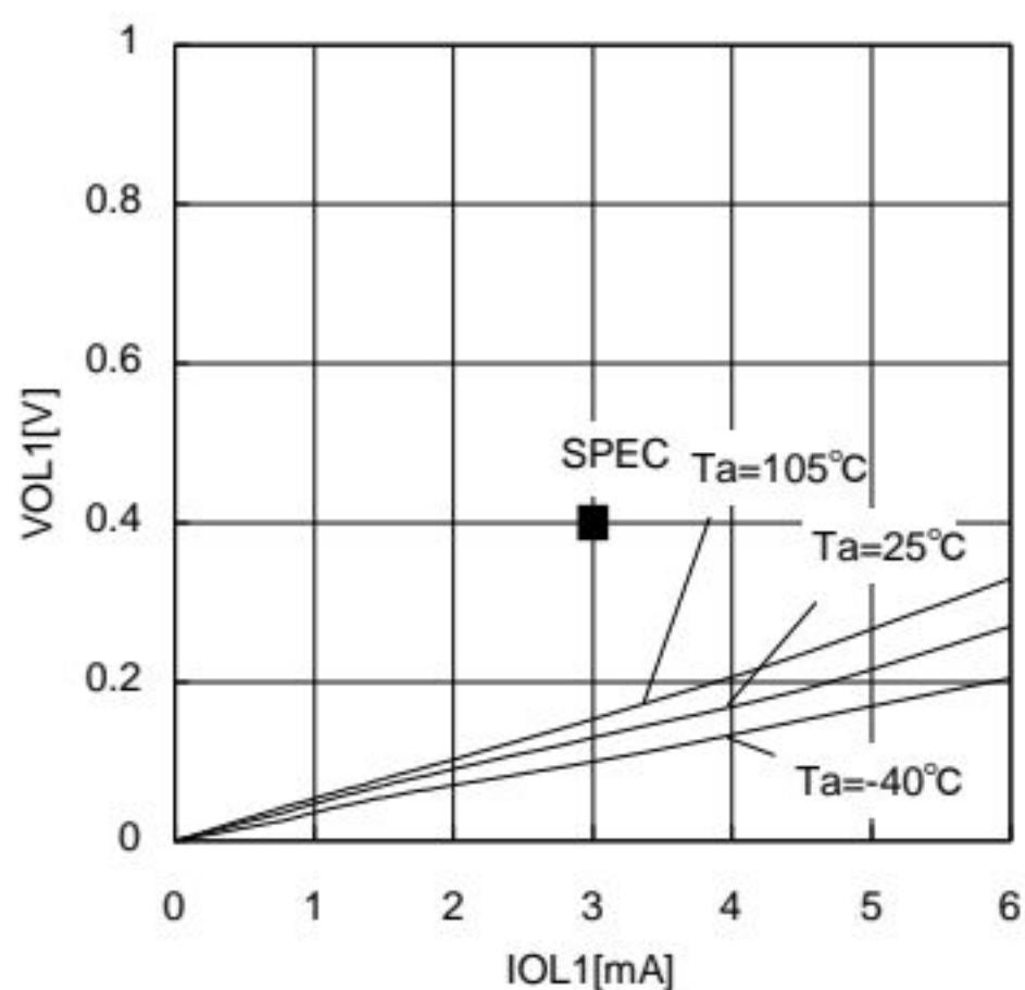
Figure 4. L output voltage V_{OL1} - I_{OL1} ( V_{CC} = 2.5\text{V} )
