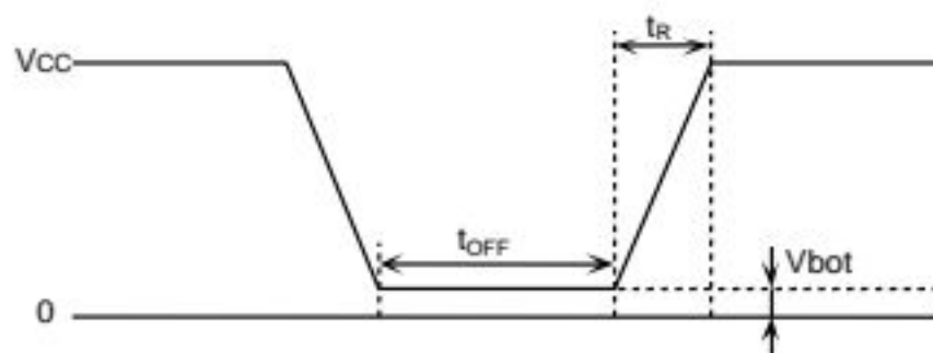
Figure 58. Rise waveform diagram
