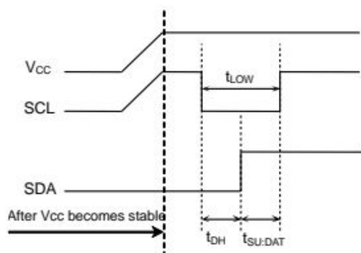
Figure 59. When SCL= 'H' and SDA= 'L'
