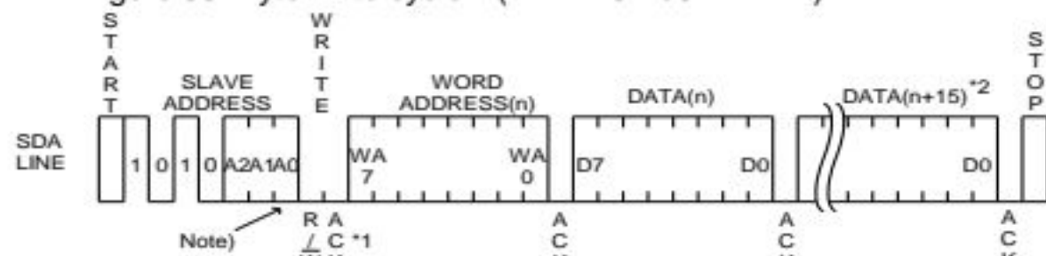
Figure 36. Page write cycle (BR24A01AF/02F/04F/08F/16F-WLB)
