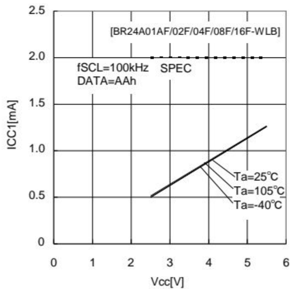
Figure 10. Current consumption at WRITE operation ICC1 ( f_{SCL}=100kHz )
