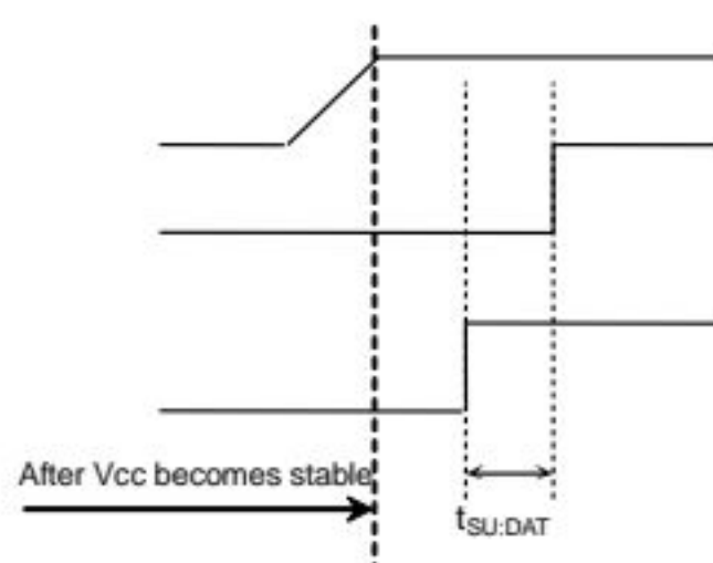
Figure 60. When SCL='L' and SDA='L'
