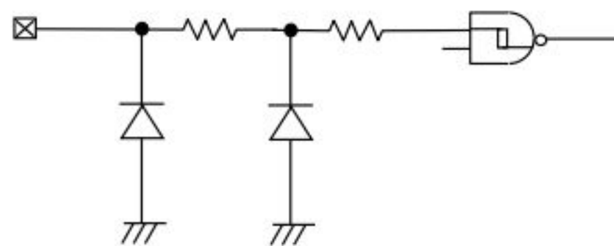
Figure 57. Input pin circuit diagram
