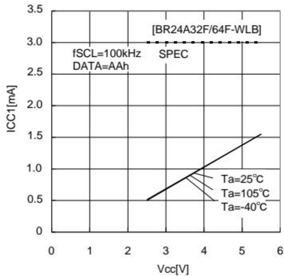
Figure 11. Current consumption at WRITE operation ICC1 ( f_{SCL}=100kHz )
