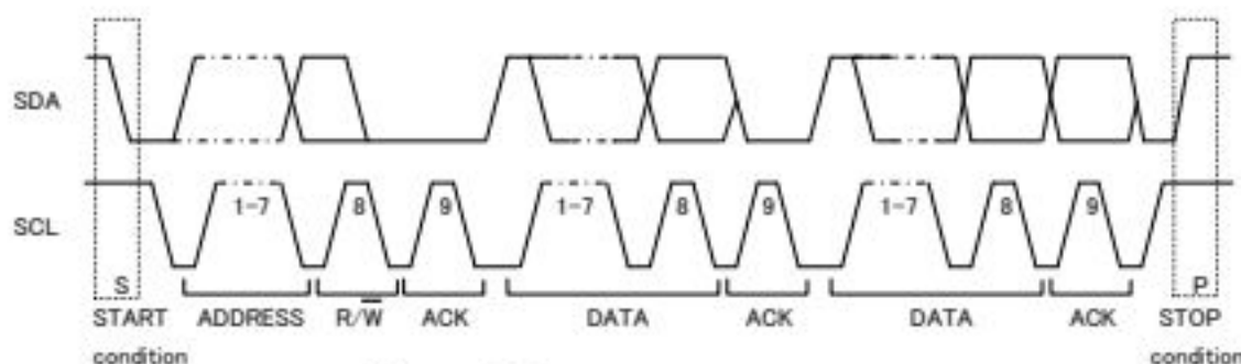
Figure 33. Data transfer timing
