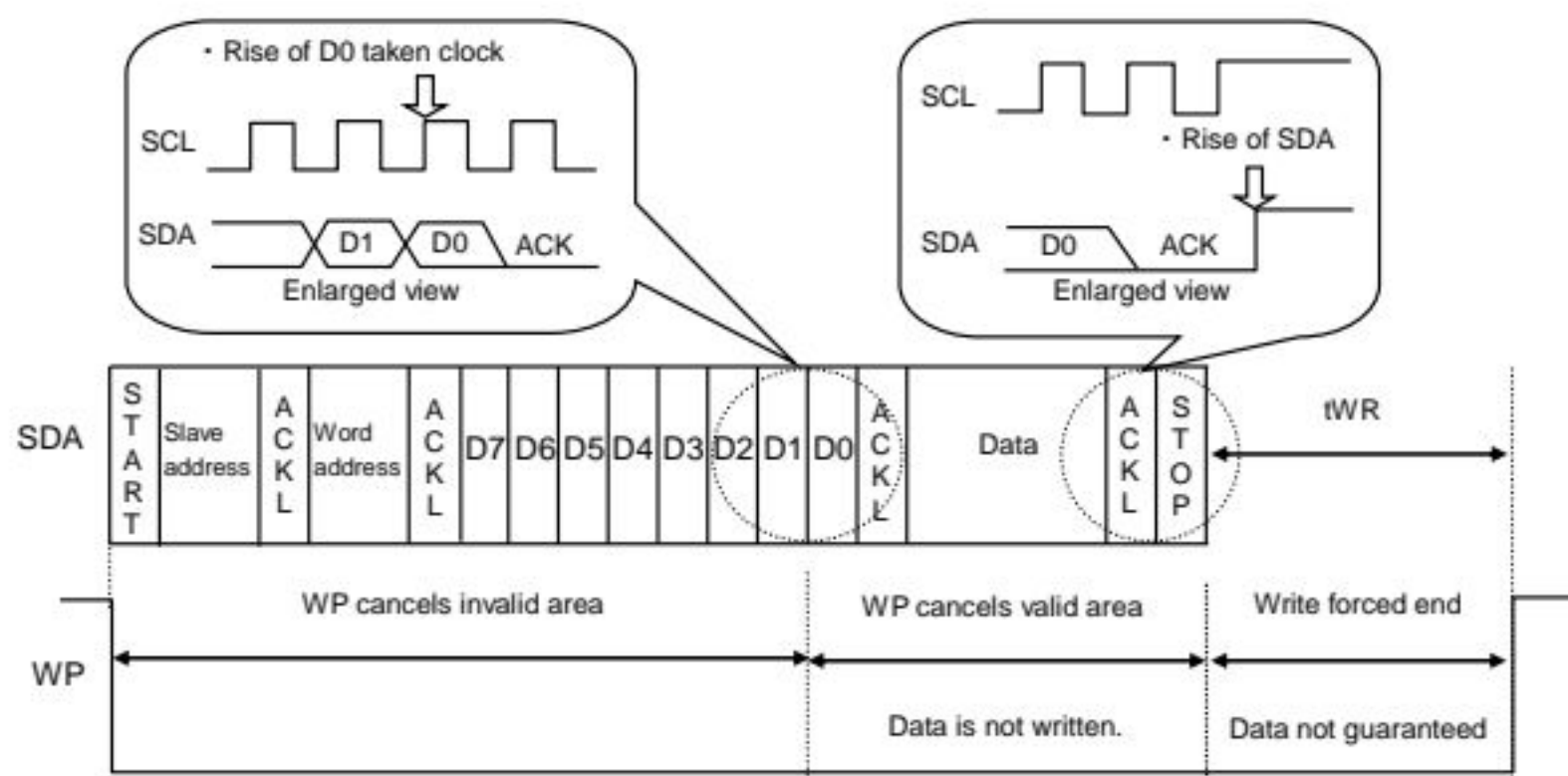
Figure 48. WP valid timing
