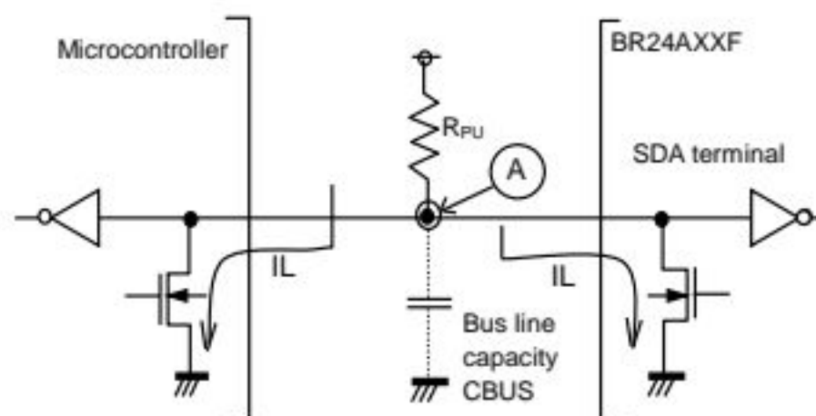
Figure 50. I/O circuit diagram
