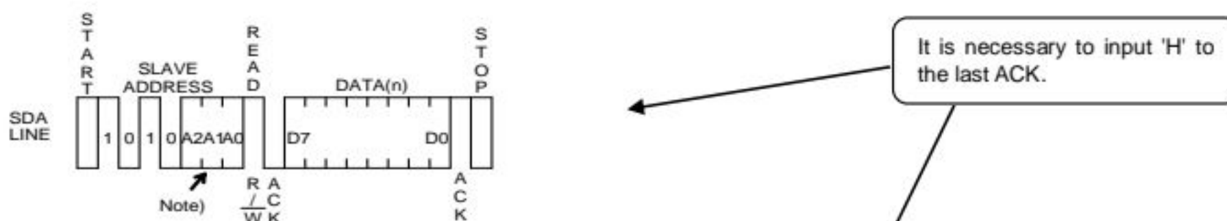
Figure 43. Current read cycle
