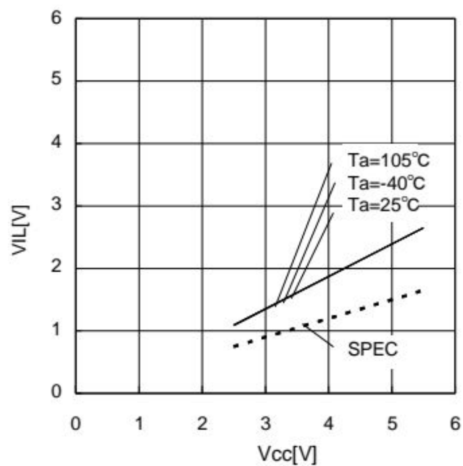
Figure 3. L input voltage V_{IL1,2} (SCL, SDA, WP)
