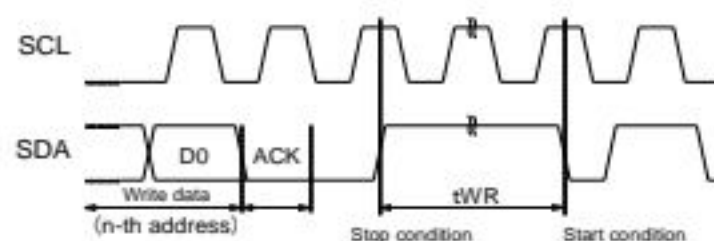
Figure 1-(c) Write cycle timing
