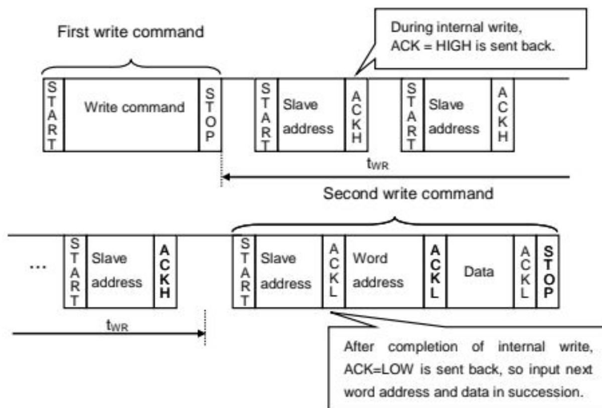
Figure 47. Case to continuously write by acknowledge polling
