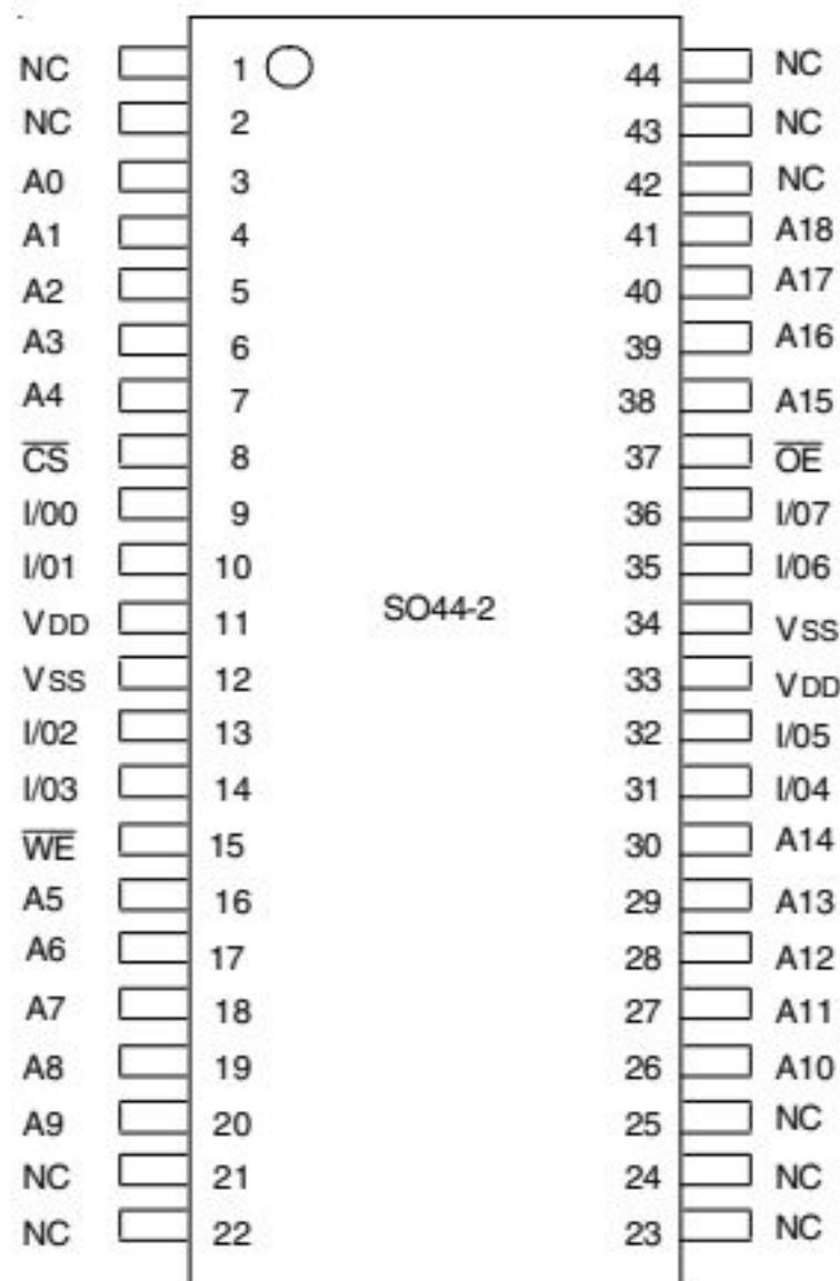
TSOP Top View
