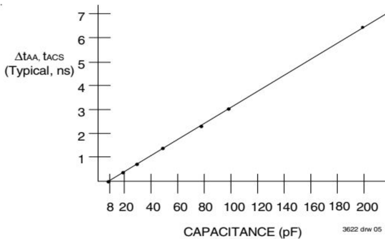
Figure 3. Output Capacitive Derating
