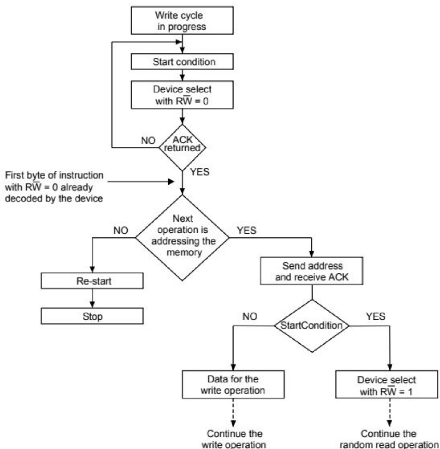
Figure 10. Write cycle polling flowchart using ACK
