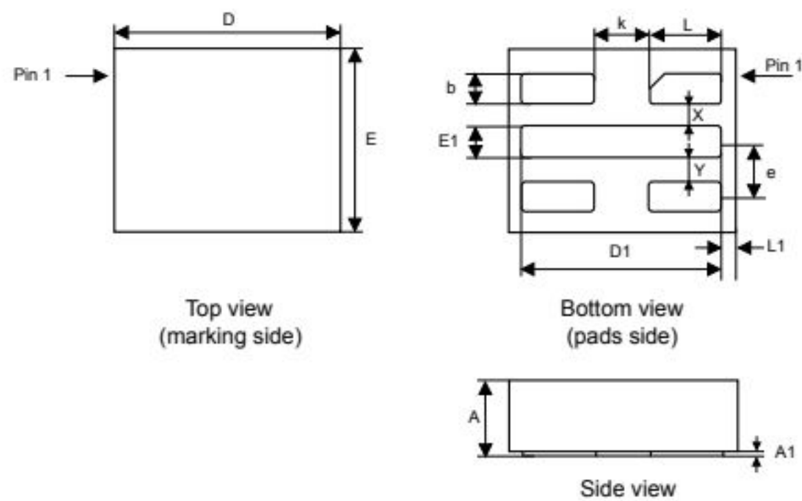
Figure 16. UFDFPN5 - Outline
