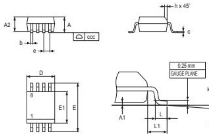
Figure 22. SO8N – Outline
