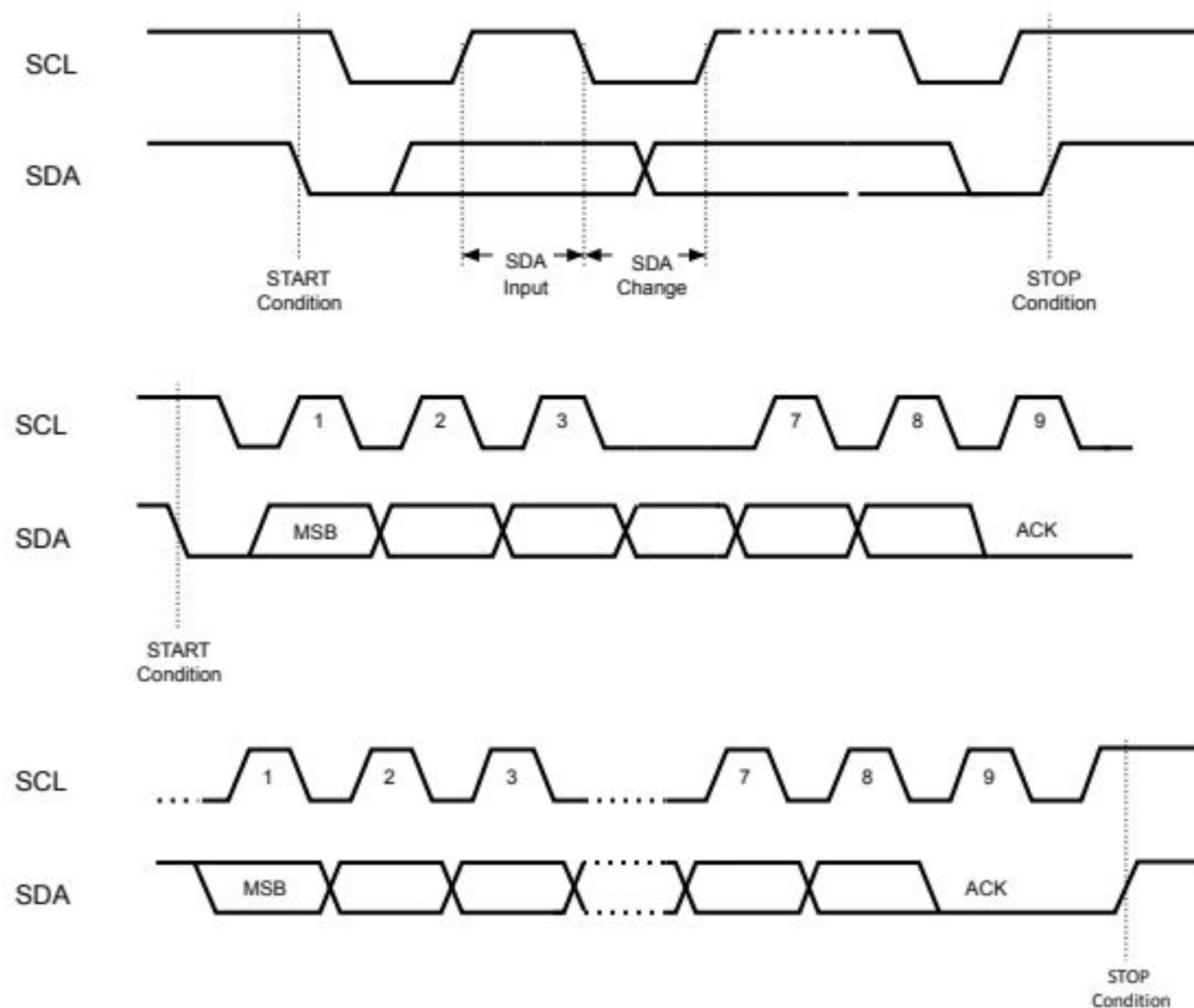
Figure 7. I 2 C bus protocol
