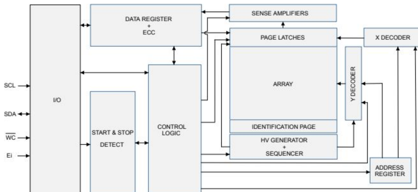
Figure 6. Block diagram
