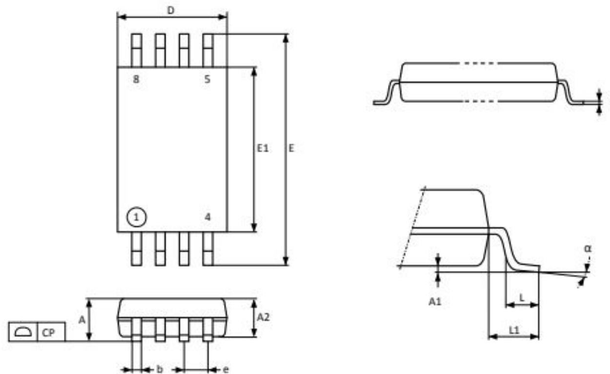
Figure 20. TSSOP8 – Outline
