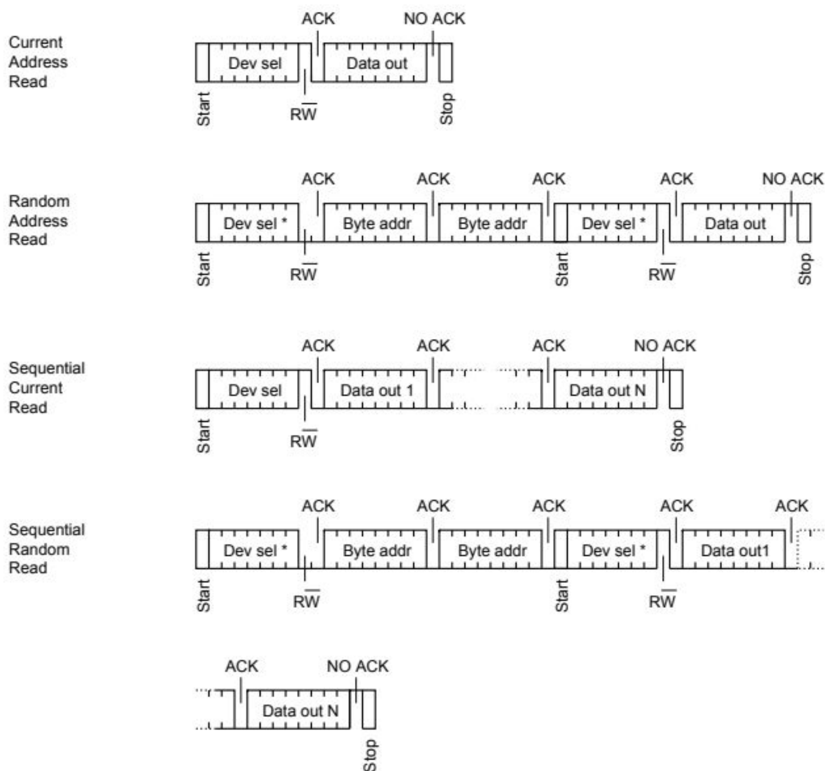
Figure 11. Read mode sequences
