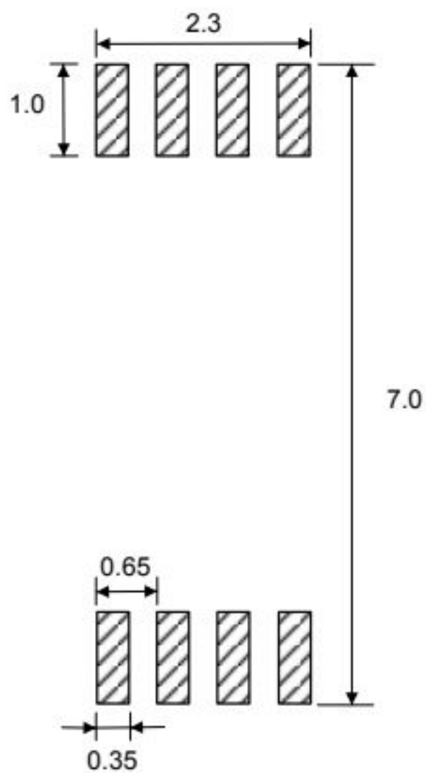
Figure 21. TSSOP8 – Recommended footprint
