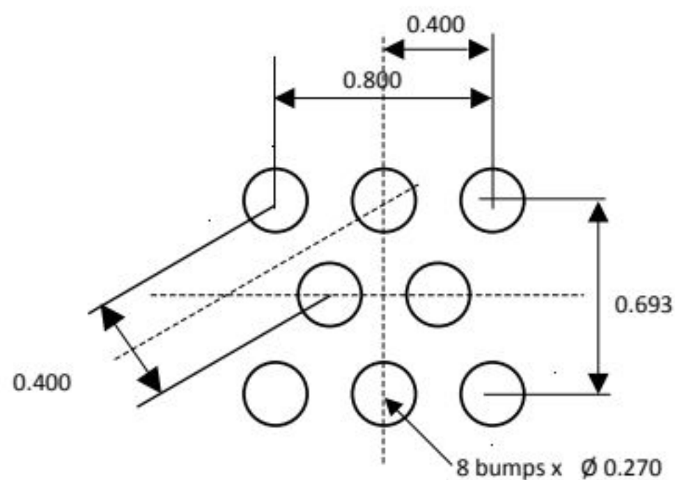
Figure 25. WLCSP8 - Recommended footprint
