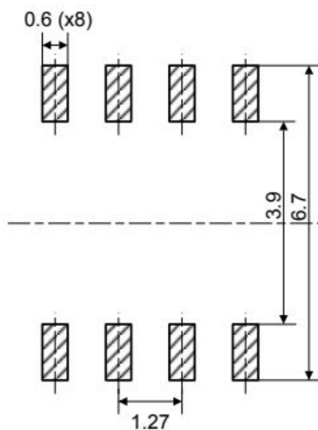
Figure 23. SO8N - Recommended footprint
