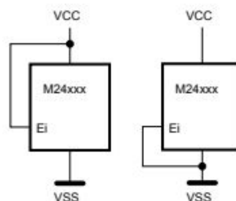
Figure 5. Chip enable inputs connection
