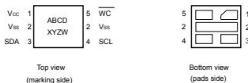
Figure 3. UDFPN5 (DFN5) package connections
