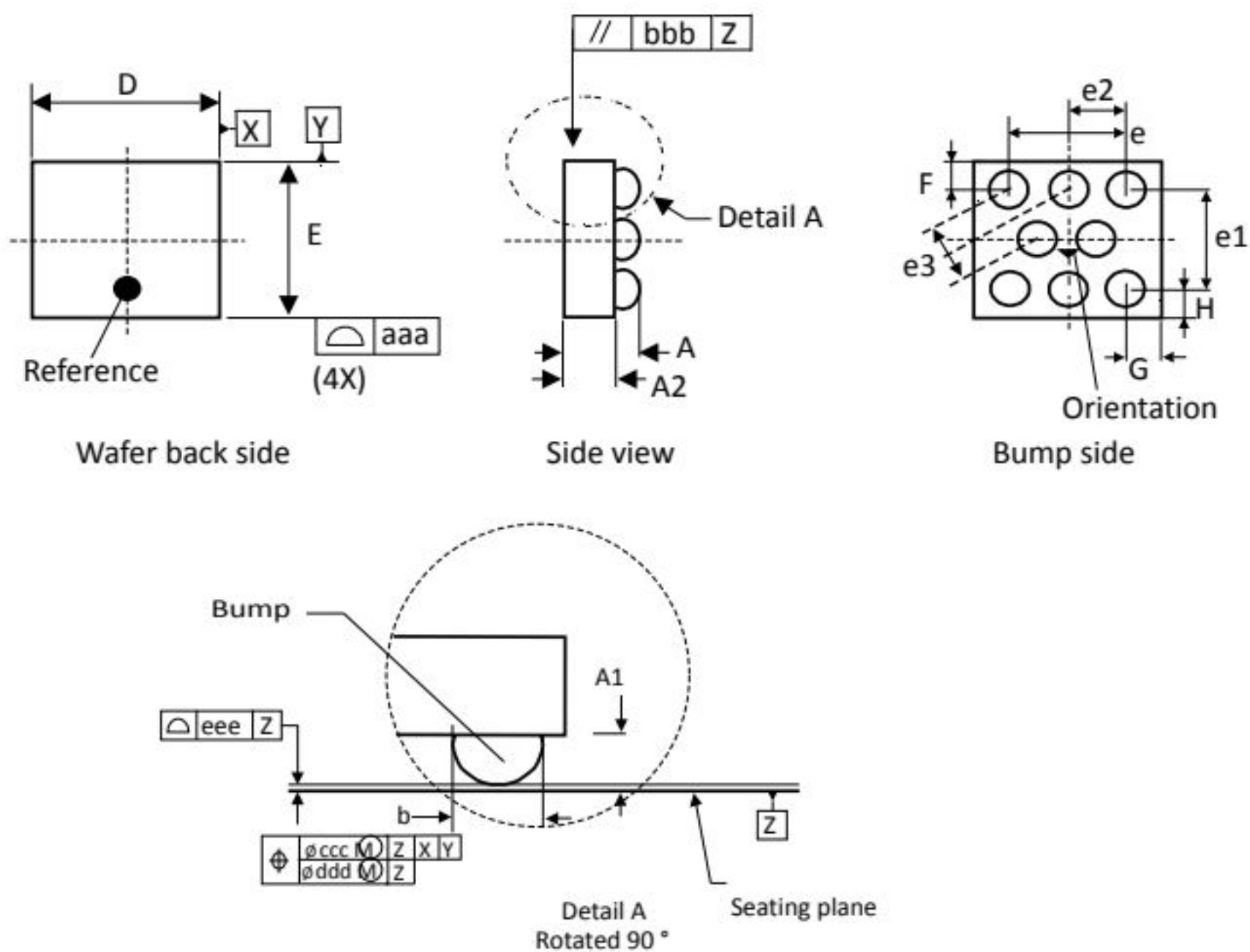
Figure 24. WLCSP8 - Outline
