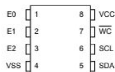
Figure 2. 8-pin package connections, top view
