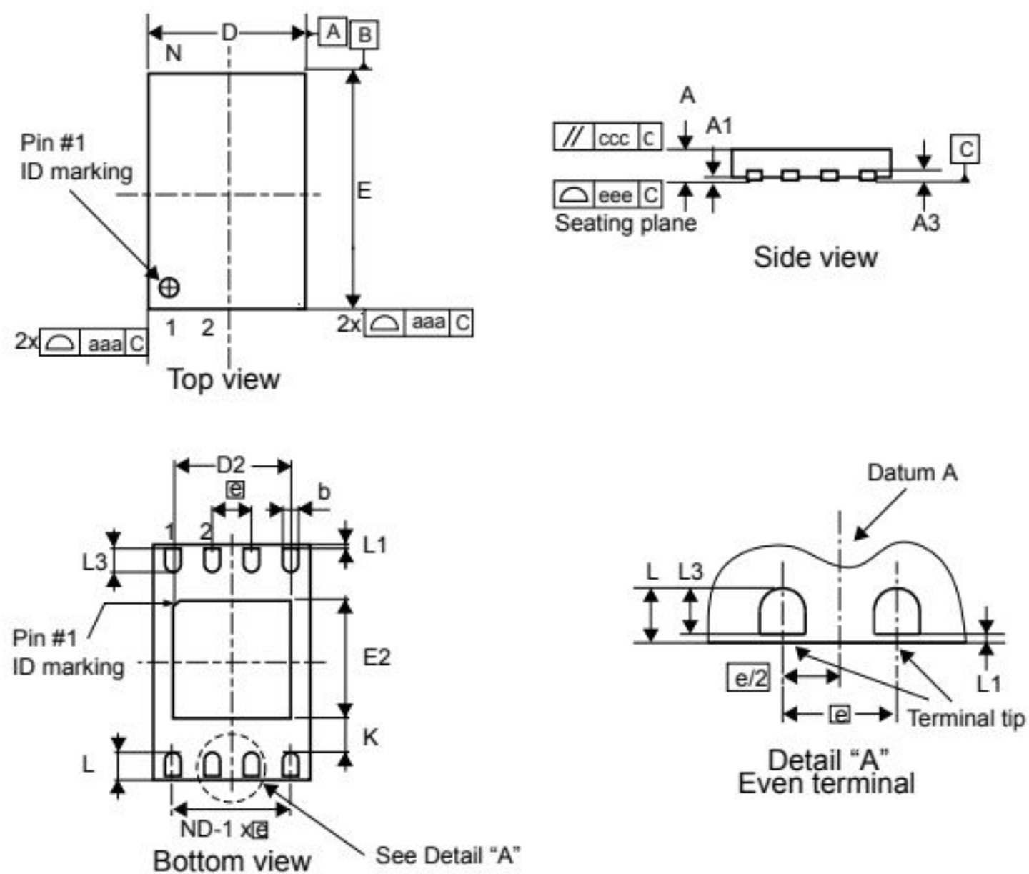
Figure 18. UFDFPN8 - Outline
