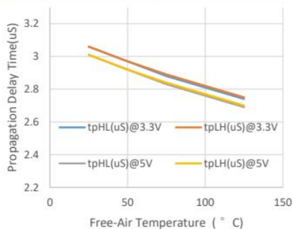
Figure8. Propagation Delay Time vs. Free-Air Temperature
