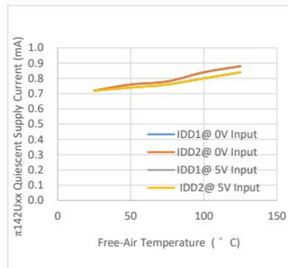
Figure 14 \pi 142Uxx Quiescent Supply Current with 5V Supply vs. Free-Air Temperature
