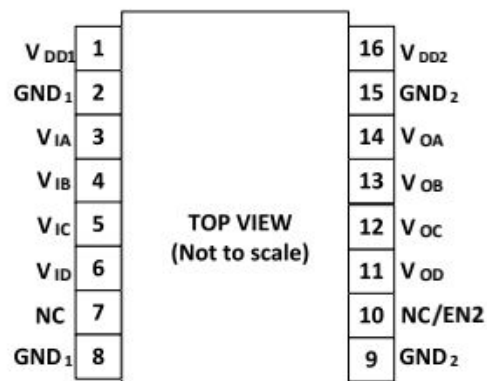
Figure3 \pi 140U_{xx} Pin Configuration
