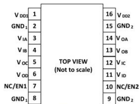
Figure 5. \pi 142U_{xx} Pin Configuration
