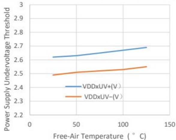
Figure7. UVLO vs. Free-Air Temperature
