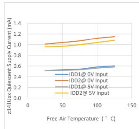
Figure 12 \pi 141Uxx Quiescent Supply Current with 5V Supply vs. Free-Air Temperature
