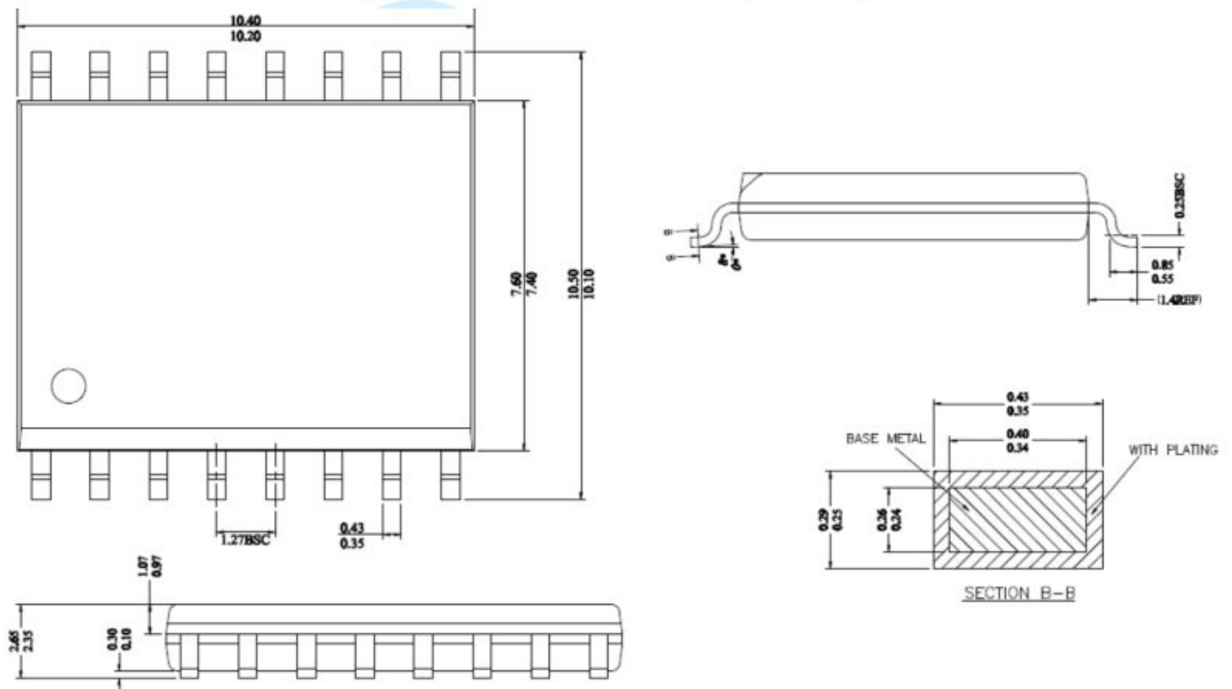
Figure 20. 16-Lead Wide Body Outline Package [16-Lead SOIC_W]
