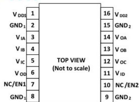
Figure4. \pi 141U_{xx} Pin Configuration
