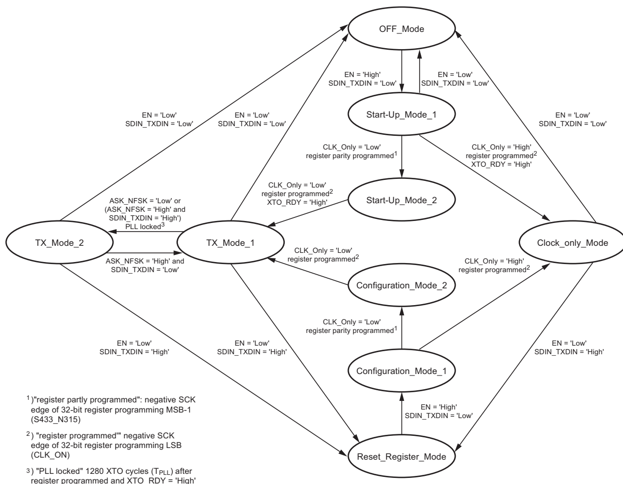
Figure 6-5. State Diagram of Operating Modes
