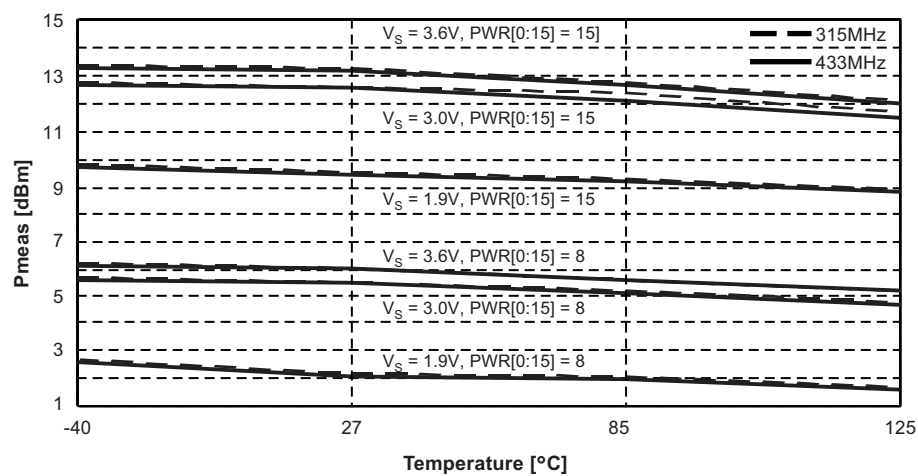
Figure 4-3. Typical Measured Output Power
