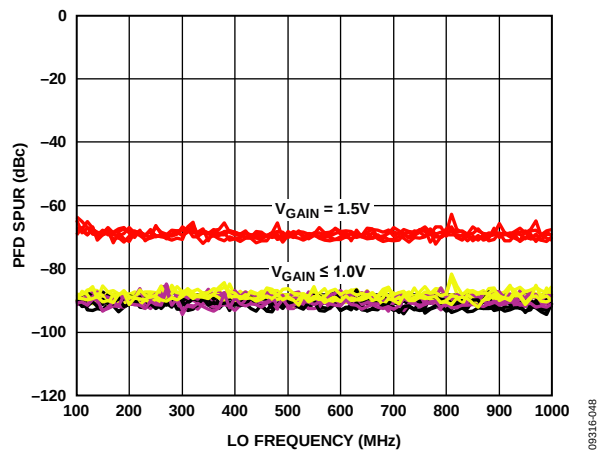
Figure 36. PFD Spurs at 27 MHz from Carrier vs. LO Frequency, Channel Gain, Supply, and Temperature
