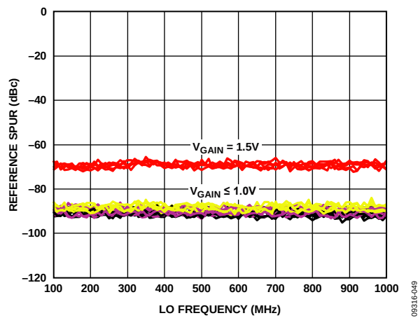
Figure 35. Reference Spurs at 13.5 MHz from Carrier vs. LO Frequency, Channel Gain, Supply, and Temperature
