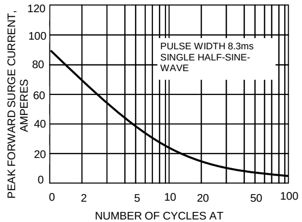
FIG.2-MAXIMUM NON-REPETITIVE SURGE
