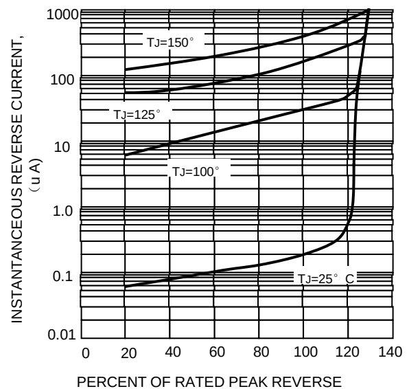
FIG.4-TYPICAL REVERSE
