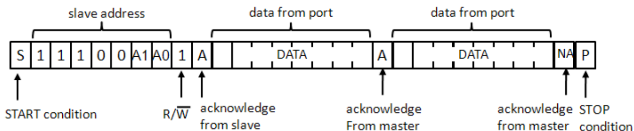
Figure 9: Read Input Port Register
