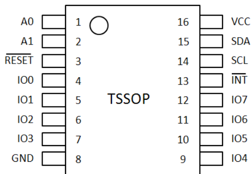
Figure 1: TSSOP-16 (Top View)
