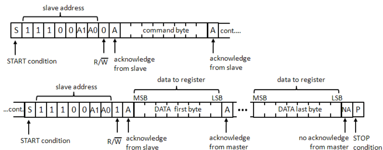
Figure 8: Read from Registers
