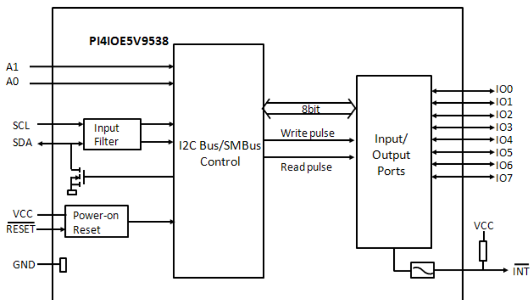
Figure 4: Block Diagram of PI4IOE5V9538
