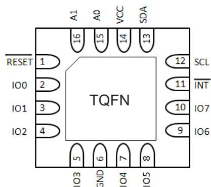
Figure 2: TQFN 4x4-16 (Top View)
