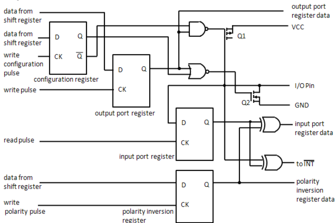
Figure 5: Simplified Schematic of I/Os
