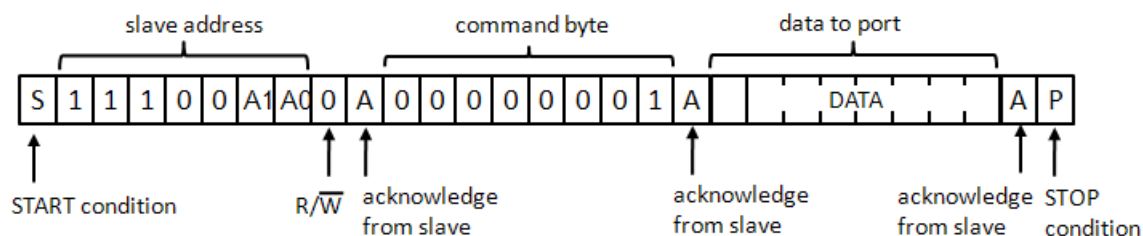
Figure 6: Write to Output Registers
