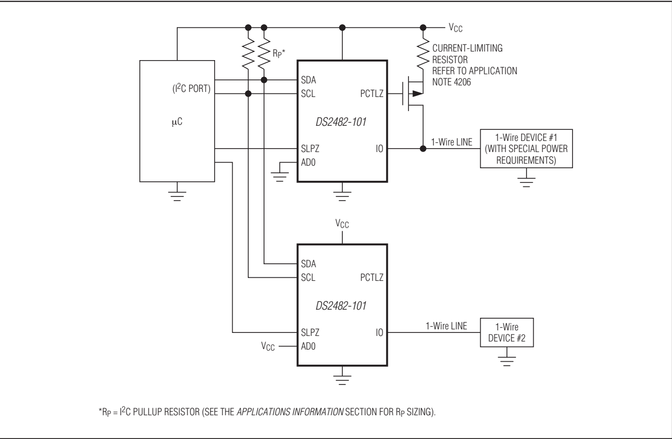
Figure 10. Application Schematic
