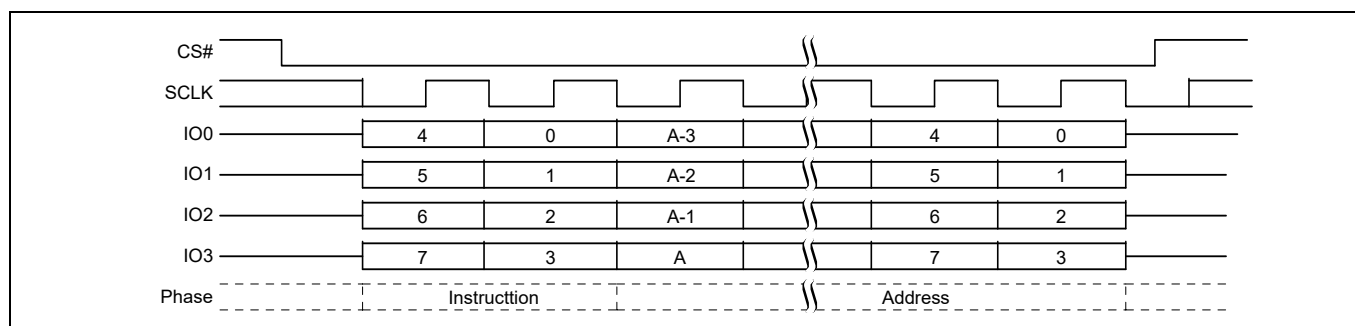
Figure 83 Half Block Erase (HBE 52h or 4HBE 53h) QPI mode command sequence [44, 45]
