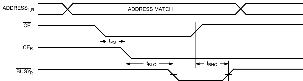
Figure 13. Busy Timing Diagram No. 1 ( \overline{CE} Arbitration) [29]
