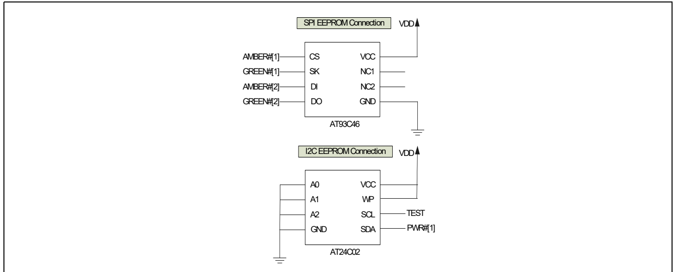
Figure 8 EEPROM connections
