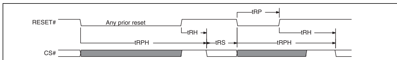
Figure 33 Hardware reset
