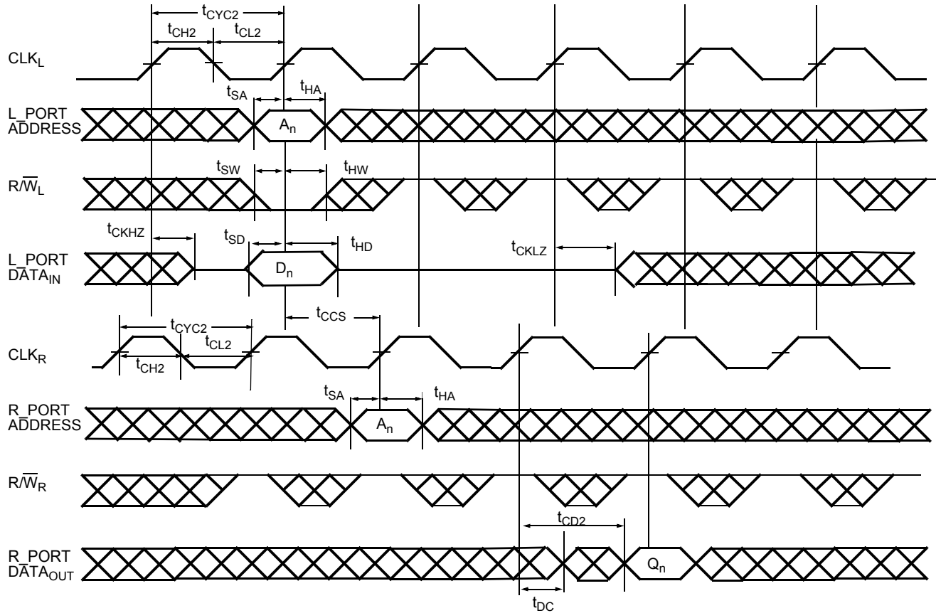
Figure 16. Left_Port (L_Port) Write to Right_Port (R_Port) Read [50, 51, 52]
