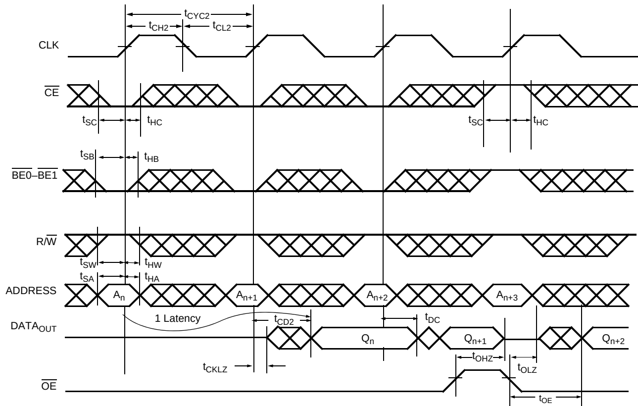
Figure 9. Read Cycle [12, 30, 31, 32, 33]
