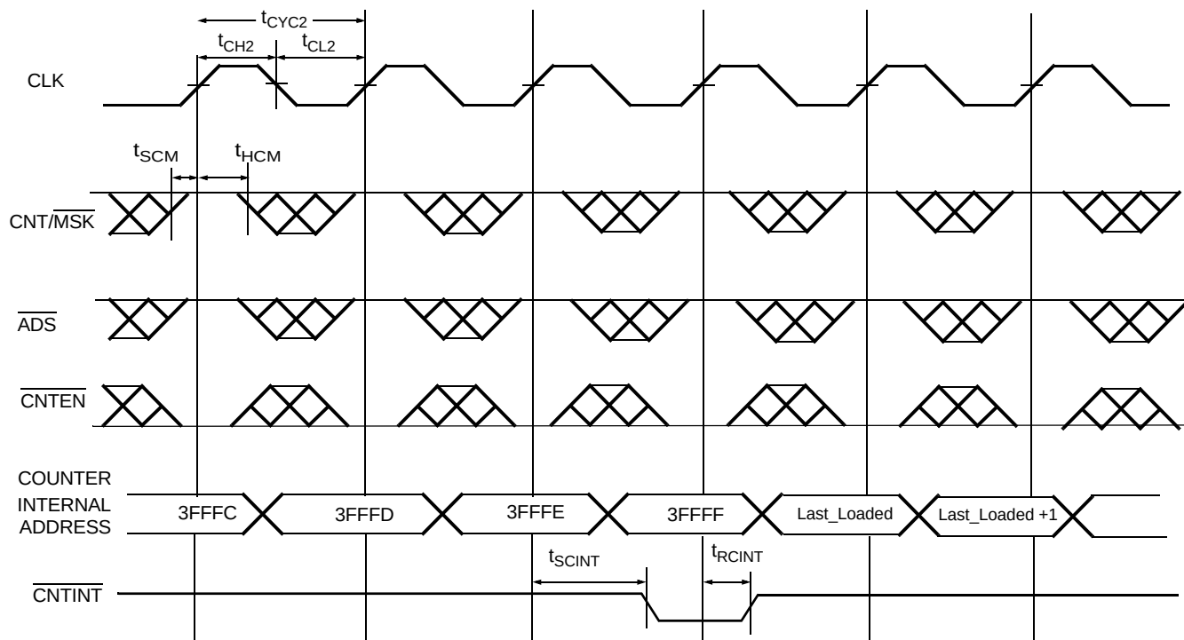
Figure 18. Counter Interrupt and Retransmit [15, 42, 50, 51, 52, 53]
