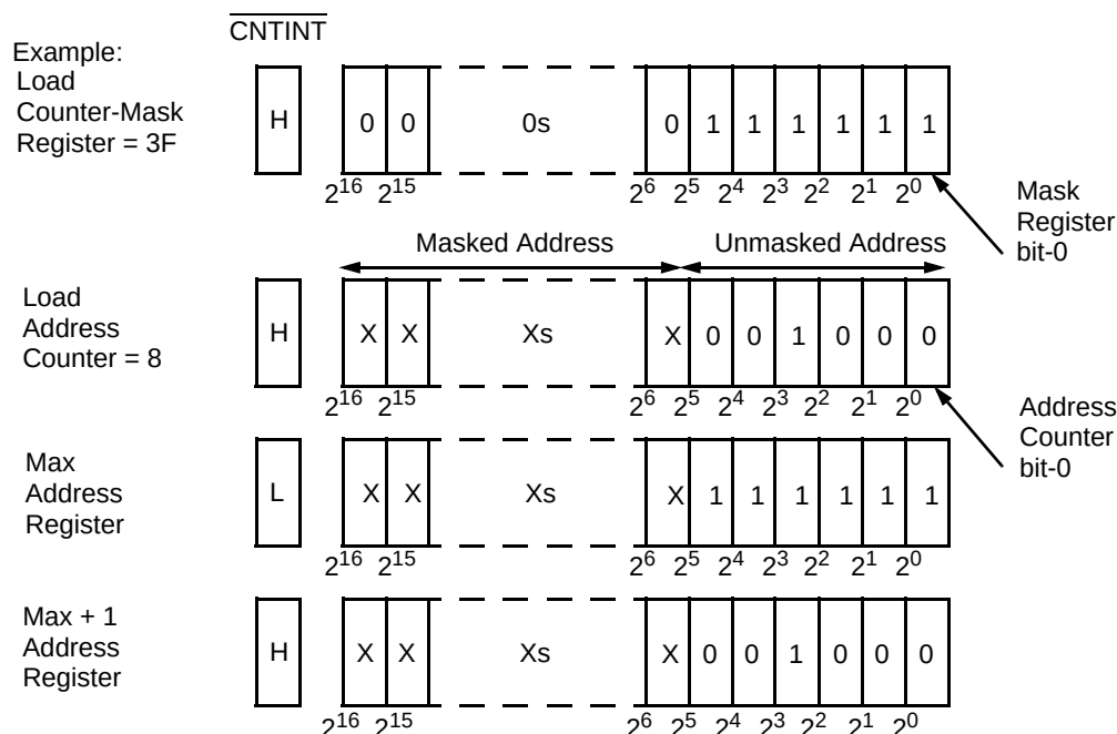
Figure 4. Programmable Counter-Mask Register Operation [2, 20]
