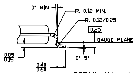
DETAIL 'A' 51-85095-**
