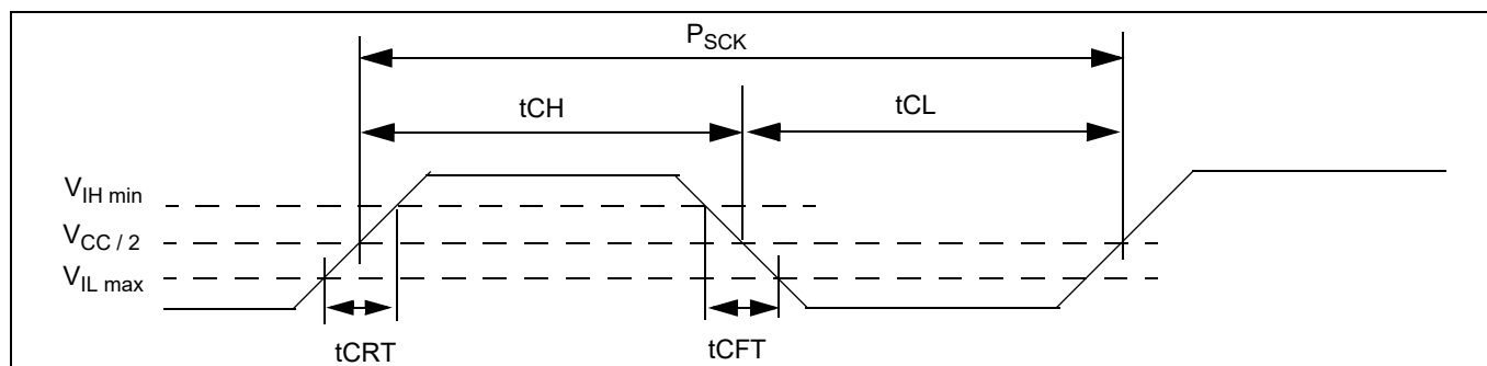
Figure 142 Clock timing
