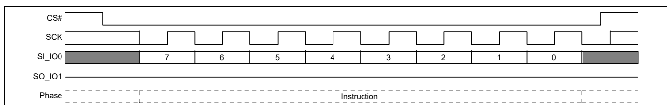
Figure 121 Software / Mode Bit Reset command sequence
