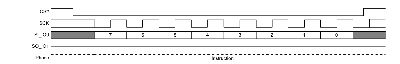
Figure 123 Deep Power Down (DPD) command sequence
