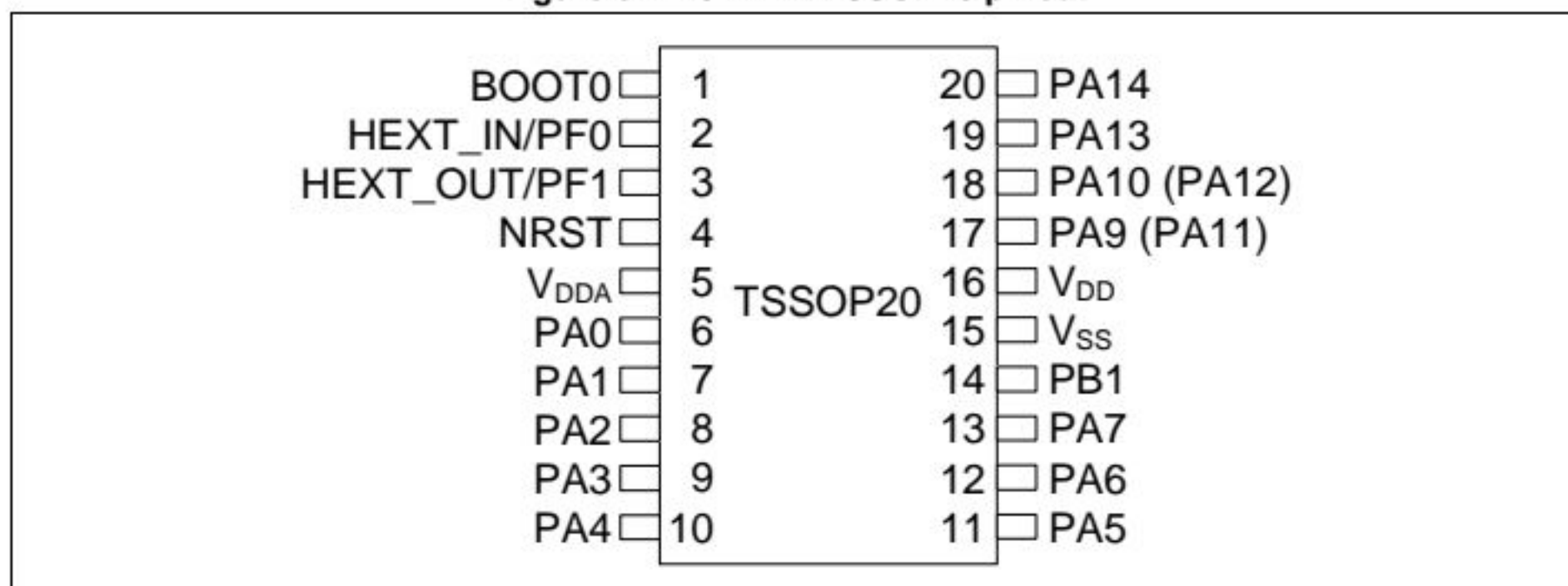
Figure 6. AT32F421 TSSOP20 pinout
