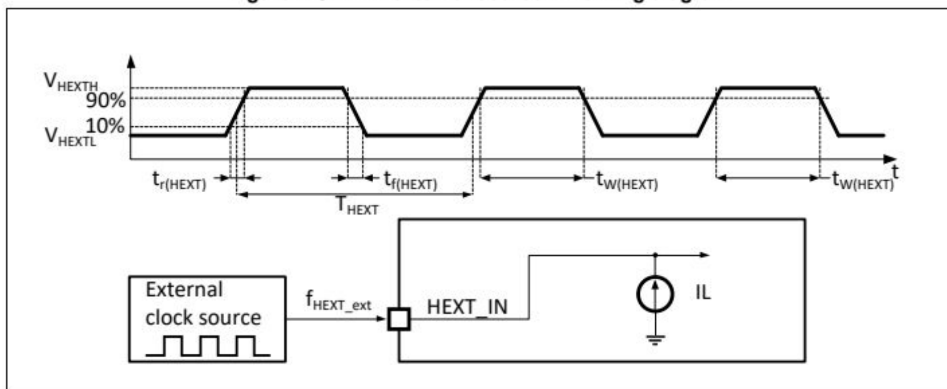
Figure 14. HEXT external source AC timing diagram
