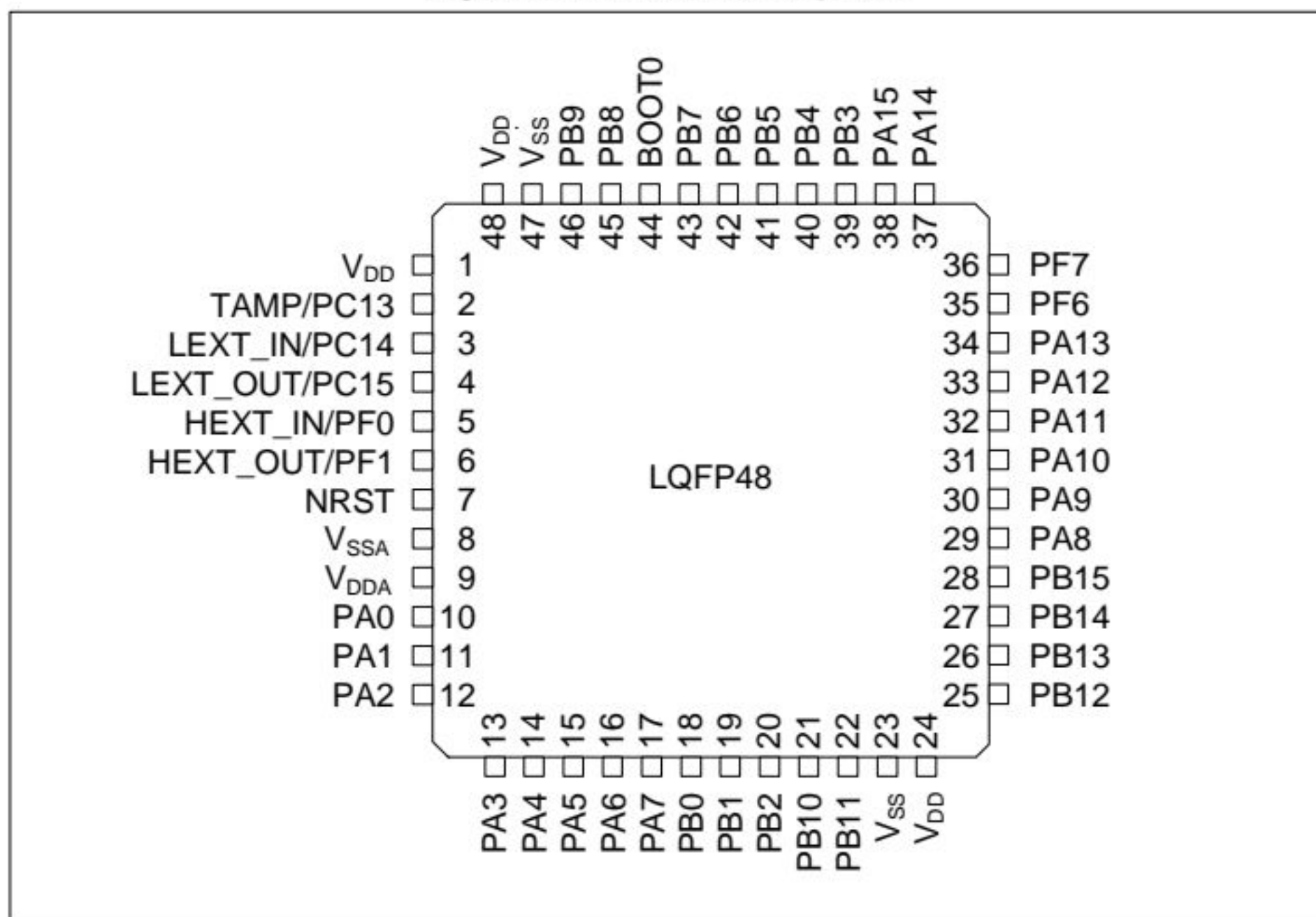
Figure 2. AT32F421 LQFP48 pinout
