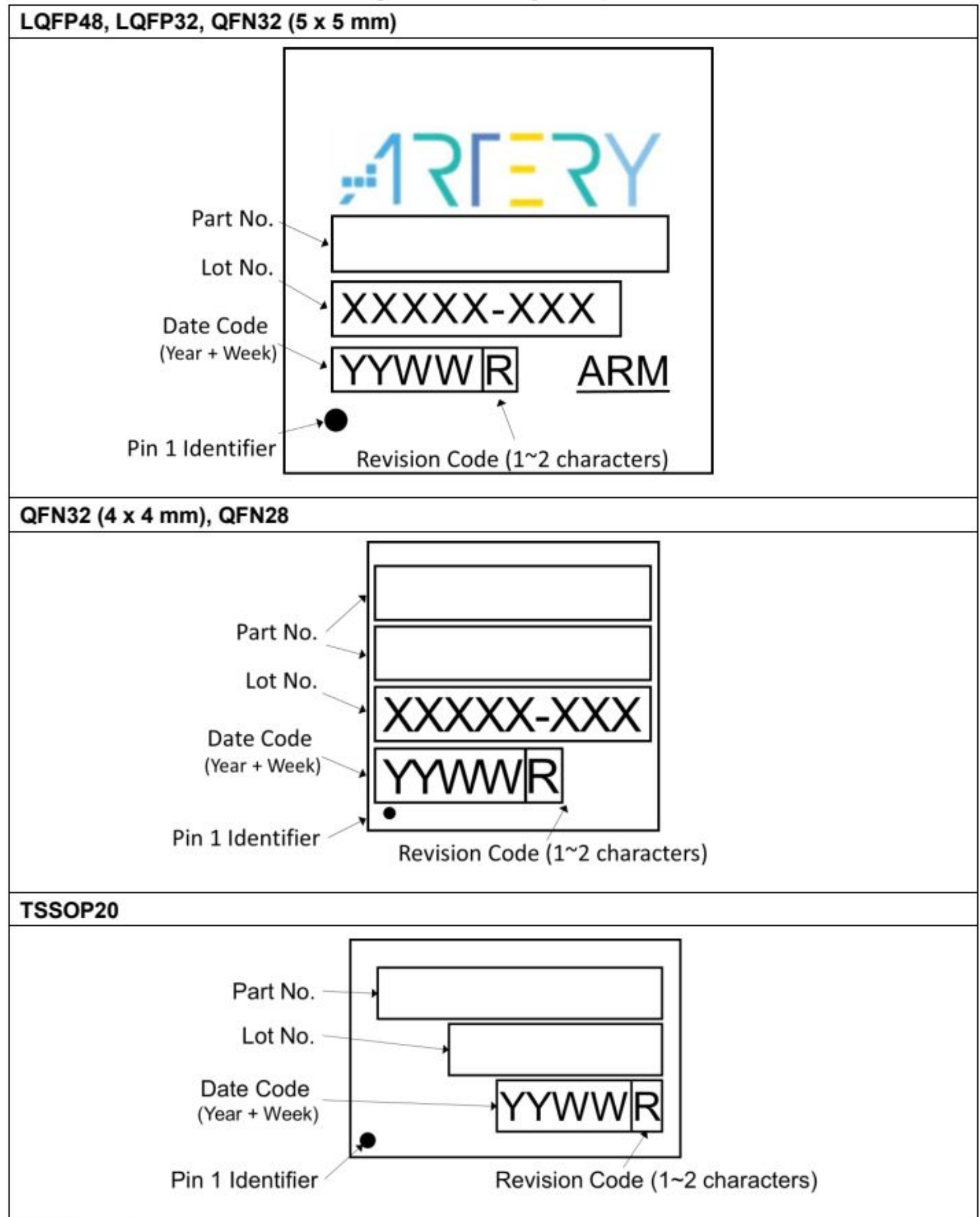
Figure 34. Marking example
