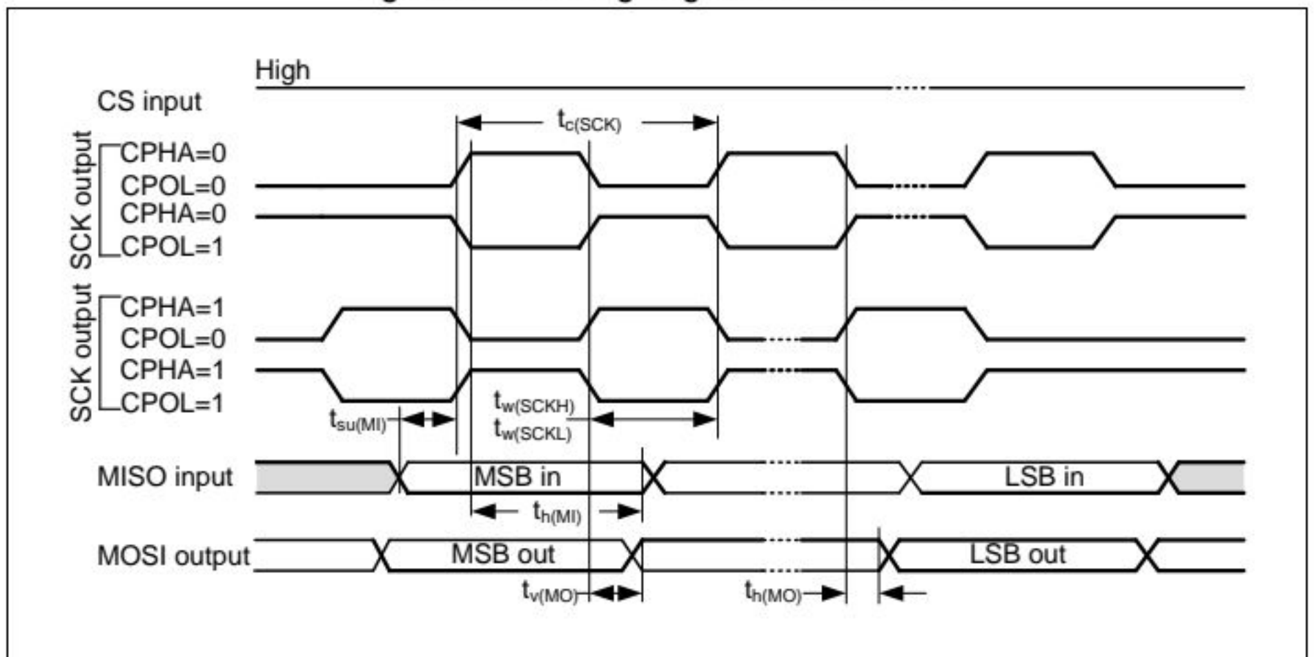
Figure 21. SPI timing diagram – master mode
