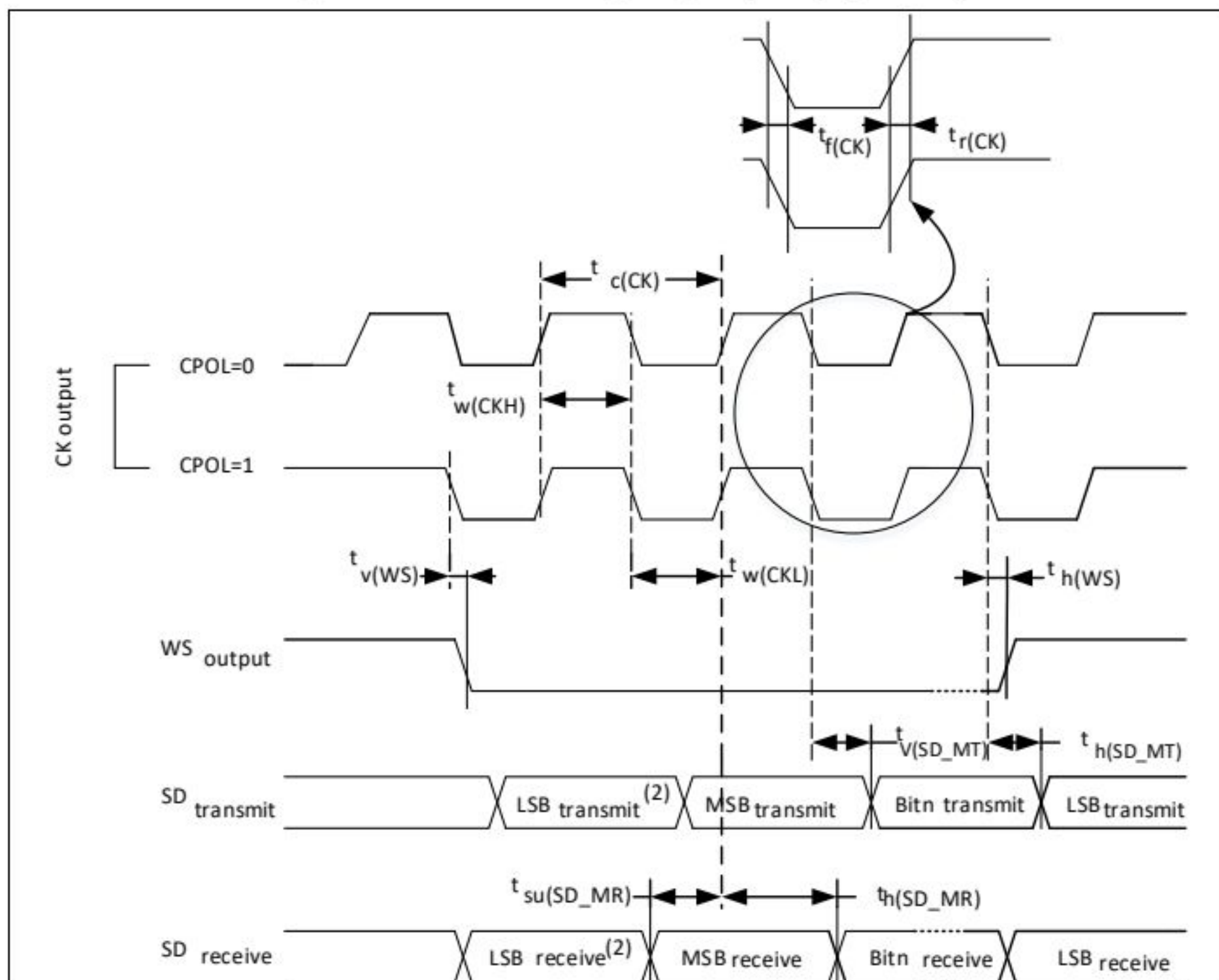
Figure 23. I 2 S master timing diagram (Philips protocol)
