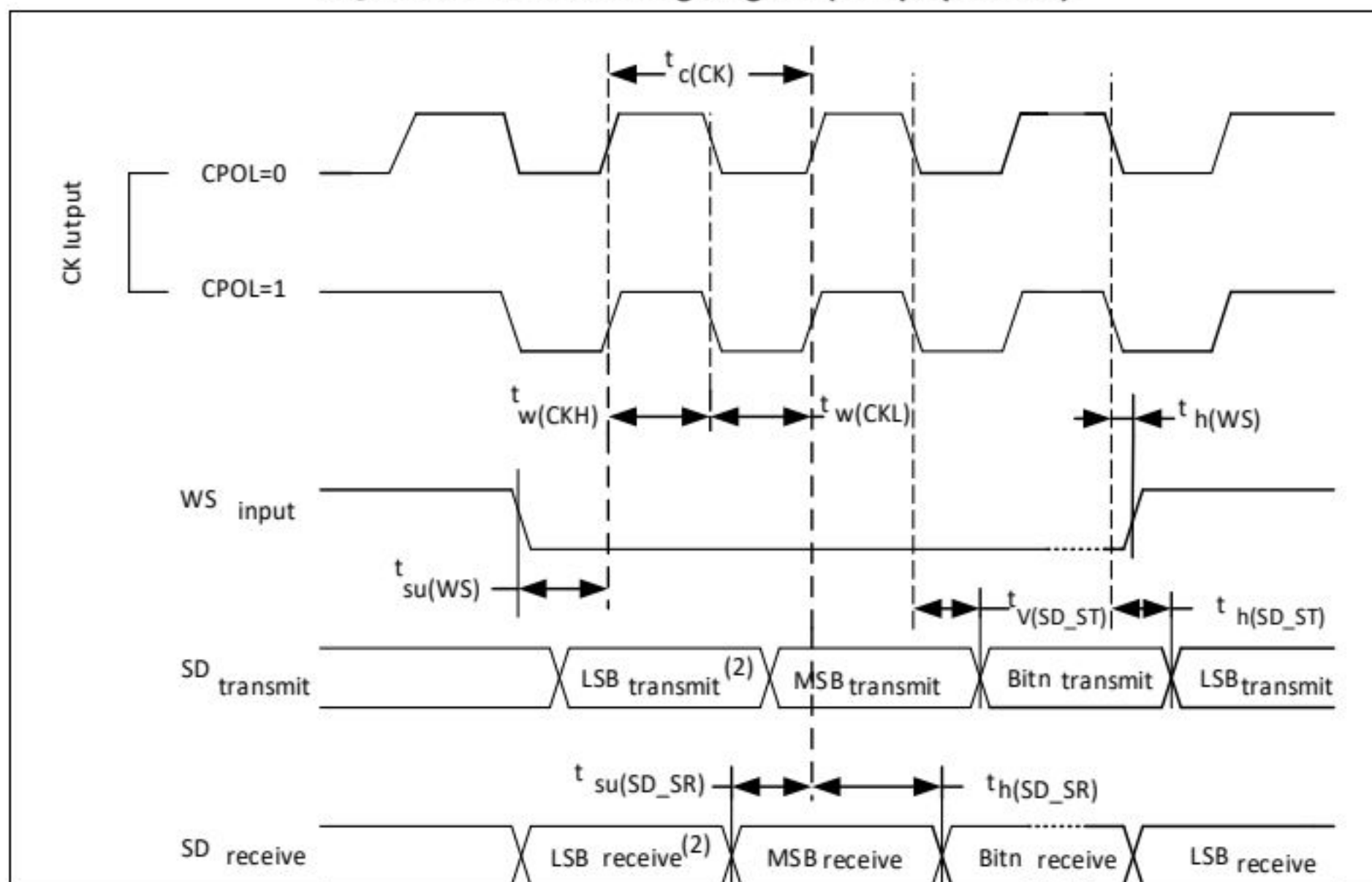
Figure 22. I 2 S slave timing diagram (Philips protocol)
