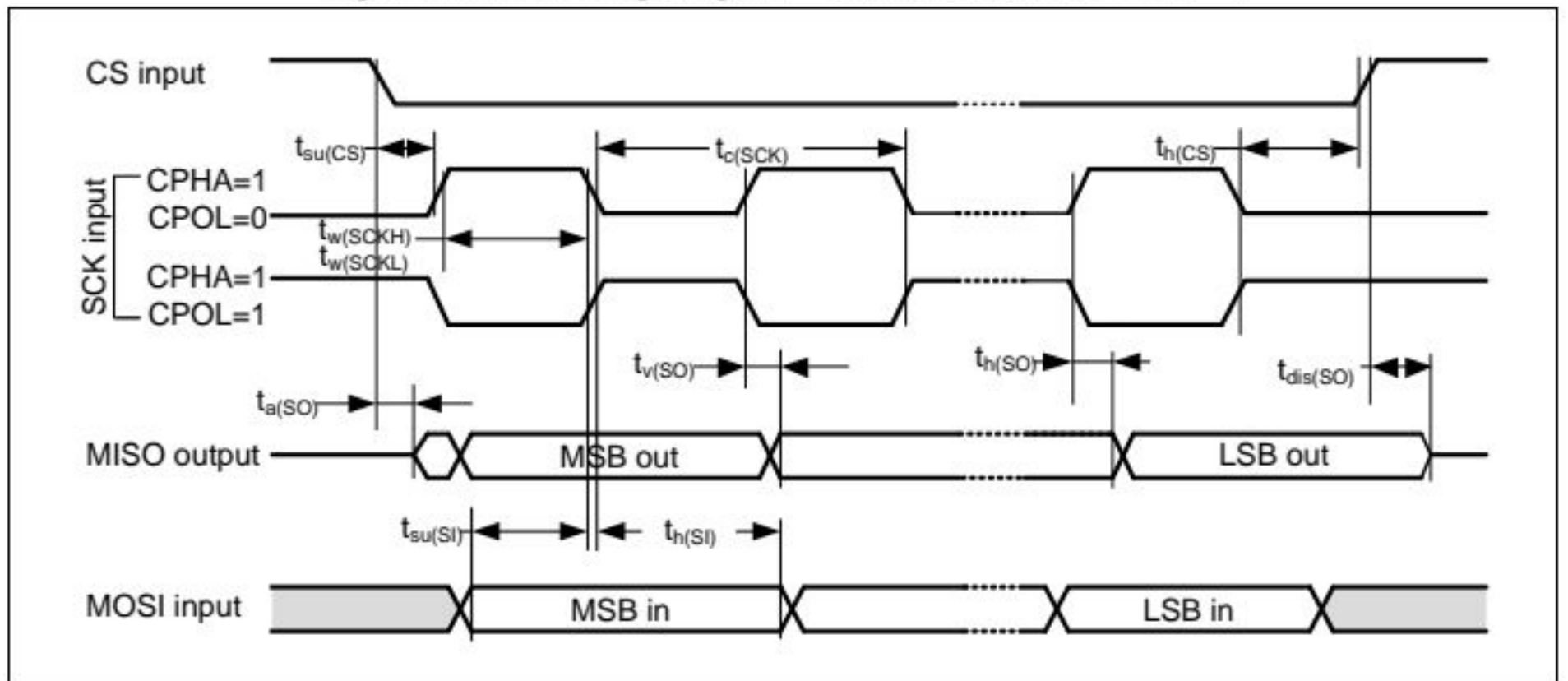
Figure 20. SPI timing diagram – slave mode and CPHA = 1
