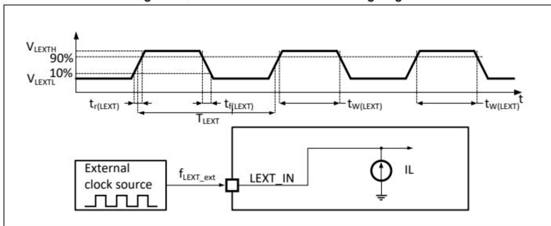
Figure 16. LEXT external source AC timing diagram
