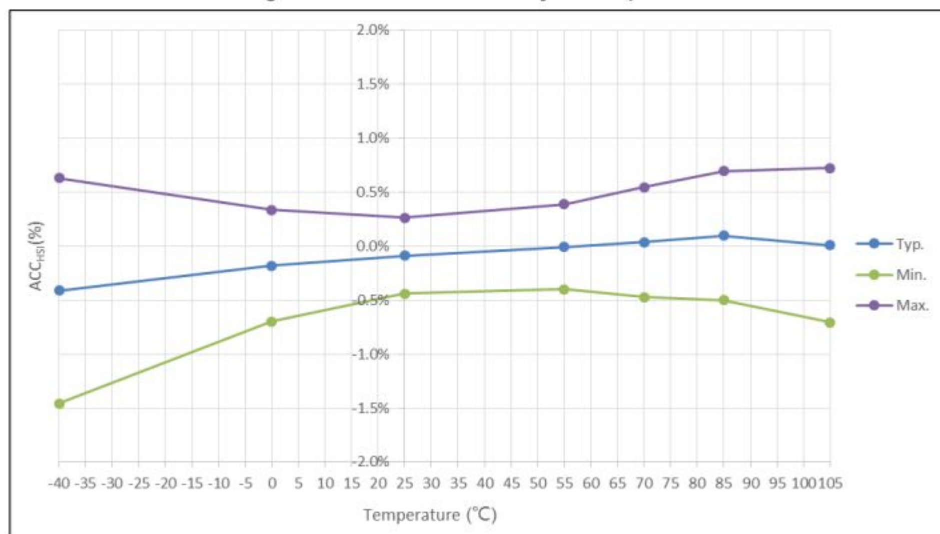
Figure 17. HICK clock accuracy vs. temperature
