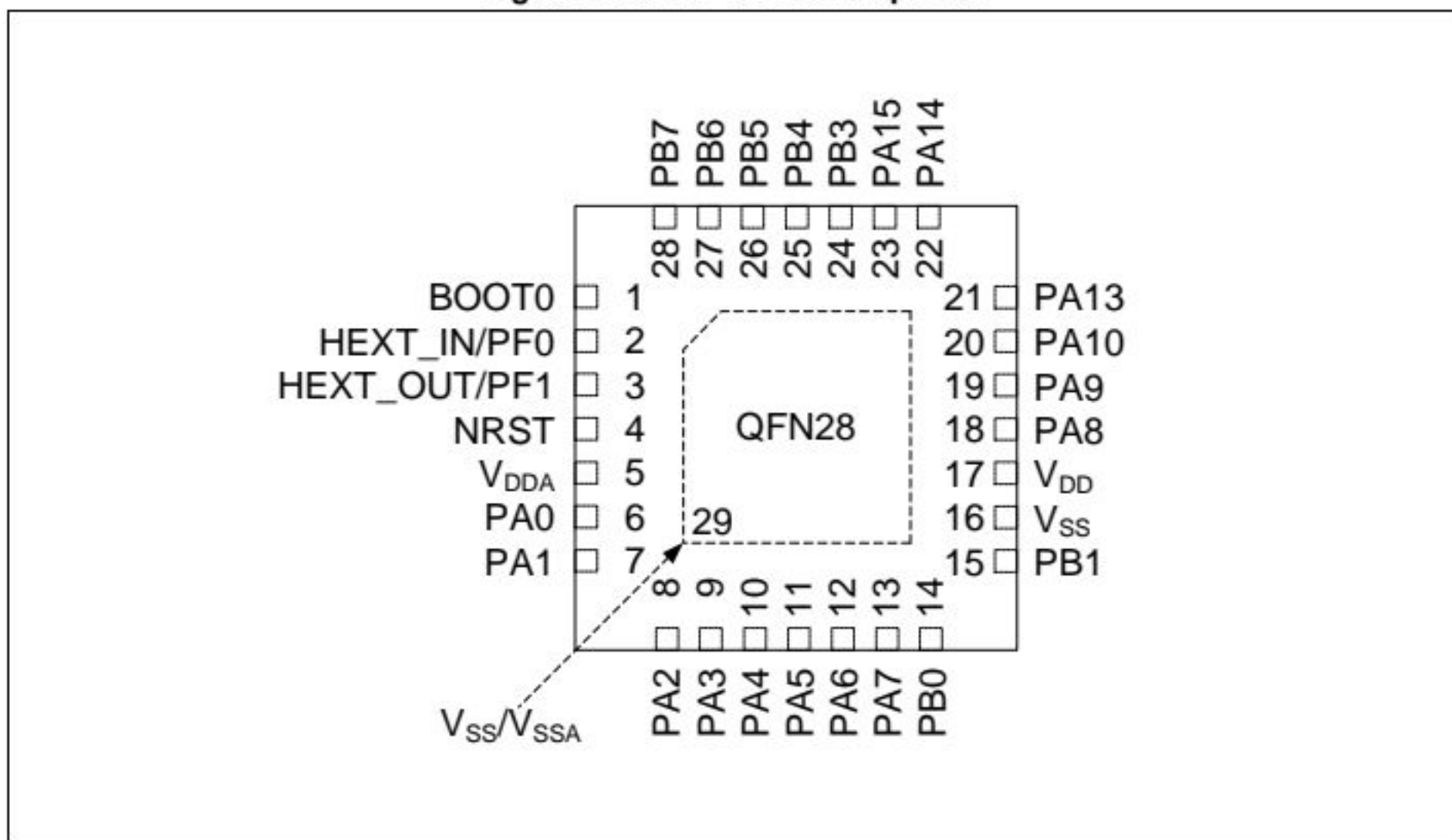
Figure 5. AT32F421 QFN28 pinout
