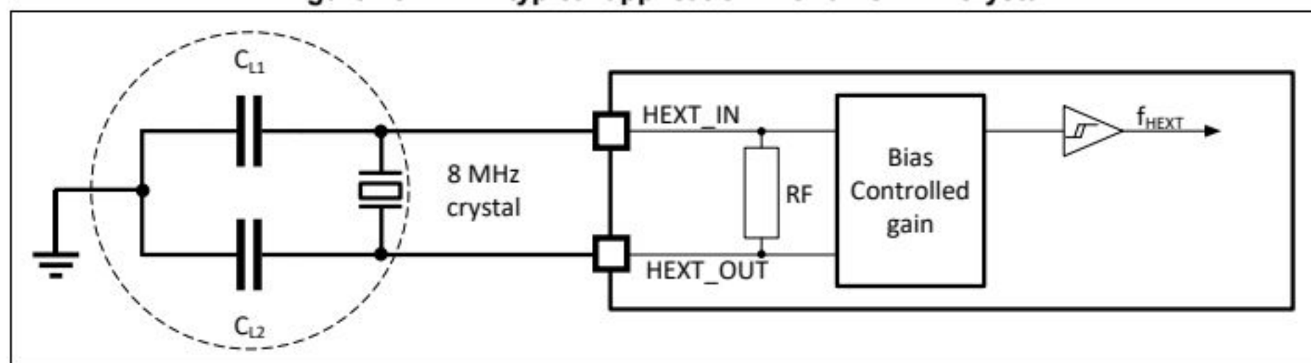
Figure 13. HEXT typical application with an 8 MHz crystal
