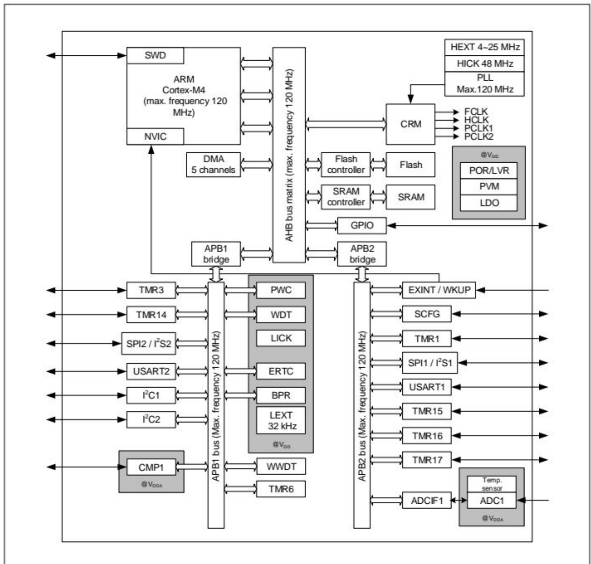
Figure 1. AT32F421 block diagram
