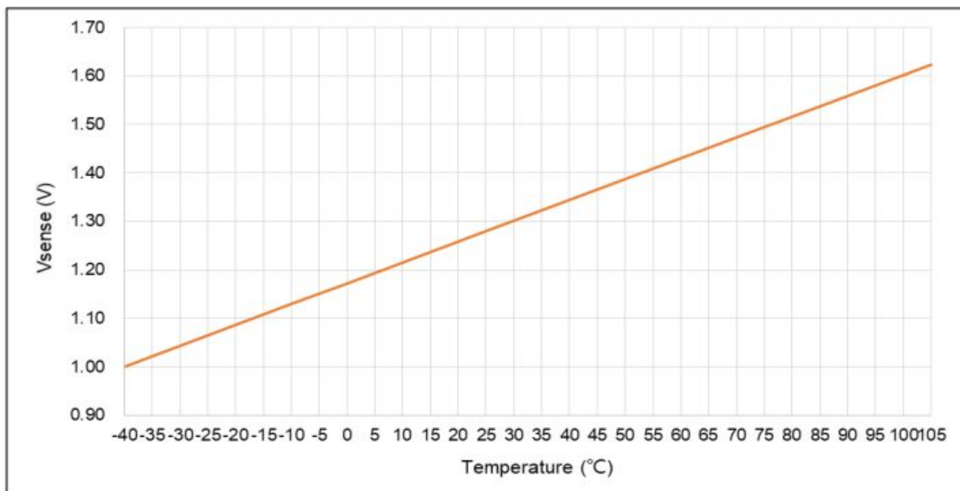
Figure 26. V_{TS} vs. temperature (ideal curve)
