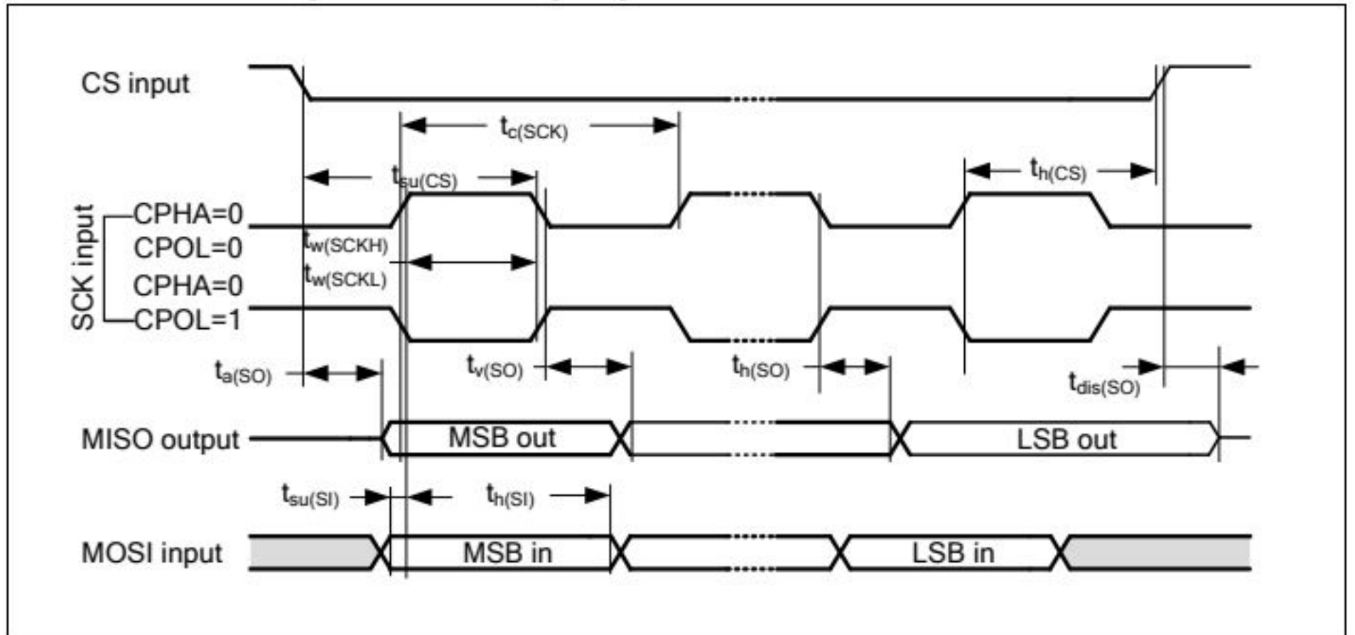
Figure 19. SPI timing diagram – slave mode and CPHA = 0
