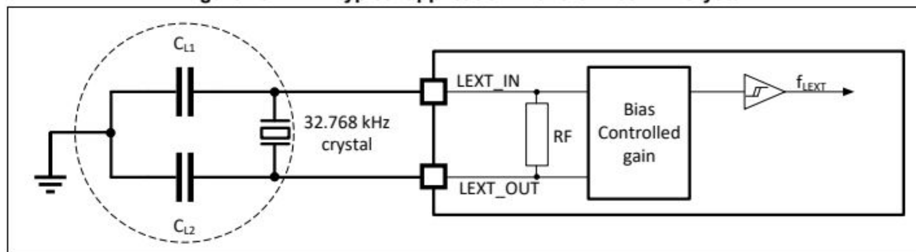
Figure 15. LEXT typical application with a 32.768 kHz crystal
