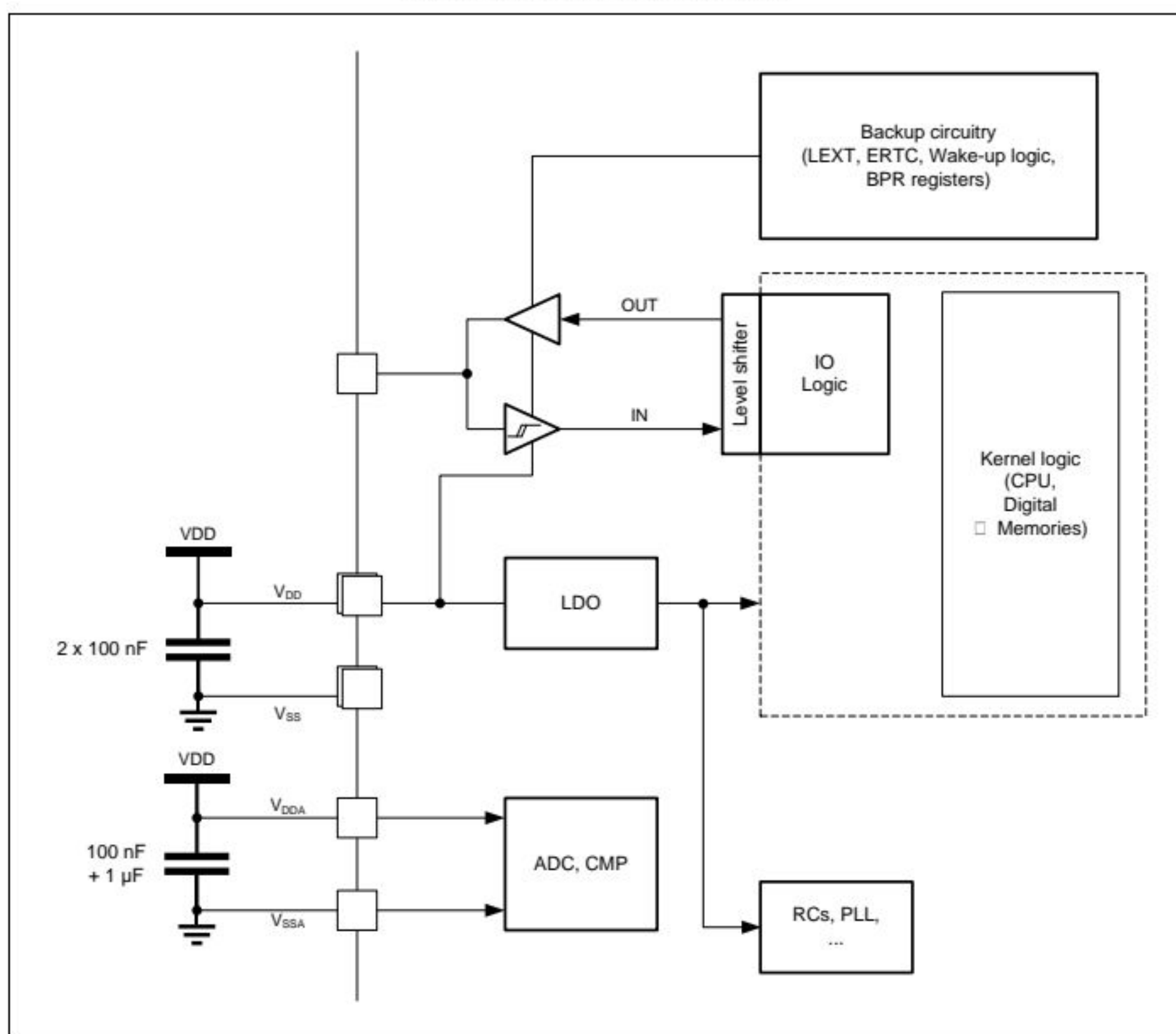
Figure 8. Power supply scheme
