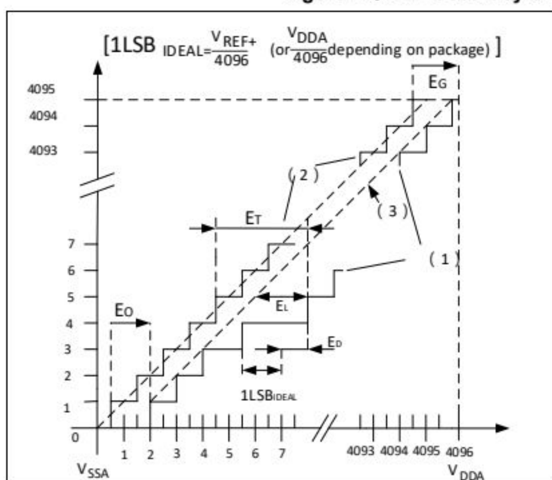
Figure 24. ADC accuracy characteristics
