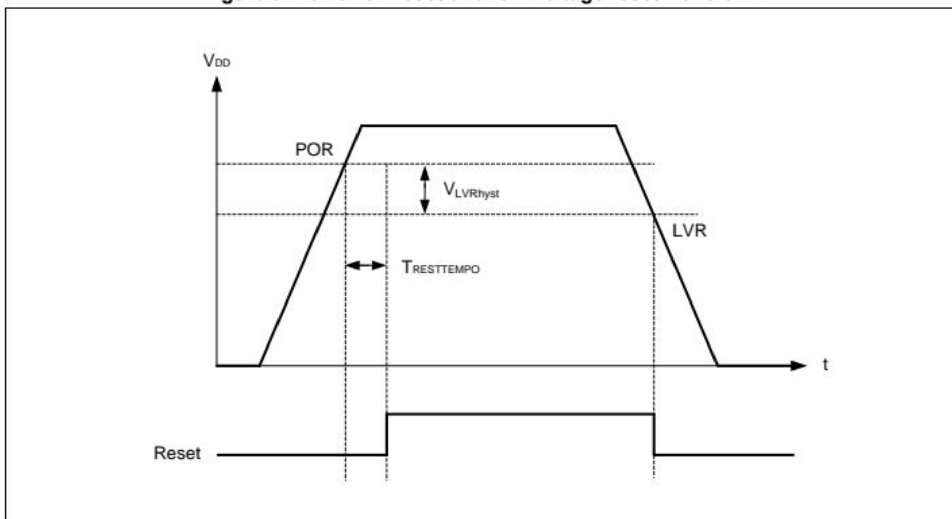
Figure 9. Power-on reset and low voltage reset waveform
