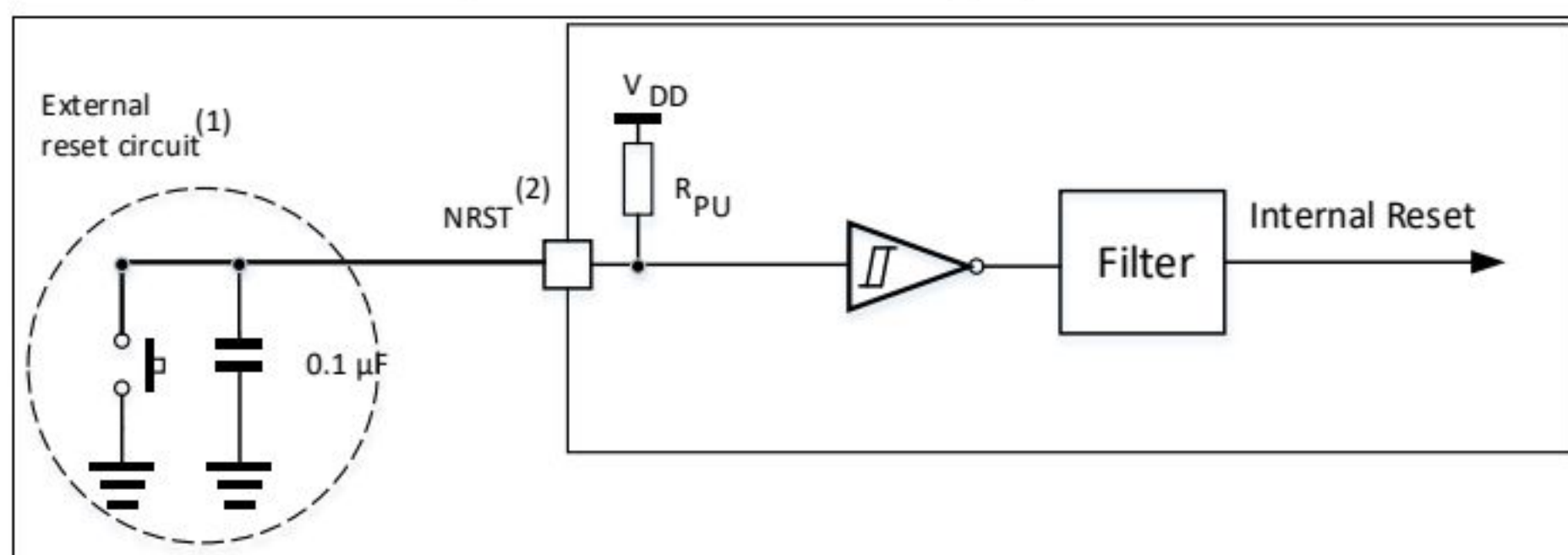
Figure 18. Recommended NRST pin protection
