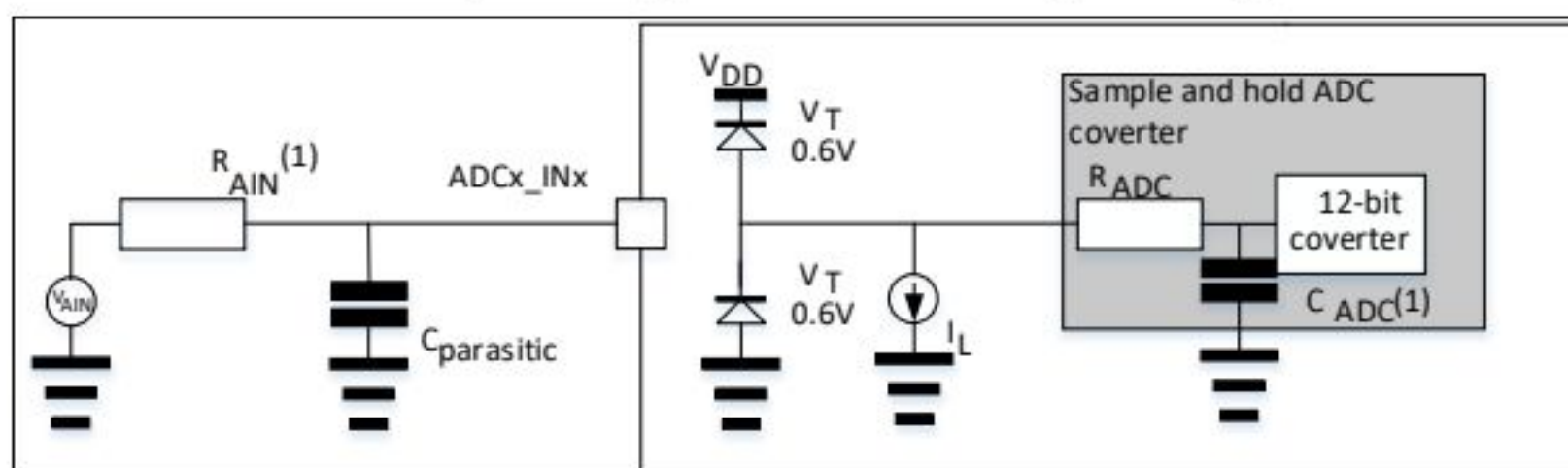
Figure 25. Typical connection diagram using the ADC
