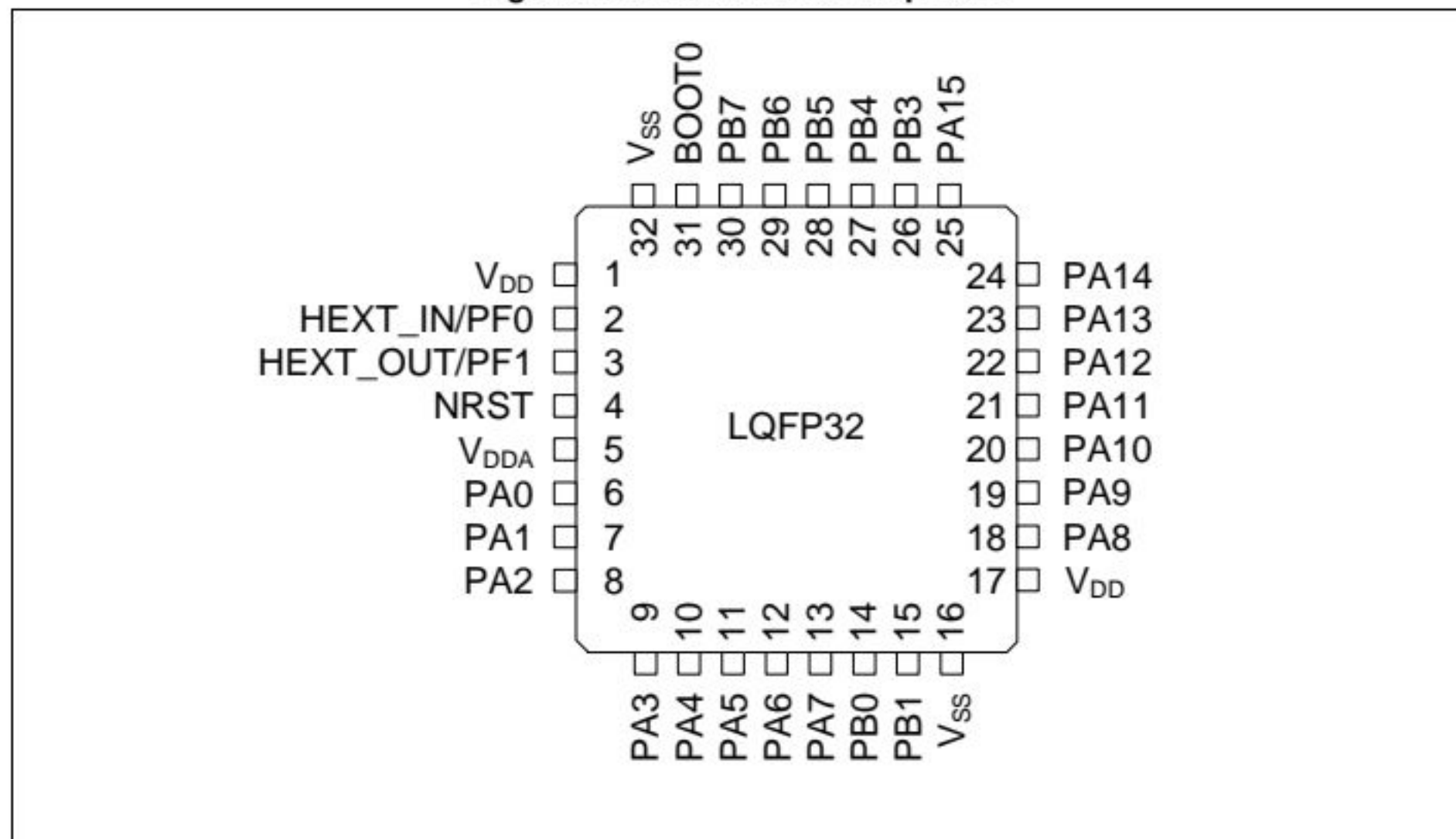
Figure 3. AT32F421 LQFP32 pinout
