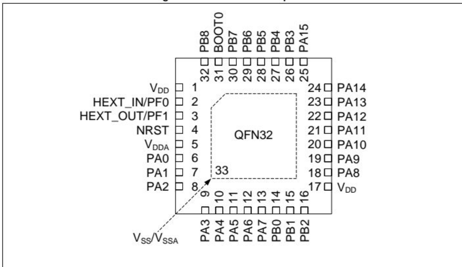
Figure 4. AT32F421 QFN32 pinout
