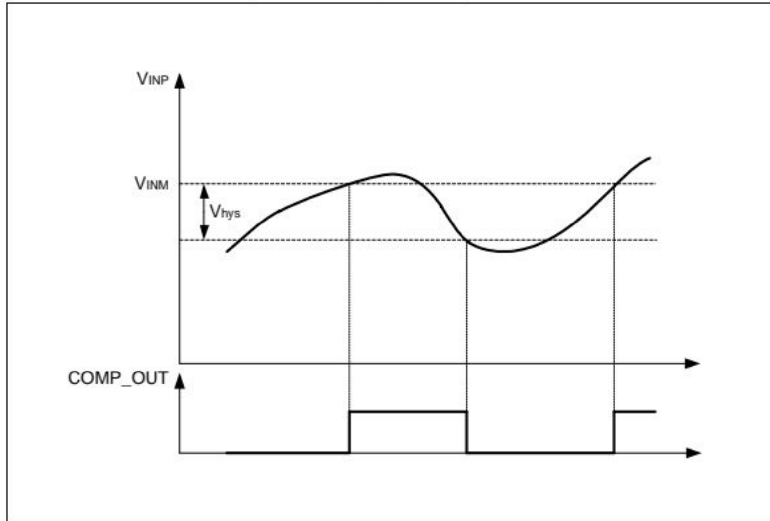
Figure 27. Comparator hysteresis
