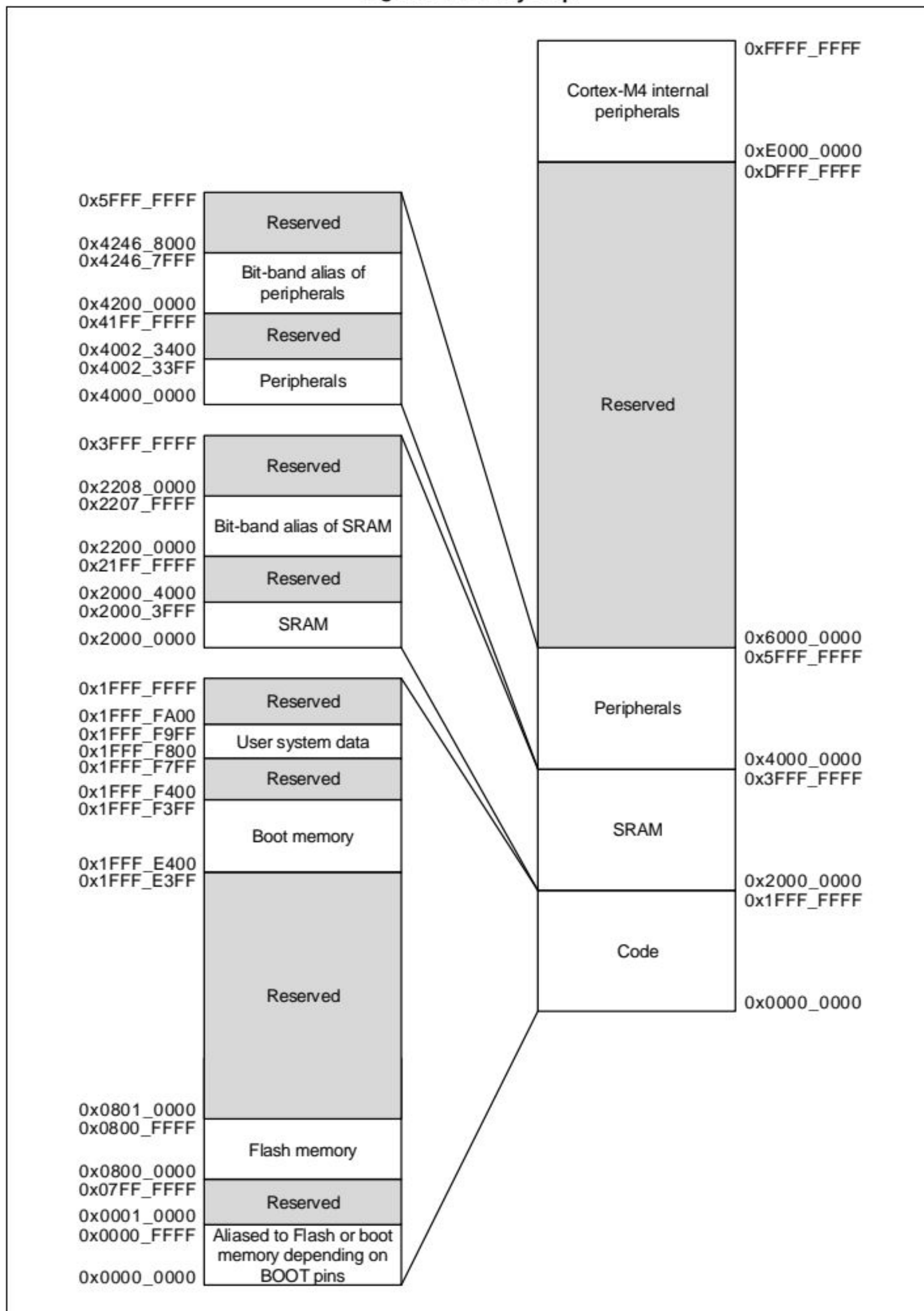
Figure 7. Memory map
