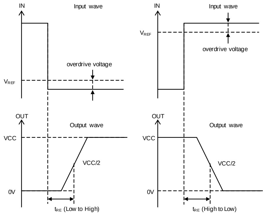
Figure 113. Response Time
