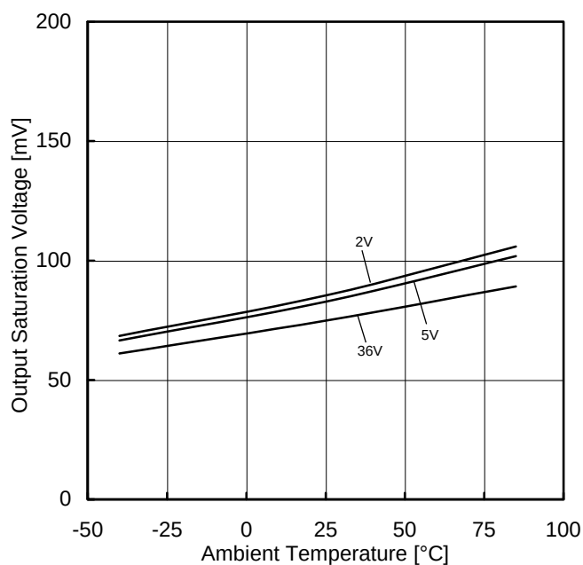
Figure 6. Output Saturation Voltage vs Ambient Temperature ( I_{OL}=4\text{mA} )
