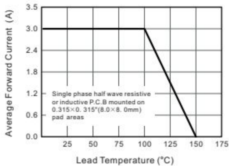
Fig.2 Maximum Average Forward Current Rating
