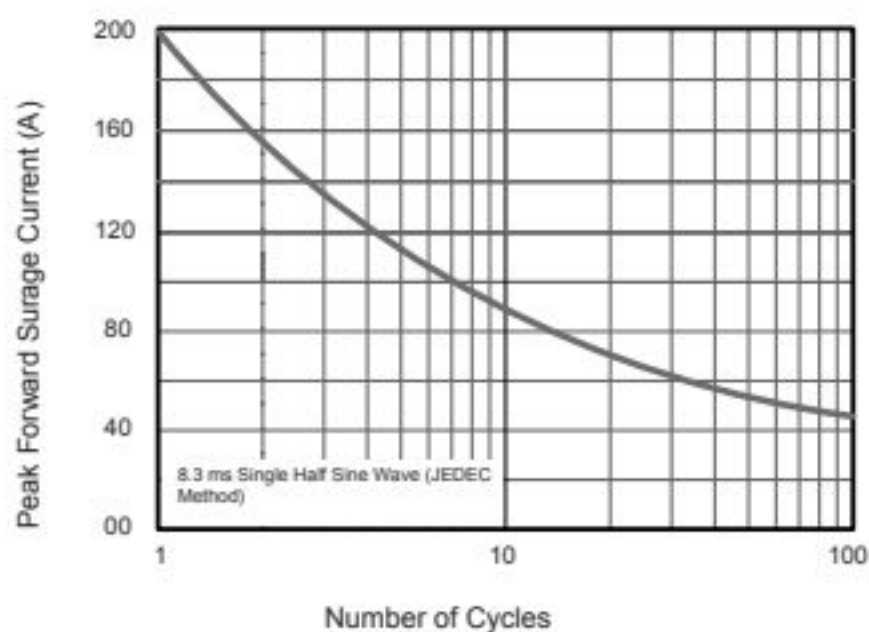
Fig.5 Maximum Non-Repetitive Peak Forward Surge Current
