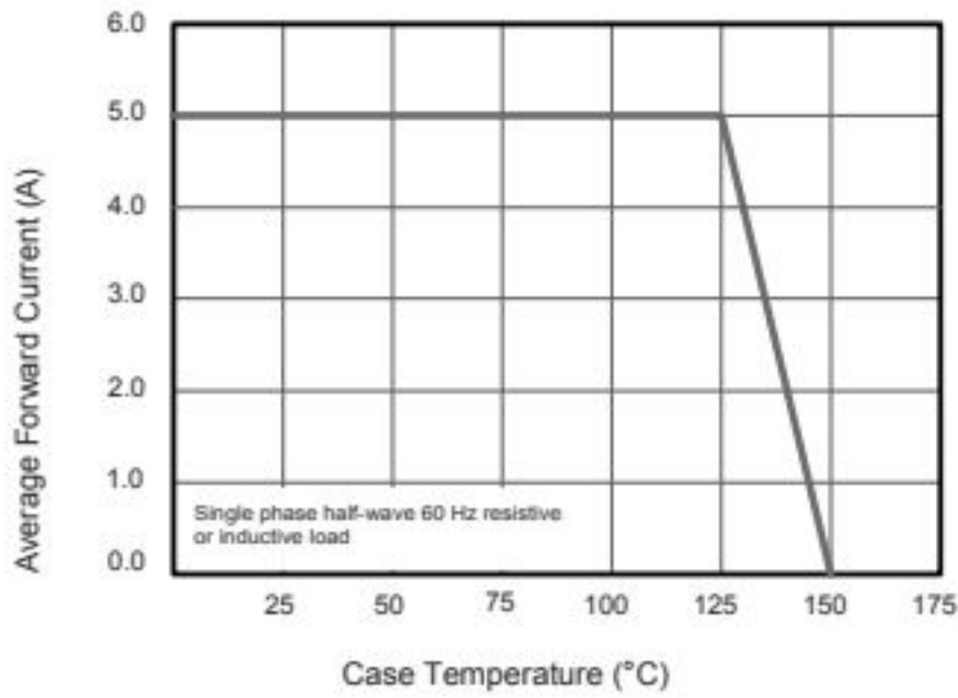
Fig.1 Forward Current Derating Curve
