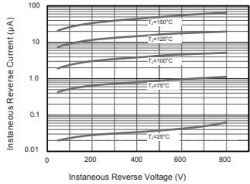
Fig.2 Typical Instantaneous Reverse Characteristics
