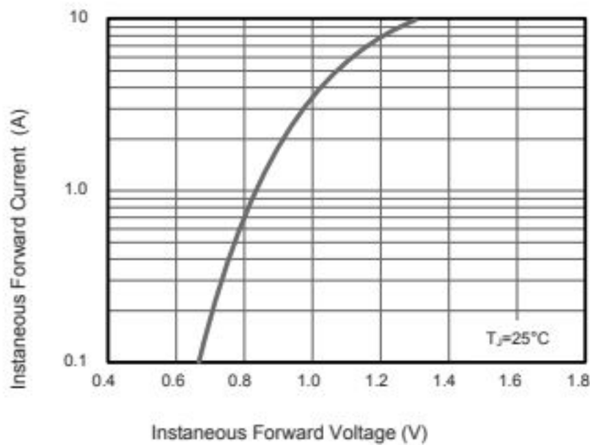
Fig.3 Typical Forward Characteristic
