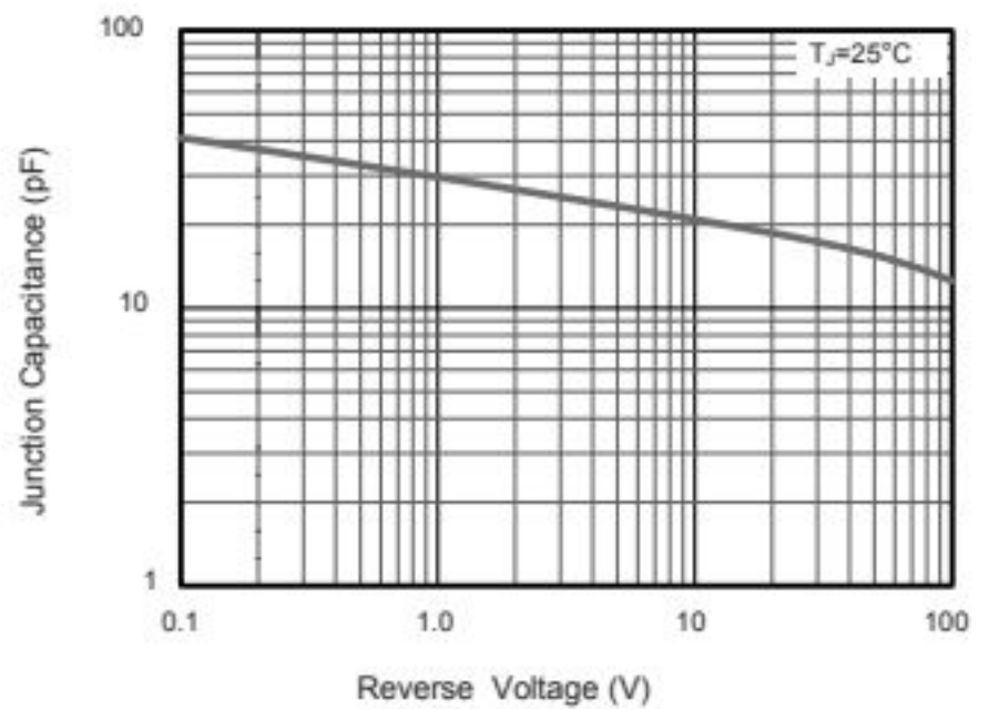
Fig.4 Typical Junction Capacitance
