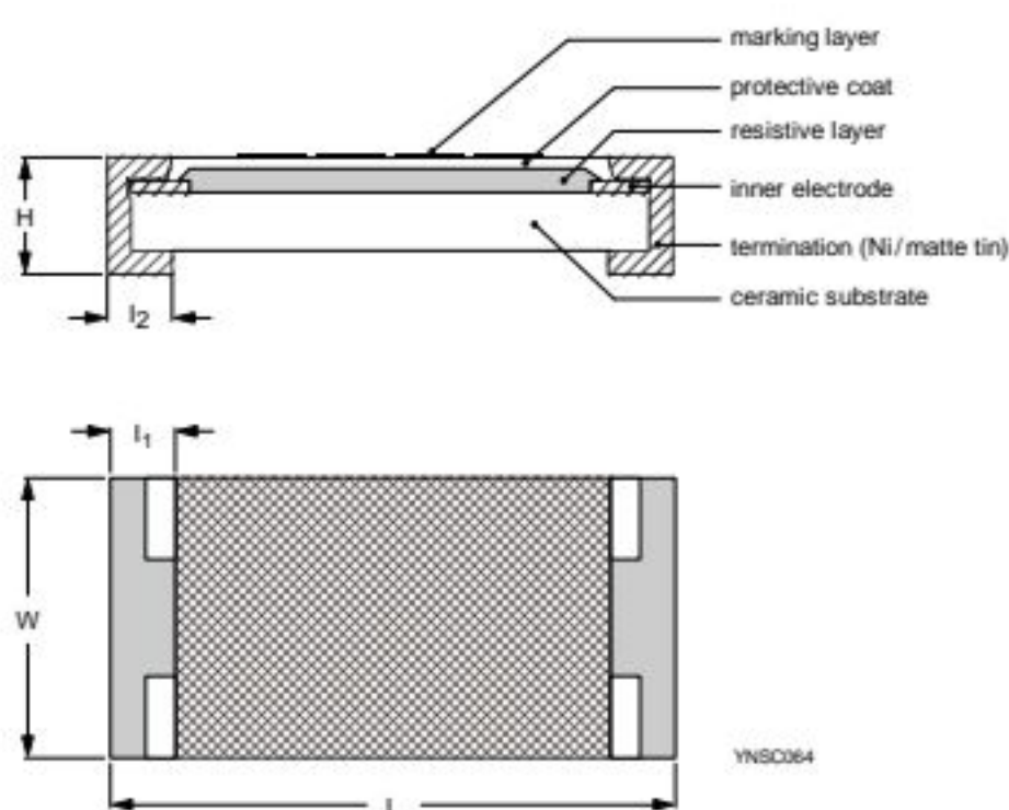
Fig. 5 Chip resistor outlines
