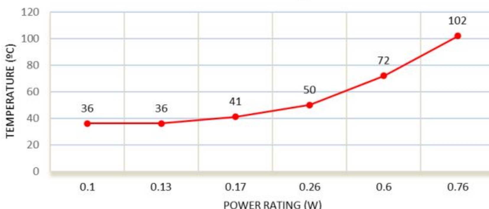
CSR1206 100mΩ Surface Temperature Rise
