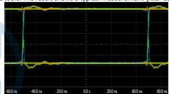
Figure 16. \pi 130Mxx/\pi 131Mxx Eye Diagram
