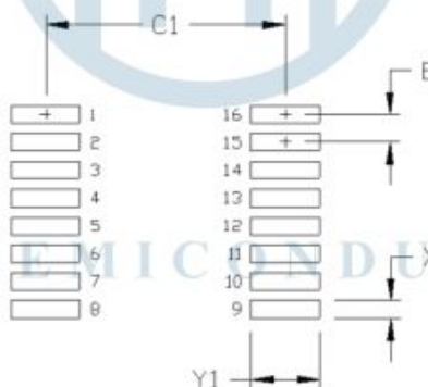
Figure 23. 16-Lead SSOP Land Pattern
