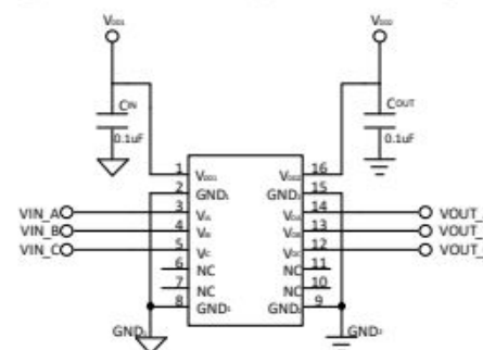
Figure 2. \pi 130x3x Typical Application Circuit
