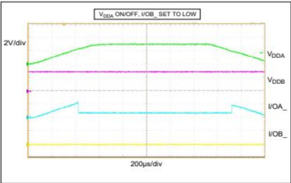
Figure 7. Undervoltage-Lockout Behavior (I/OA_ Set Low)
