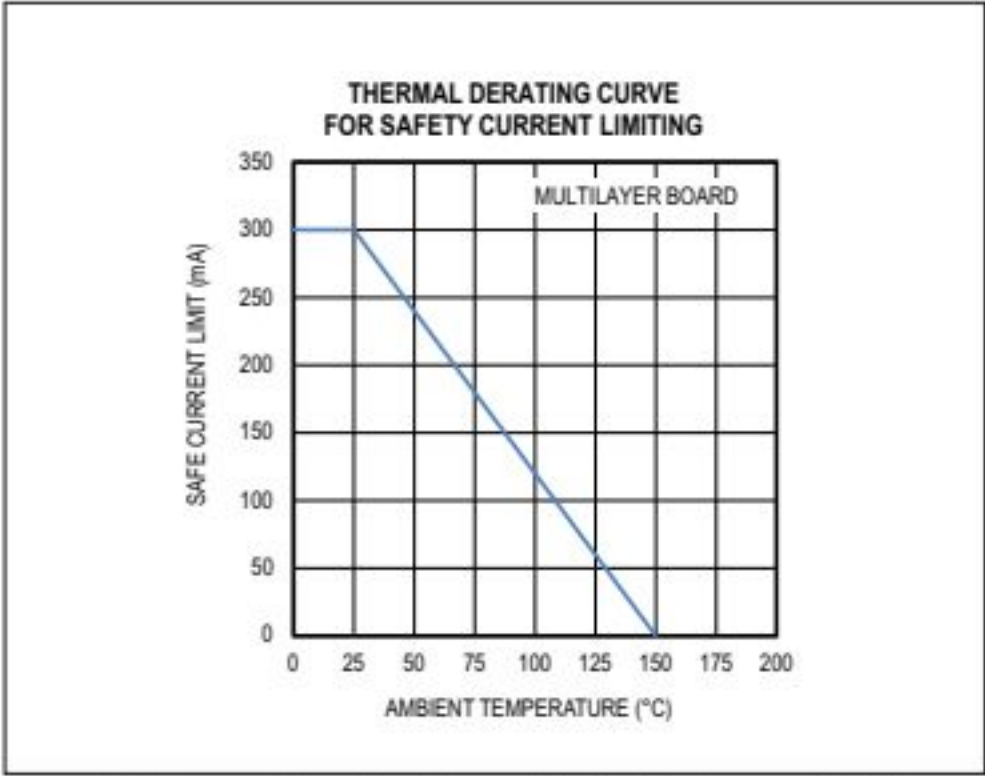
Figure 3. Thermal Derating Curve for Safety Current Limiting
