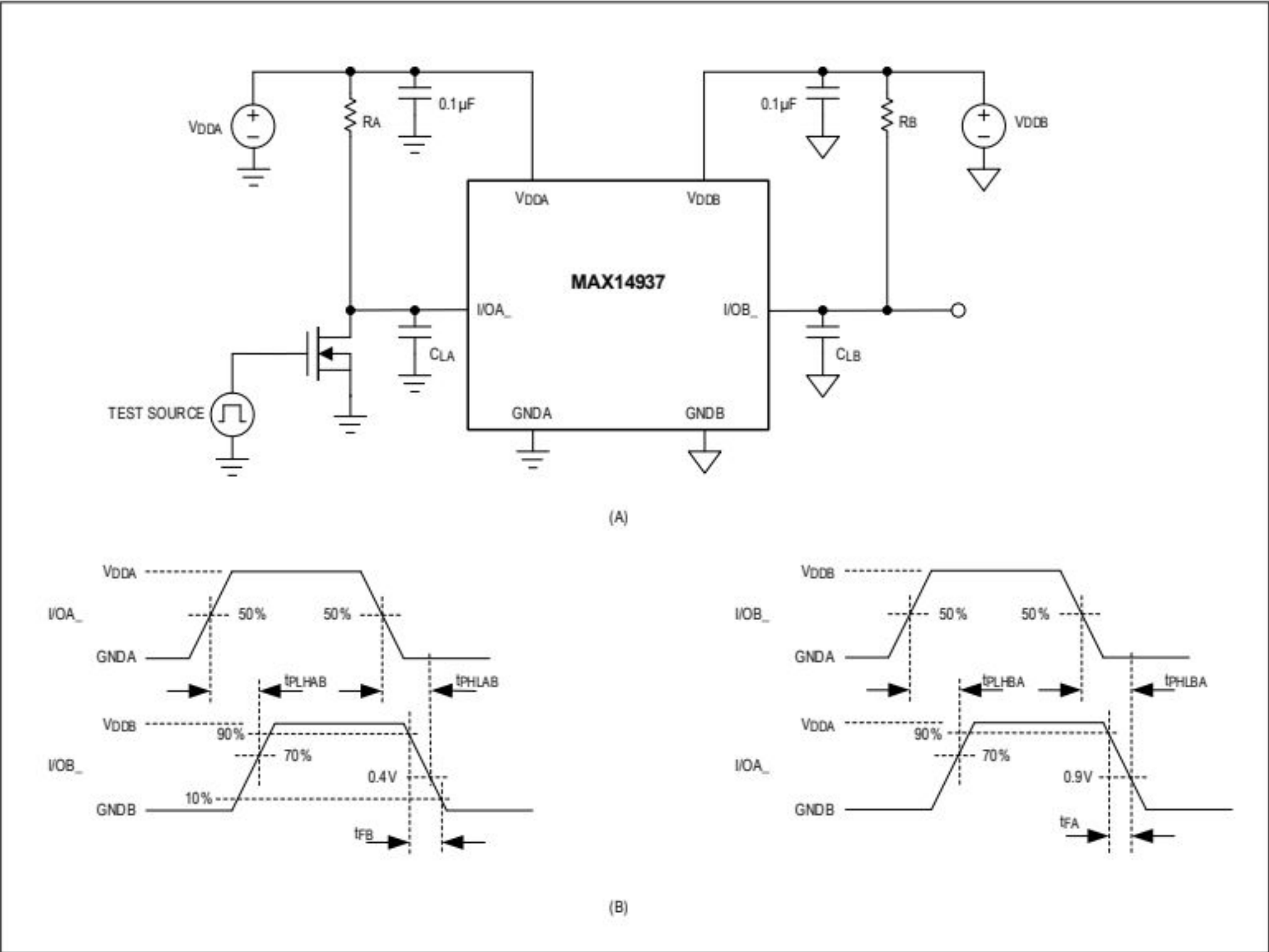
Figure 1. Test Circuit (A) and Timing Diagrams (B)
