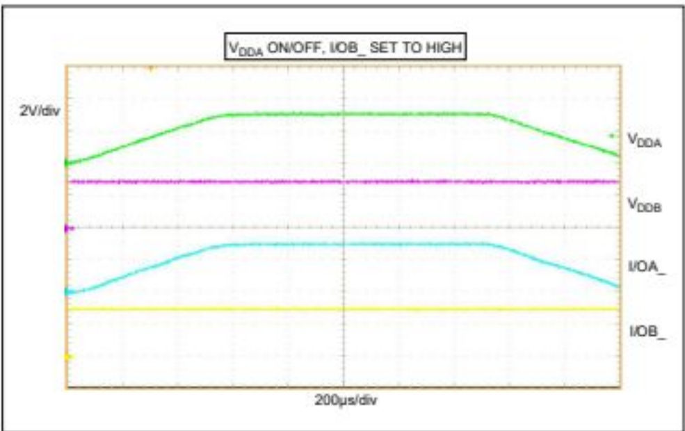
Figure 5. Undervoltage-Lockout Behavior (I/OA_ Set High)
