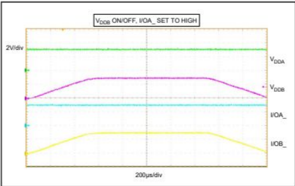
Figure 4. Undervoltage-Lockout Behavior (I/OB_ Set High)
