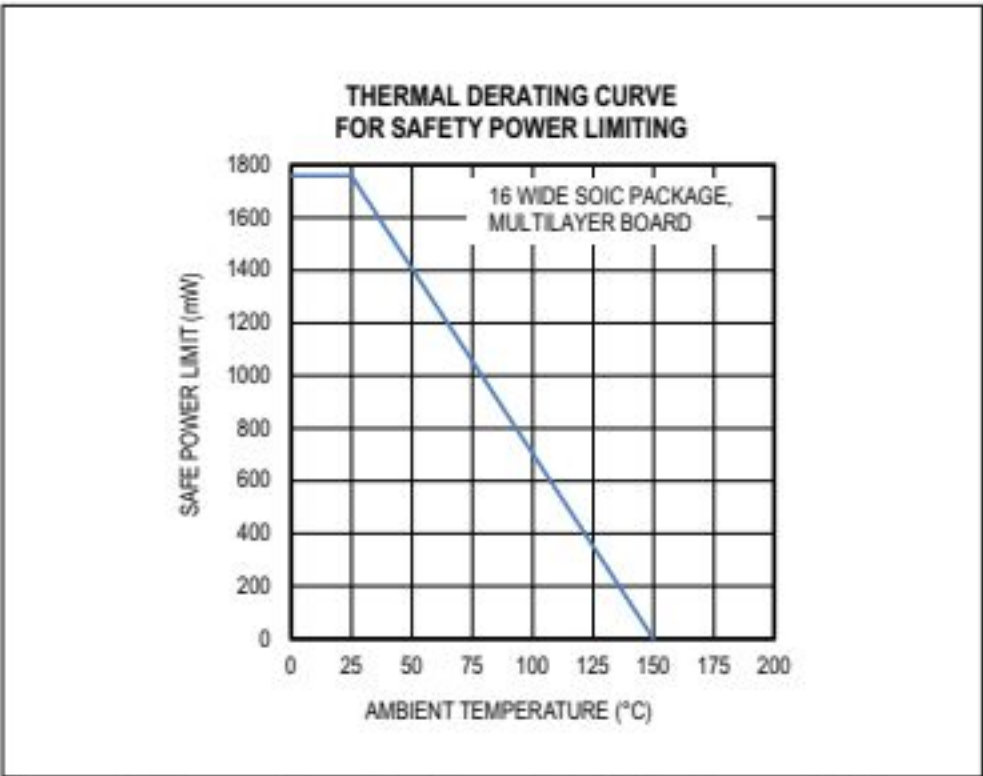
Figure 2. Thermal Derating Curve for Safety Power Limiting
