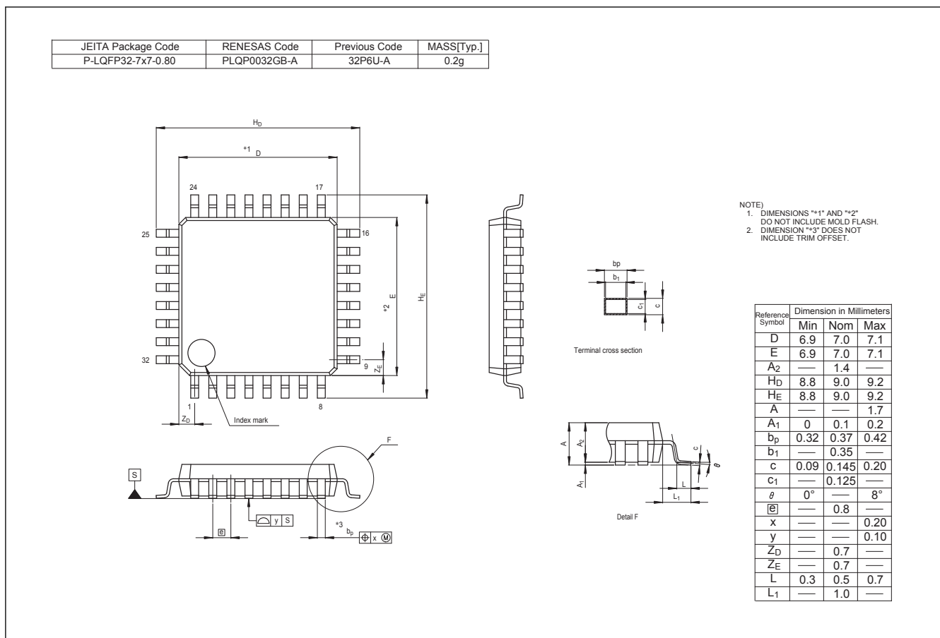
Figure 2.7 LQFP 32-pin (1)
