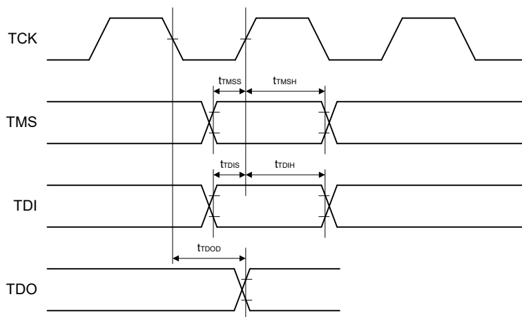
Figure 2.61 Boundary scan input/output timing
