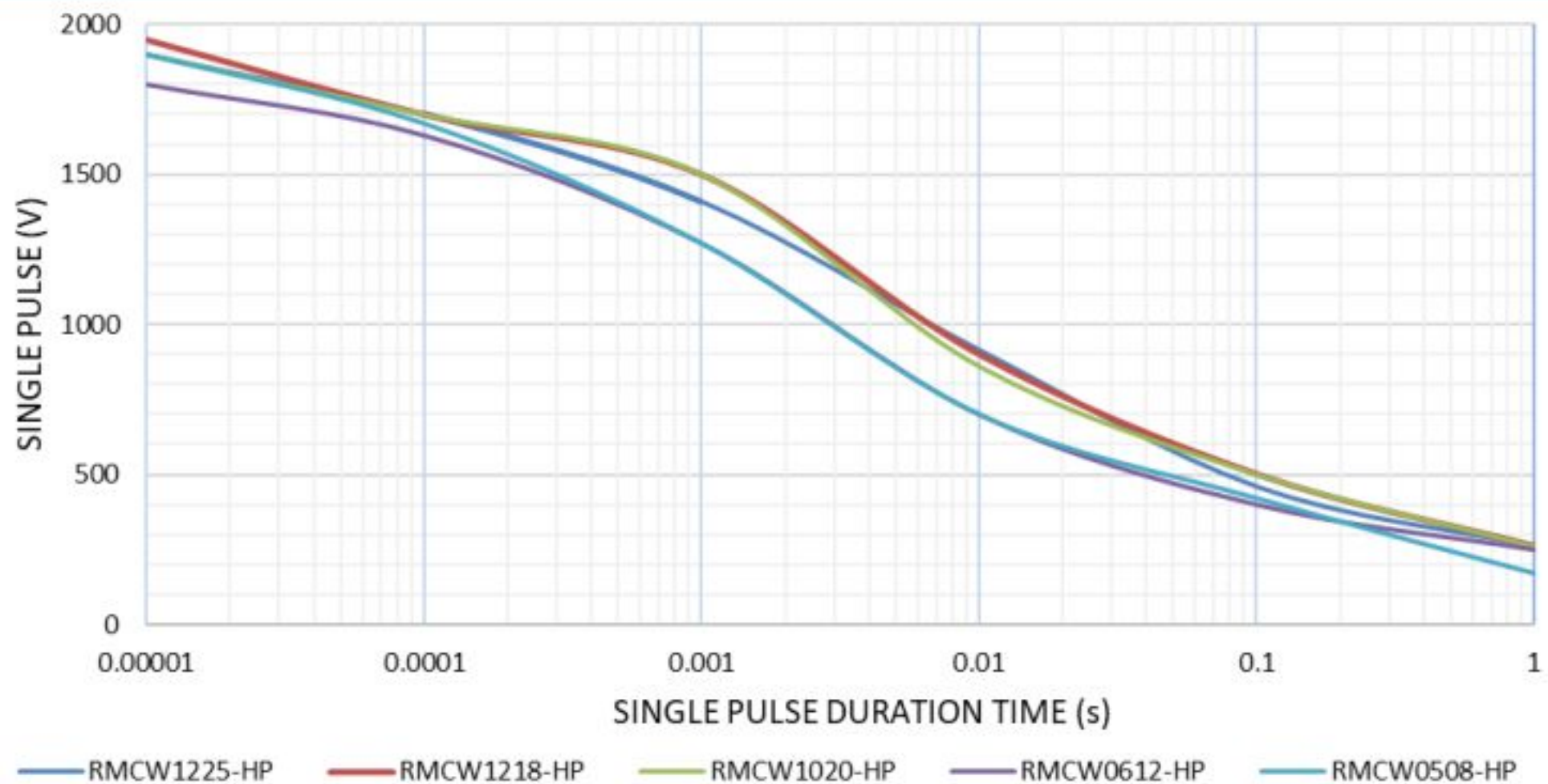
RMCW-HP Single Pulse – Voltage x Time
