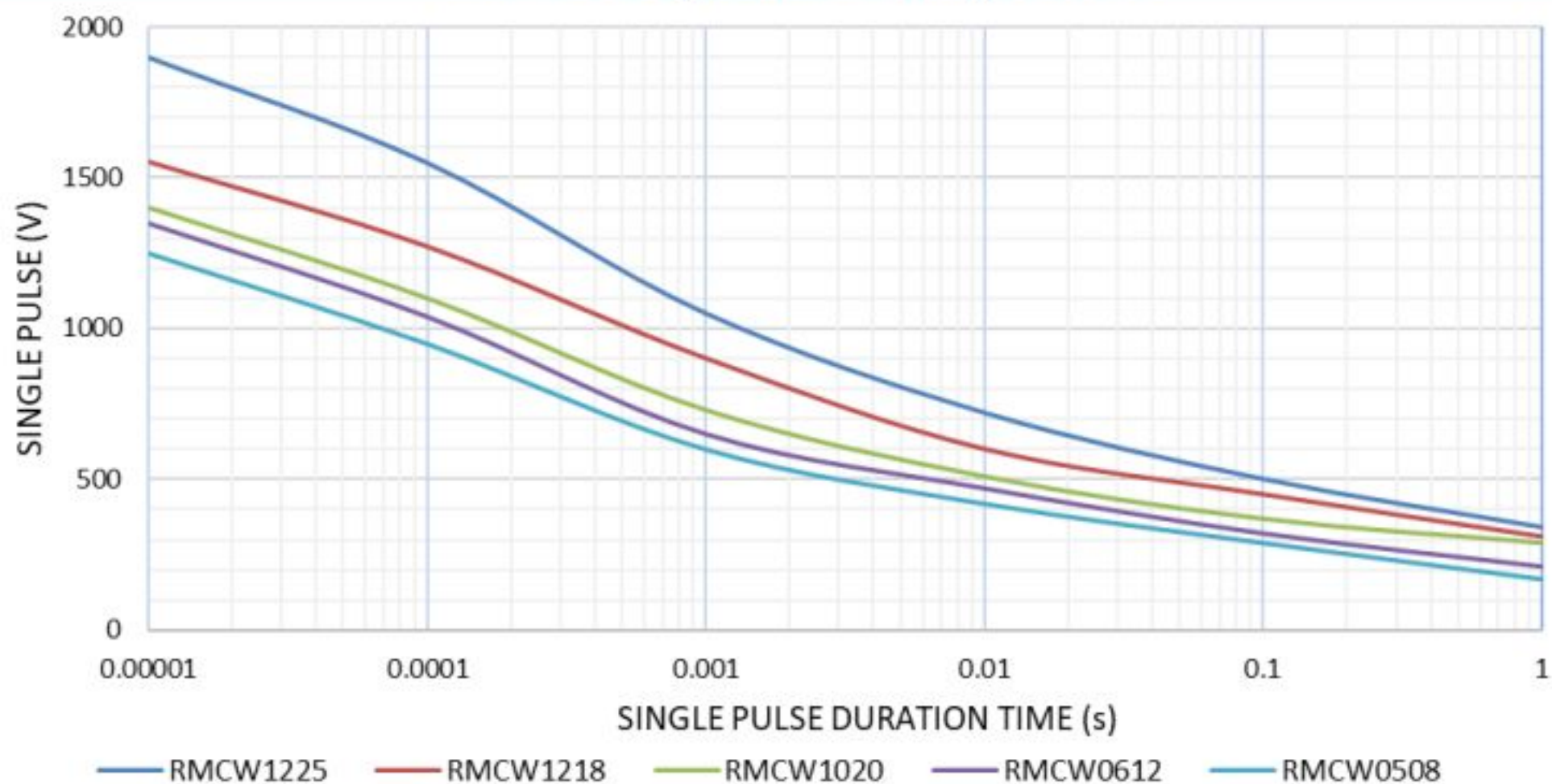
RMCW Single Pulse – Voltage x Time
