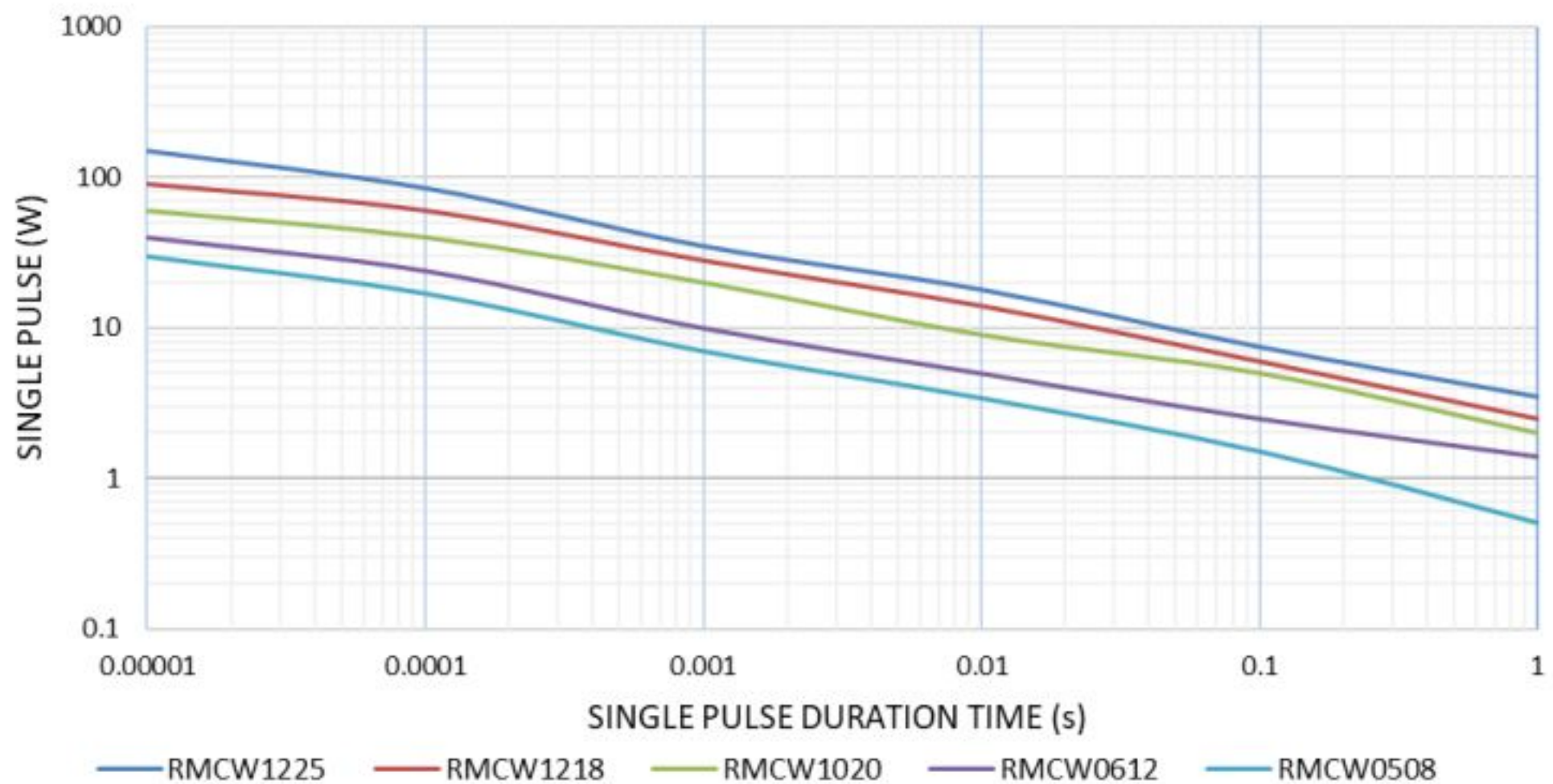
RMCW Single Pulse – Power x Time
