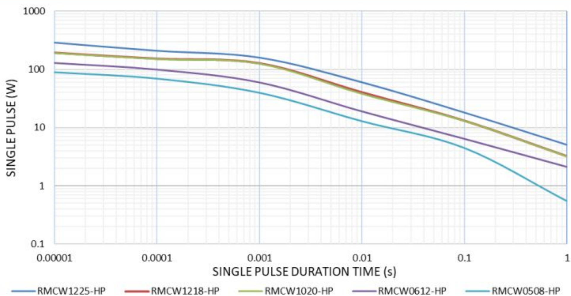
RMCW-HP Single Pulse – Power x Time
