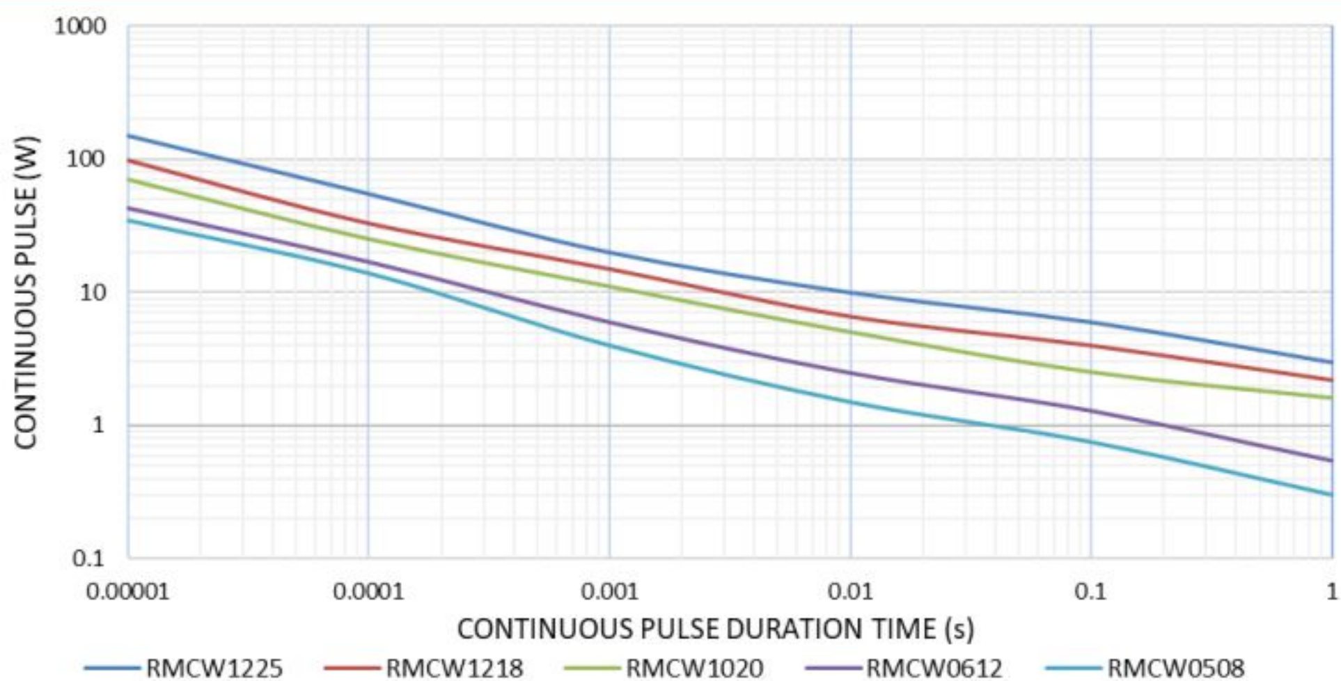
RMCW Continuous Pulse – Power x Time
