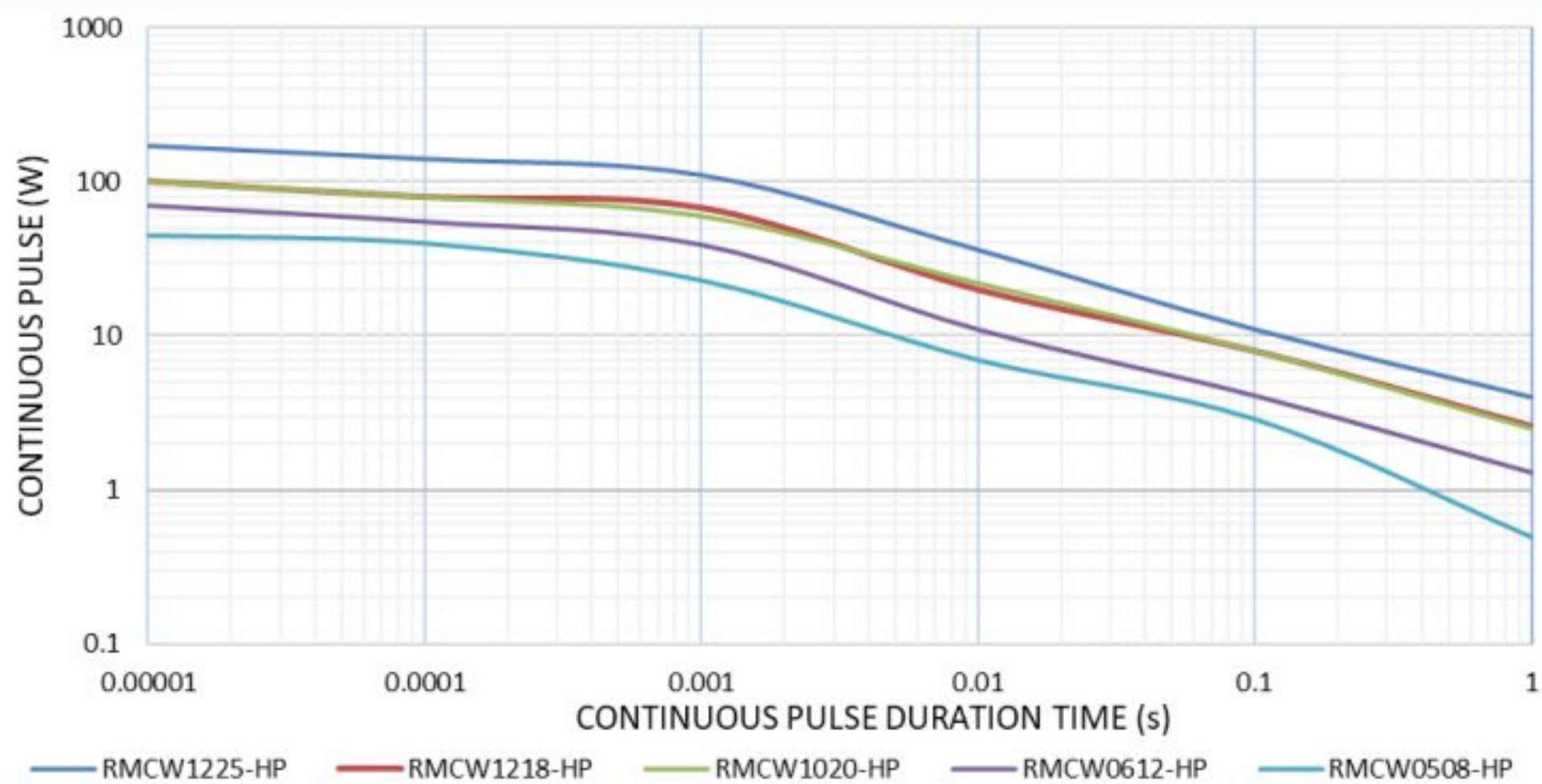
RMCW-HP Continuous Pulse – Power x Time
