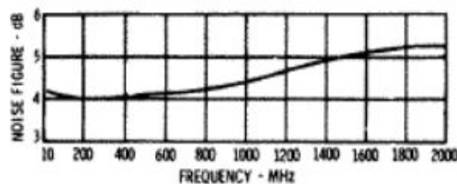
Noise Figure
