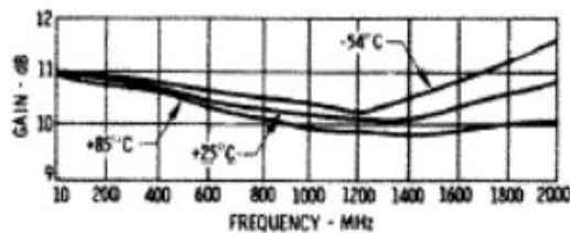
Gain
