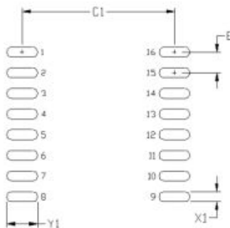
Figure 23. 16-Lead Wide Body SOIC [WB SOIC-16] Land Pattern
