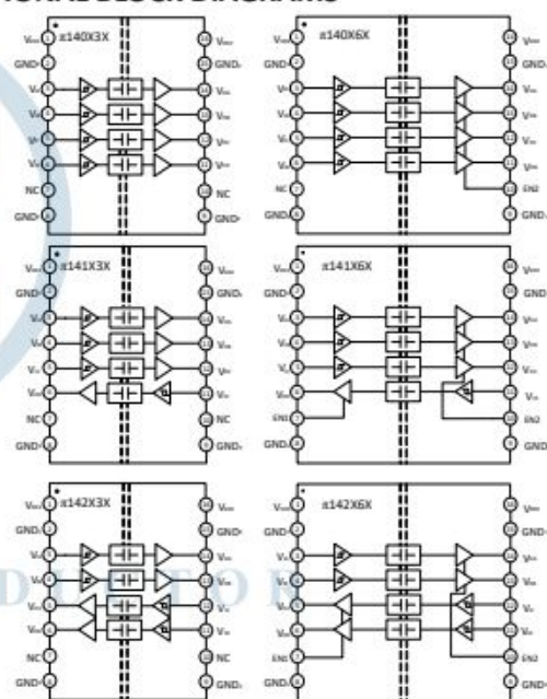
Figure 1. \pi 140xxx/\pi 141xxx/\pi 142xxx functional Block Diagram
