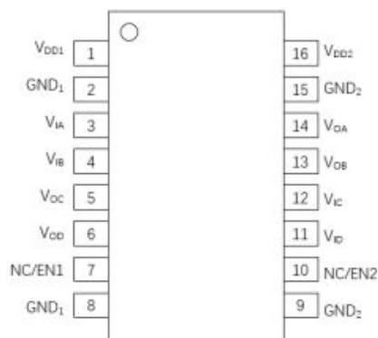
Figure 5. \pi 142Exx Pin Configuration
