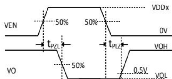
Figure 12. t_{PZL}/t_{PLZ} measurement waveform
