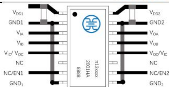
Figure 15. Recommended Printed Circuit Board Layout
