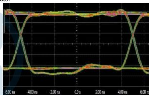
Figure 16. \pi 130Exx/\pi 131Exx Eye Diagram
