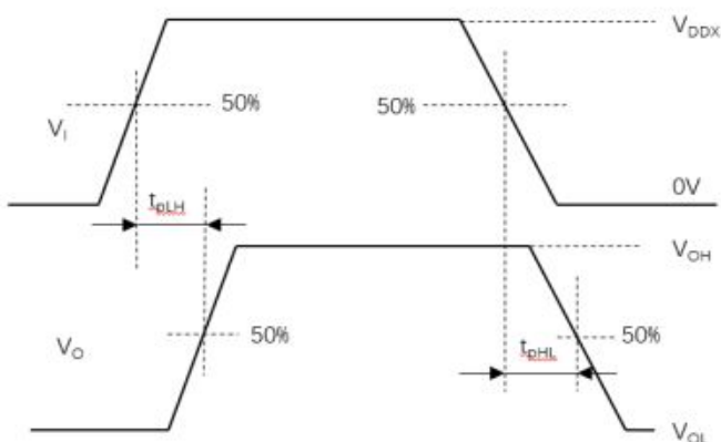
Figure 10. Propagation delay time waveform measurement
