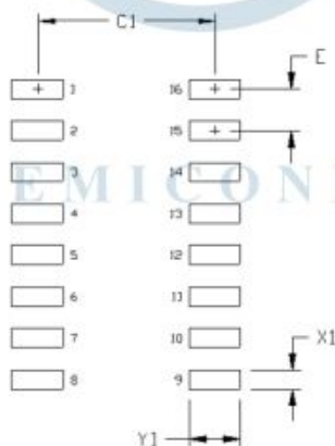
Figure 21.16-Lead Narrow Body SOIC [NB SOIC-16] Land Pattern
