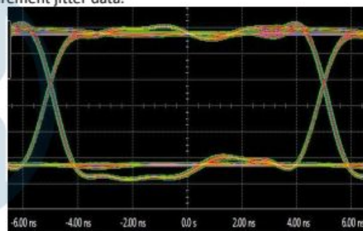
Figure 16. \pi 120Exx/\pi 121Exx/\pi 122Exx Eye Diagram
