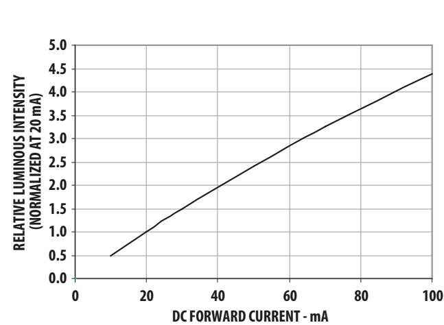
Figure 5: Relative Luminous Intensity vs. Forward Current
