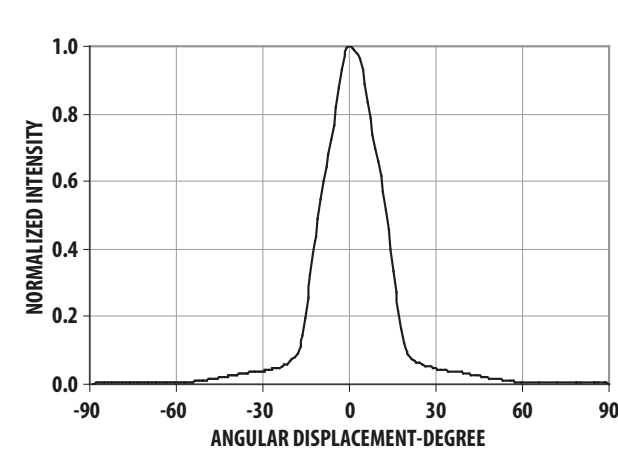
Figure 8: Radiation Pattern for 23° Viewing Angle Lamp
