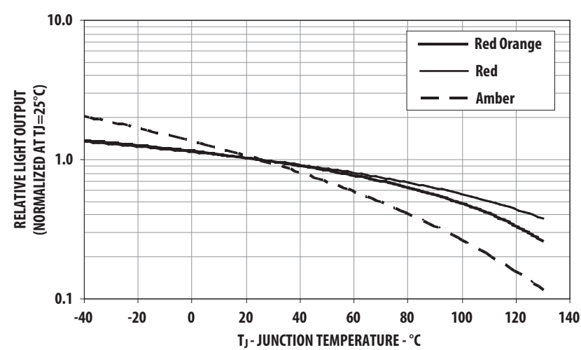
Figure 10: Relative Light Output vs. Junction Temperature
