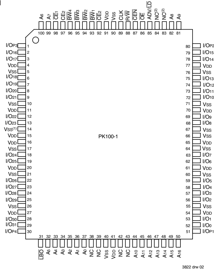
Top View TQFP
