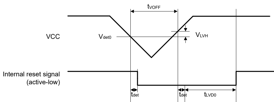
Figure 2.43 Voltage detection circuit timing ( V_{\text{det0}} )
