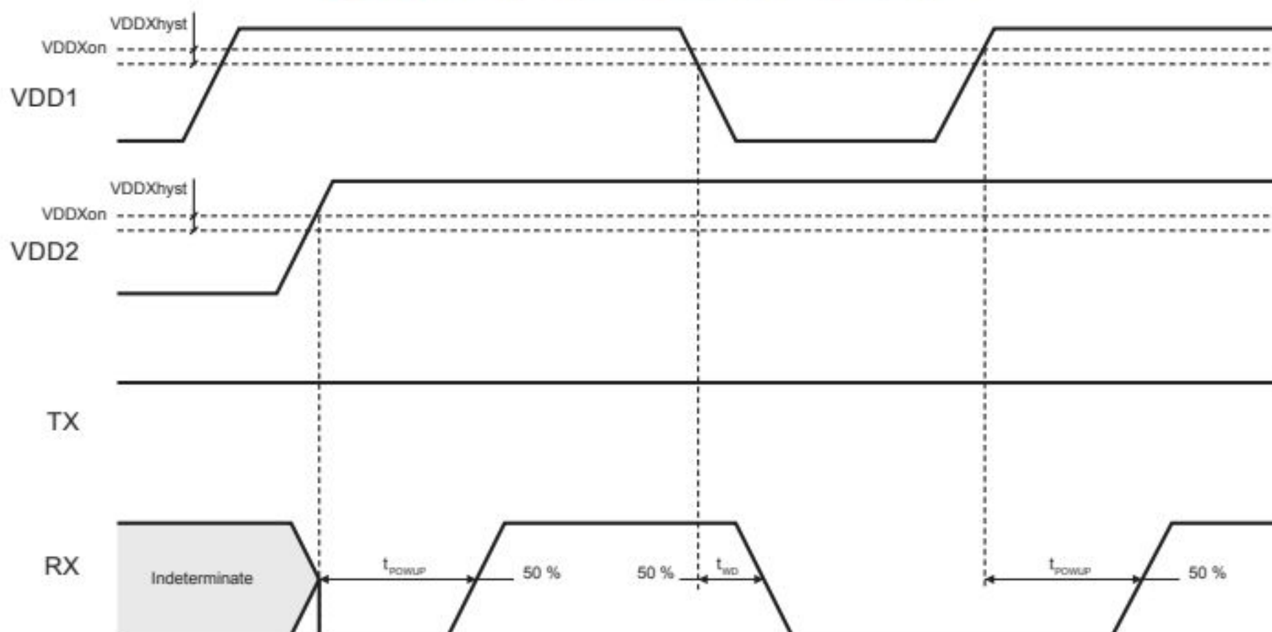
Figure 4. Timing diagram – power-up and power-down
