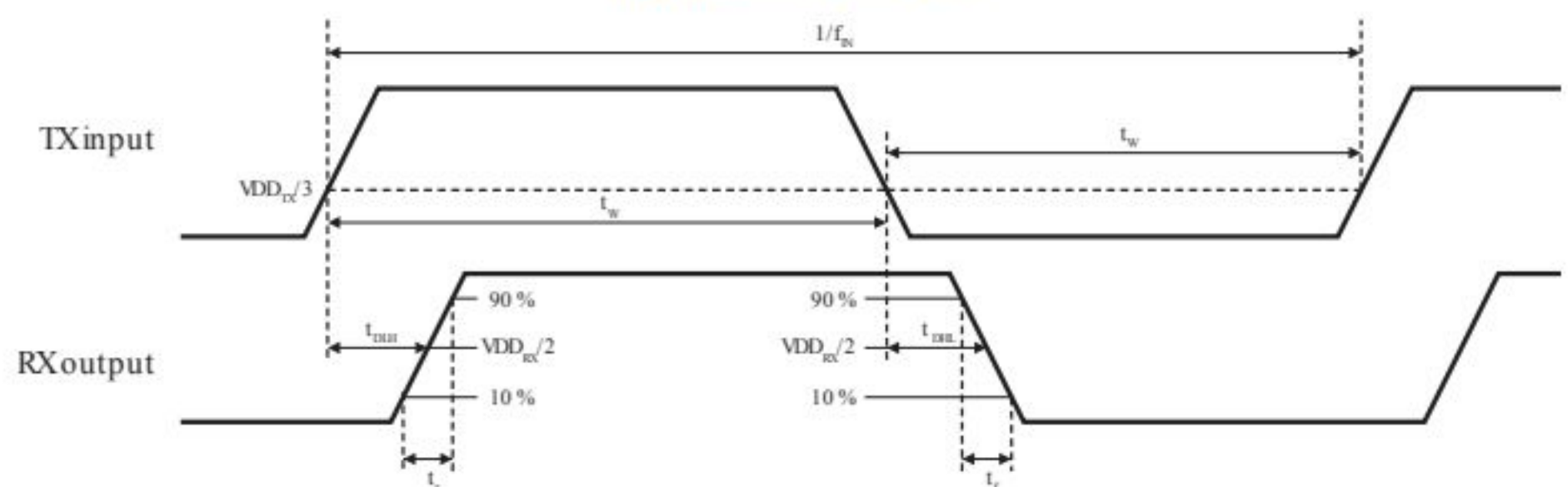
Figure 3. Timing diagram
