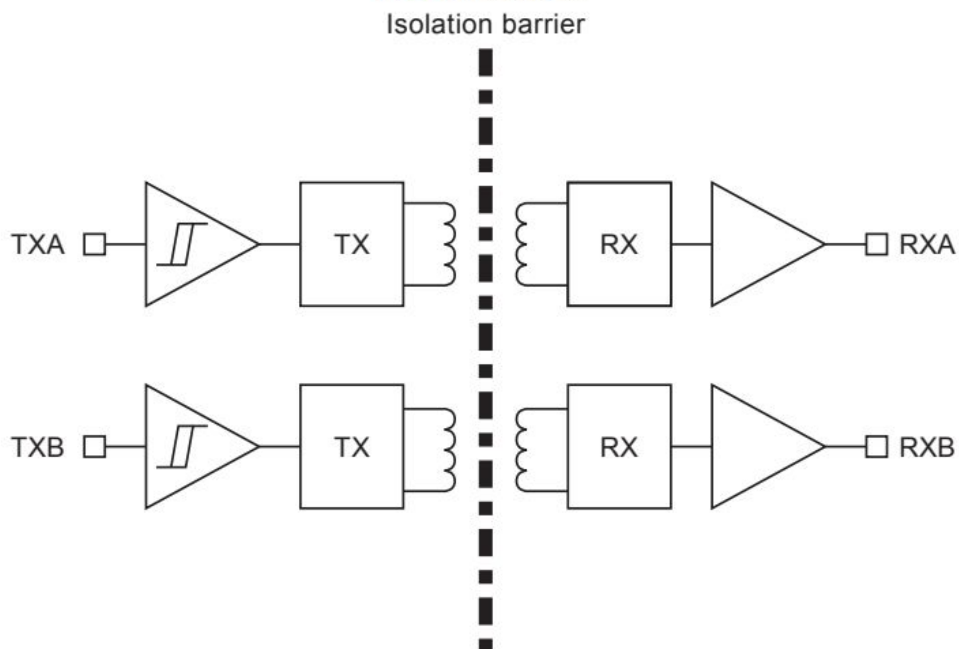
Figure 1. Block diagram
