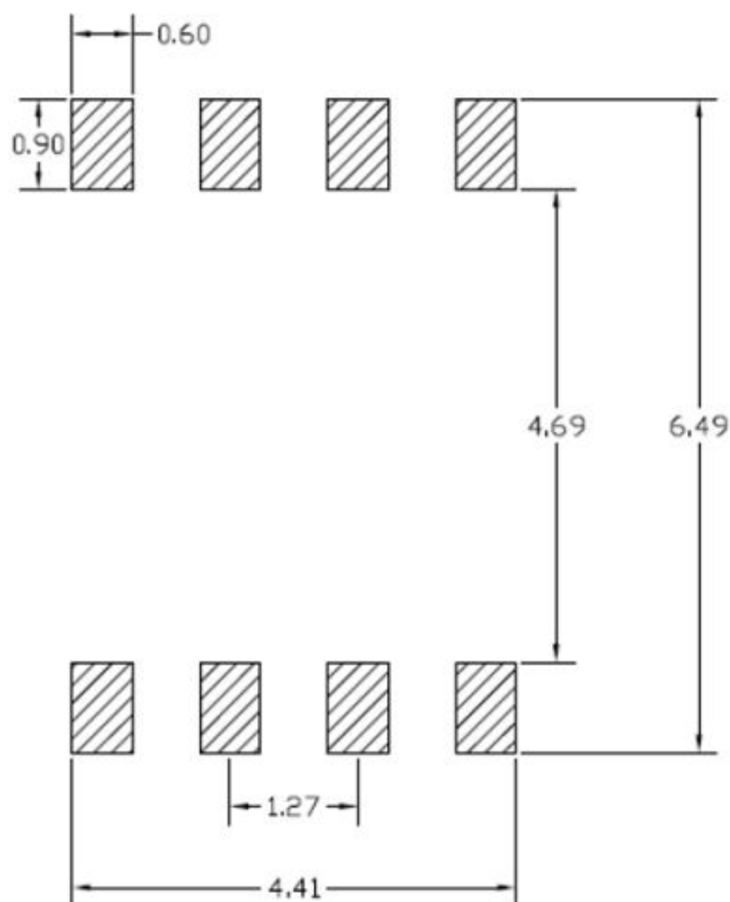
Figure 8. SO8 package recommended footprint
