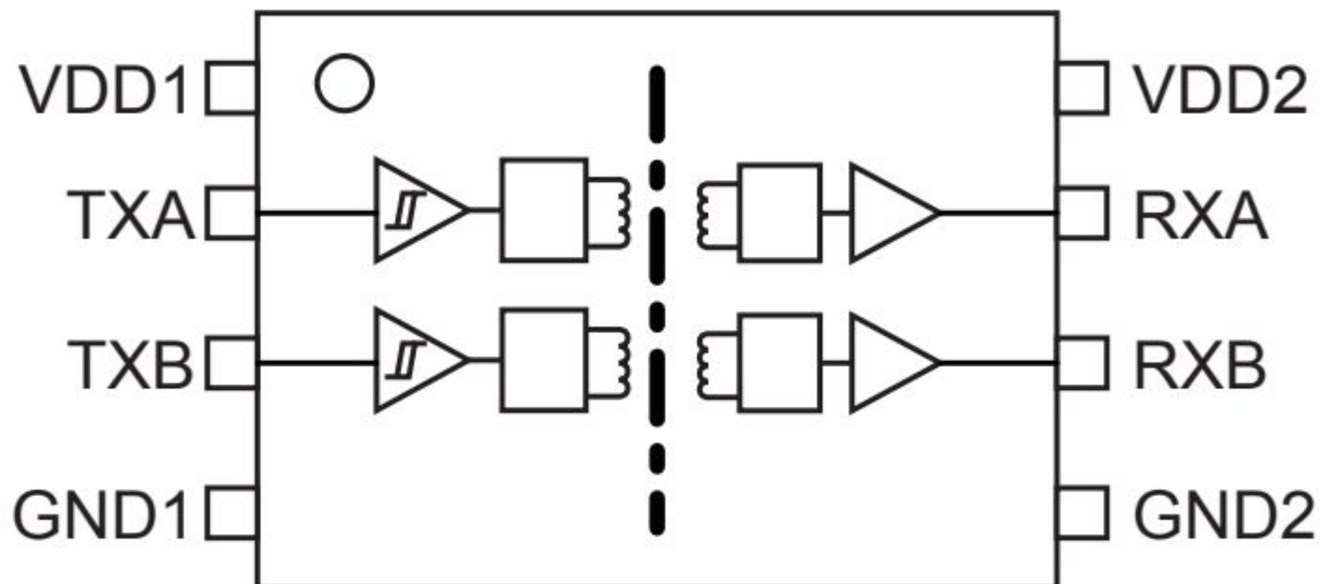
Figure 2. Pin connection (top view)
