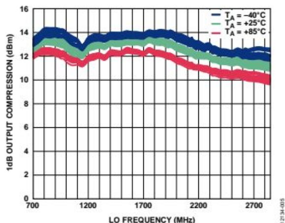
Figure 5. SSB 1 dB Output Compression Point (OP1dB) vs. LO Frequency ( f_{\text{LO}} ) and Temperature; Multiple Devices Shown
