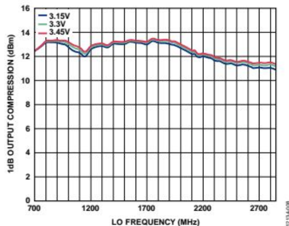
Figure 8. SSB 1 dB Output Compression Point (OP1dB) vs. LO Frequency ( f_{\text{LO}} ) and Supply
