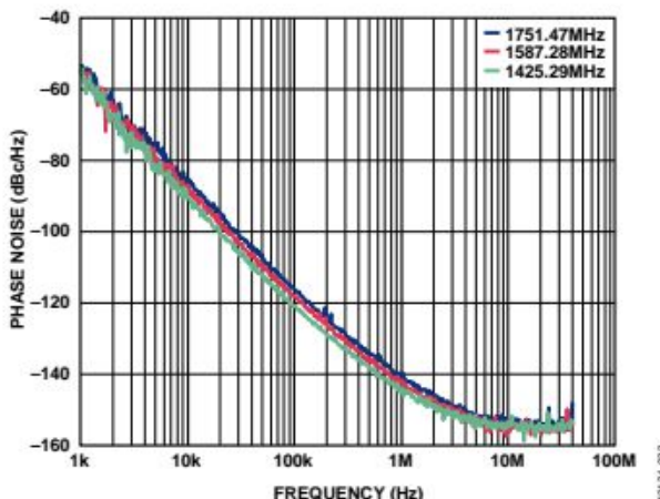
Figure 33. Open-Loop VCO Phase Noise for VCO 3 Measured at 1425.29 MHz, 1587.28 MHz, and 1751.47 MHz ( VCO \div 2 )
