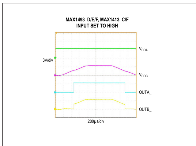
Figure 8. Undervoltage Lockout Behavior (MAX1493_ D/E/F, MAX1413_C/F High)
