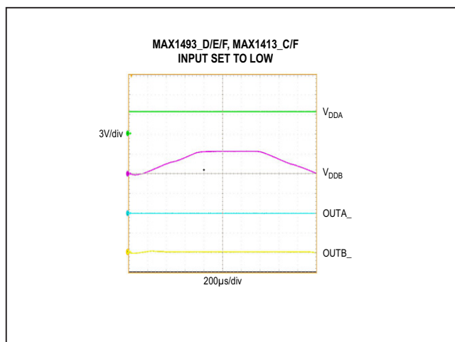
Figure 9. Undervoltage Lockout Behavior (MAX1493_ D/E/F, MAX1413_C/F Low)
