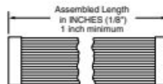
Assembled Length (-"XX.XX")
