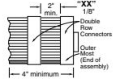
Daisy Chain (-D “XX”)
