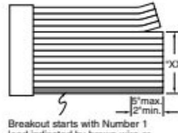
Breakout (-B “XX”)
