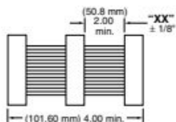
Daisy Chain (-D "XX")
