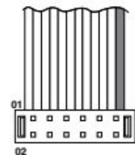
Reverse Wiring (-RW)
